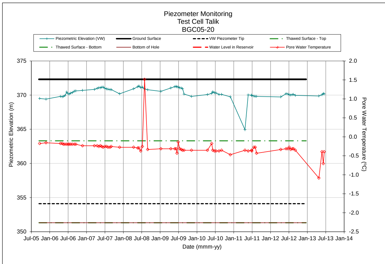
Figure 7. Pore Pressures in Test Cell Talik.
