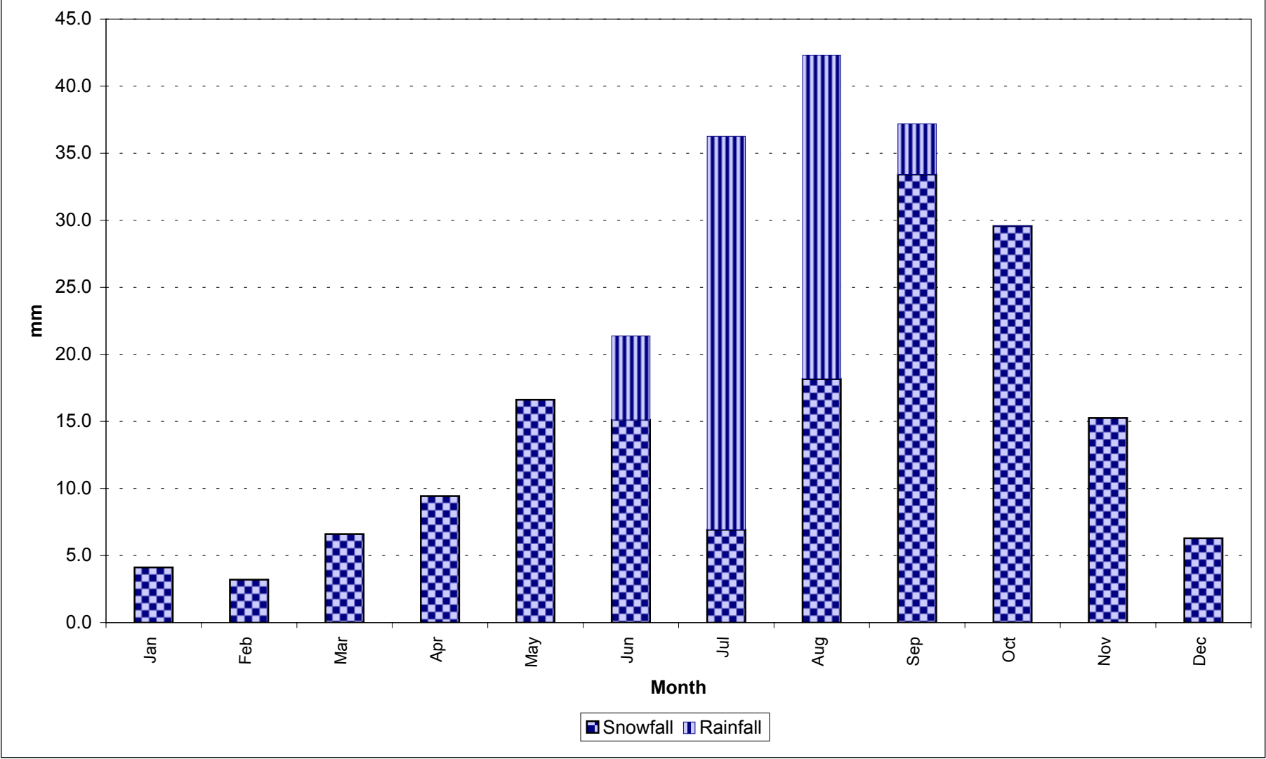
Figure 3-5: Average Monthly Precipitation (1977-2001)
