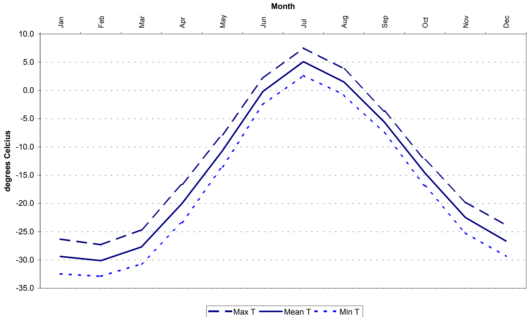
Figure 3-4: Average Monthly Temperatures (1977-2001)
