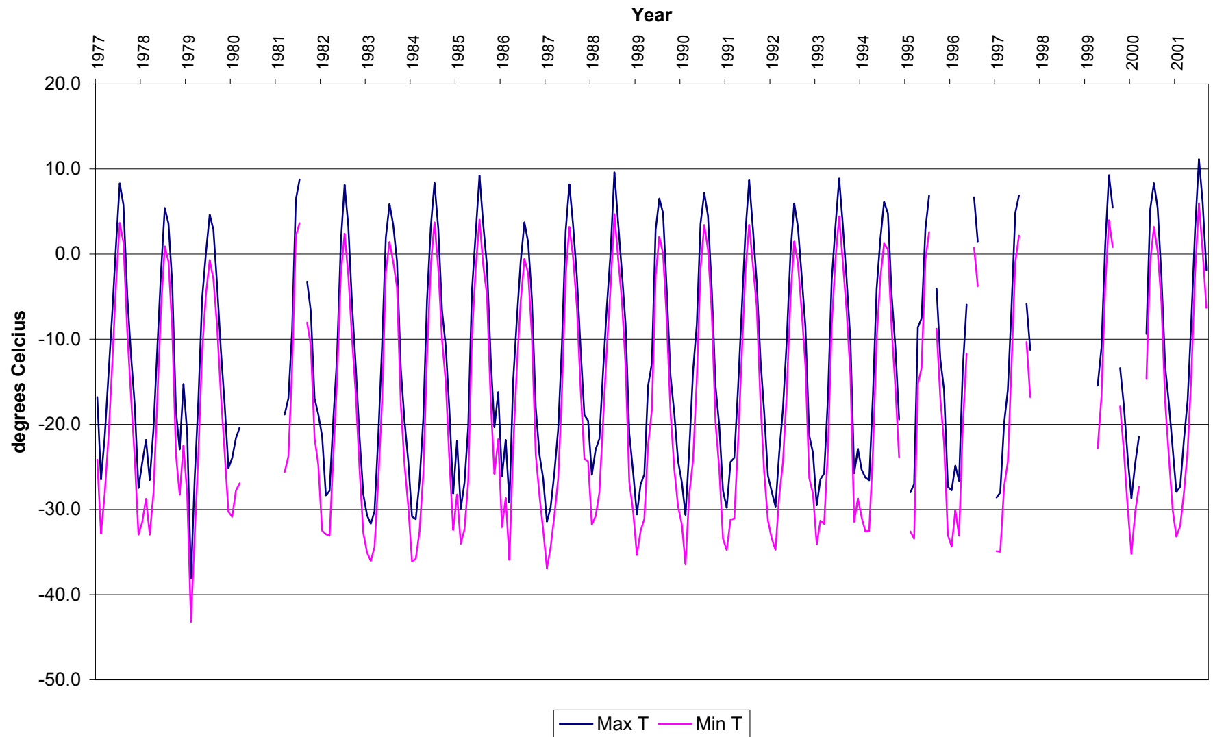
Figure 3-2: Monthly Average Temperatures
