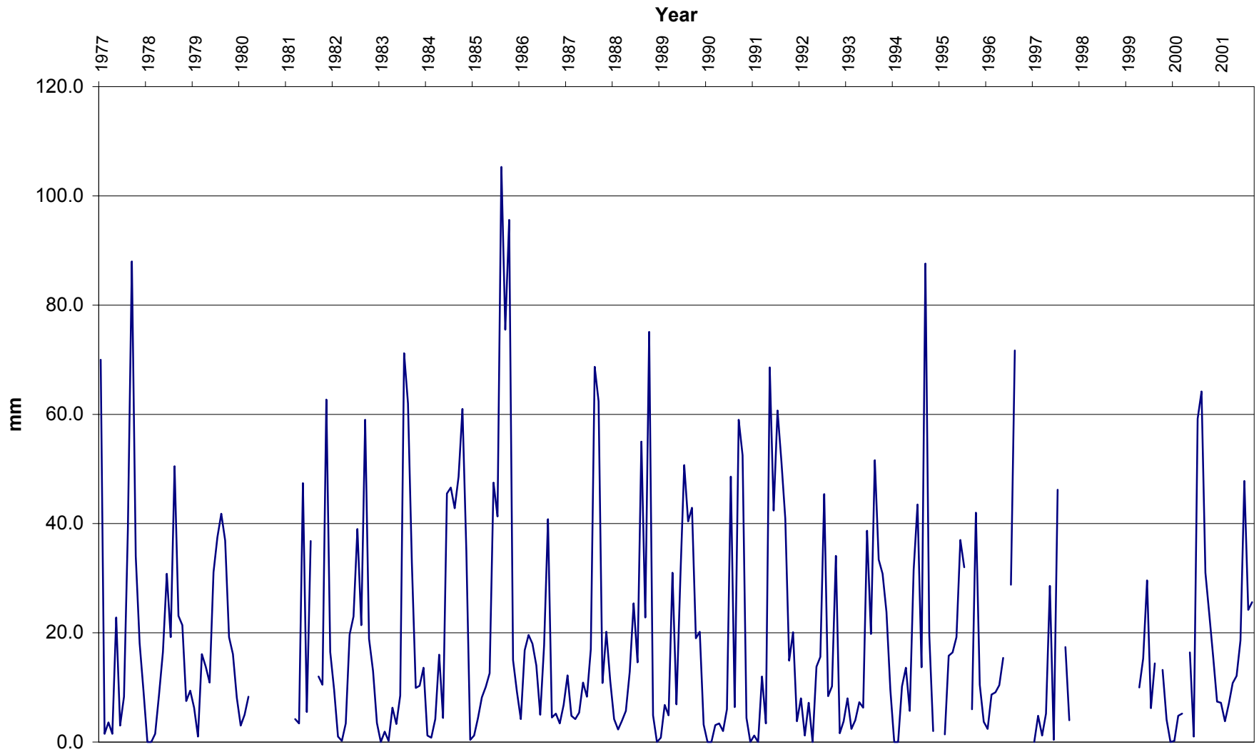
Figure 3-3: Monthly Total Precipitation
