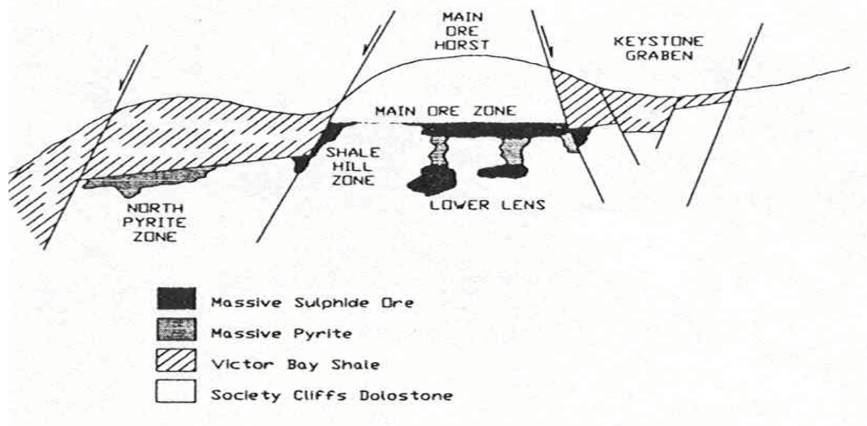
Figure 2: Schematic Nanisivik Mine geology, looking east [Lecuyer, 2001].
