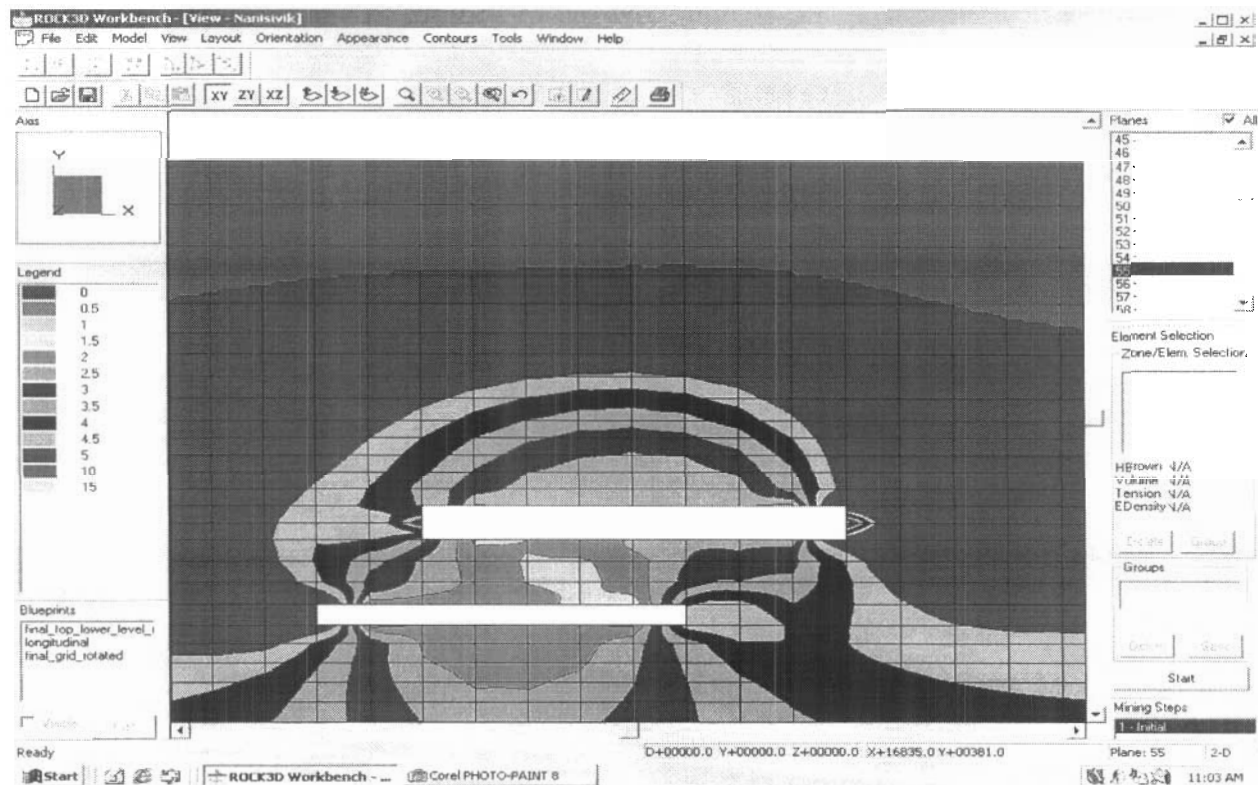
Figure 10: ROCK3D modeling results, Hoek and Brown failure criterion safety factors, section 55 looking east.
