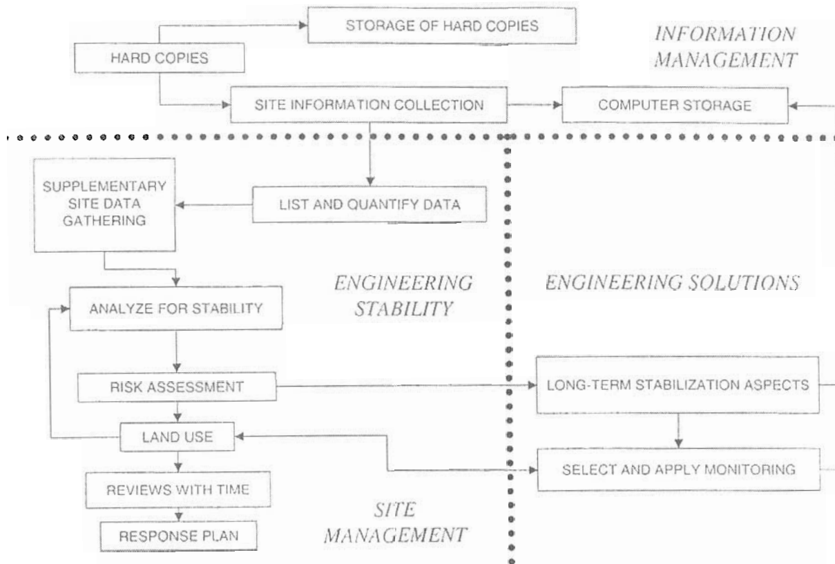
Figure 1: Shallow stope decommissioning flow chart [Bétournay, 2001].
