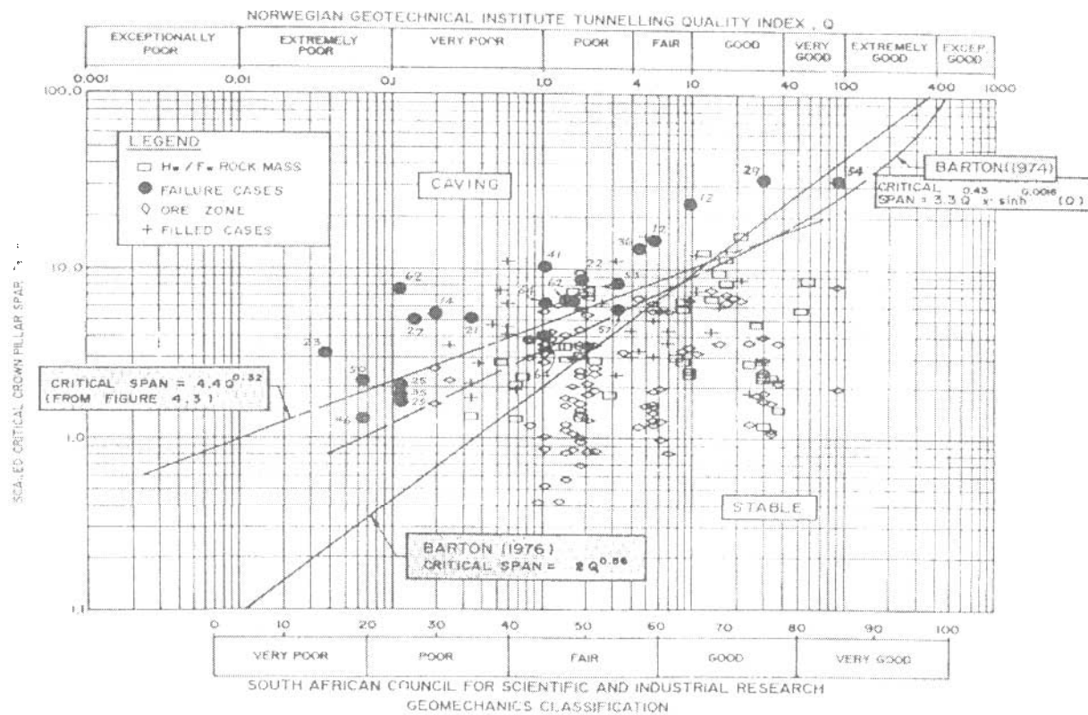
Figure 5: Critical empirical span for shallow slope surface crown pillars [CANMET Contract, 1990].
