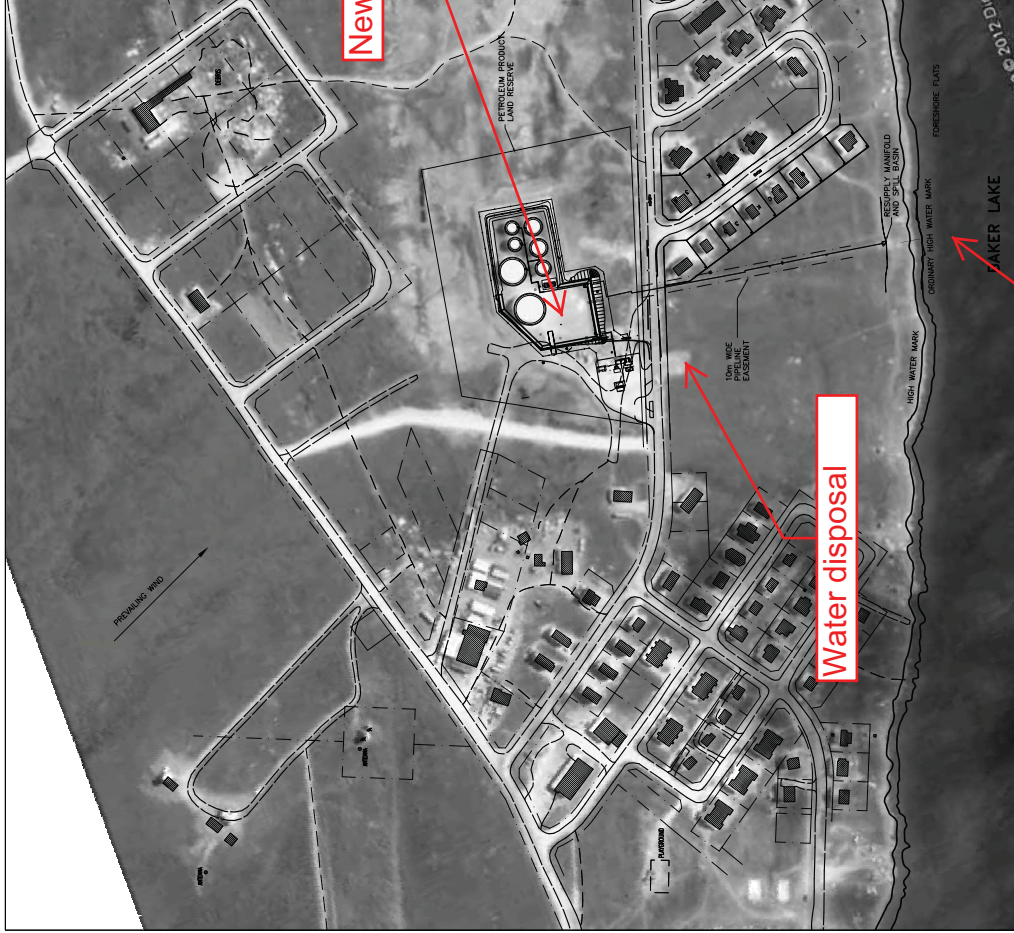
EXISTING TANK FARM SCALE: 1:2500 (APPROX.)
