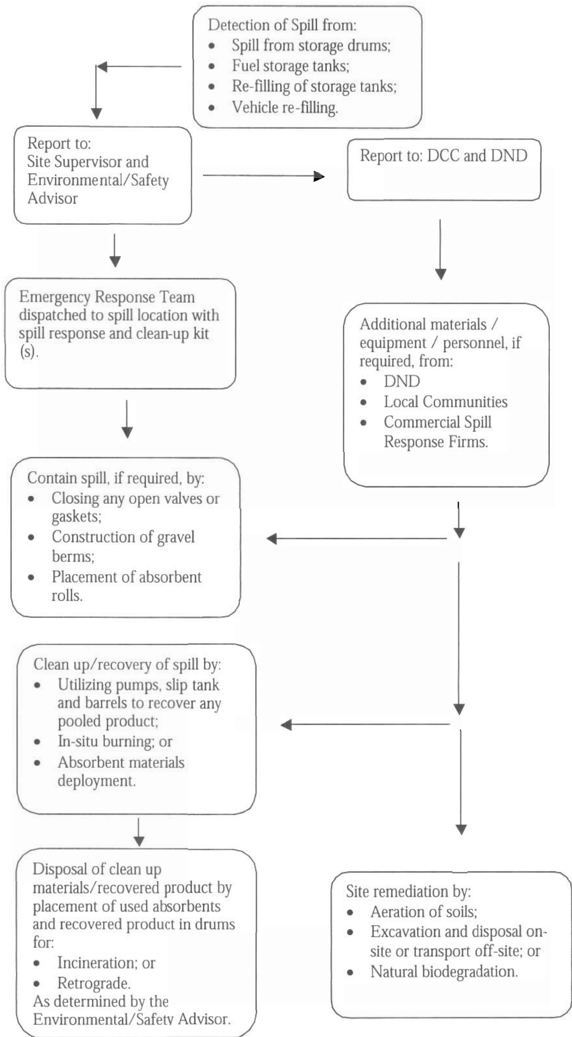
Figure 3: Procedures for Land Spill Response
