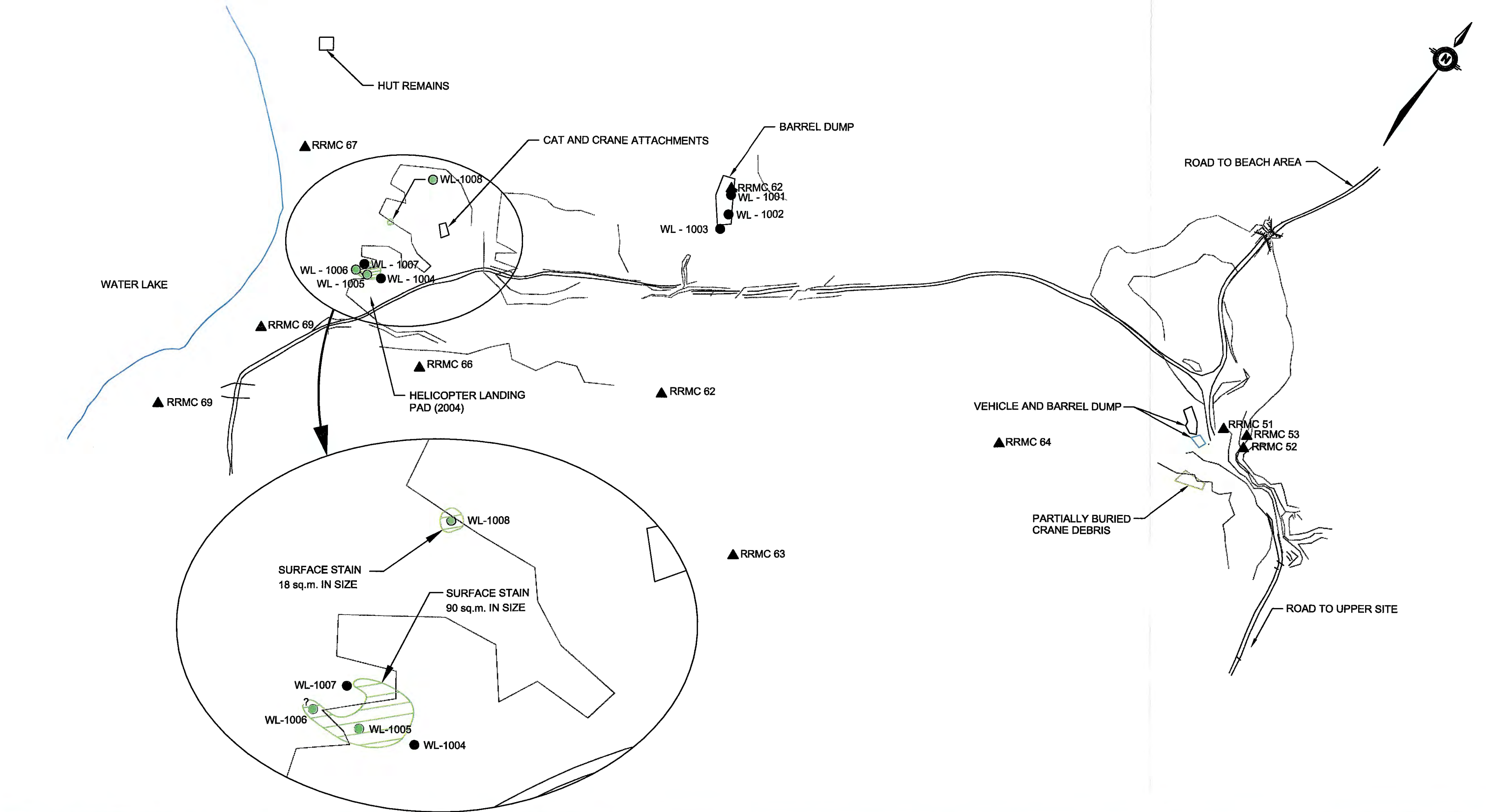
PWGSC FOX-C DEW LINE SITE - WATER LAKE BOREHOLE LOCATION PLAN Figure 4.0
