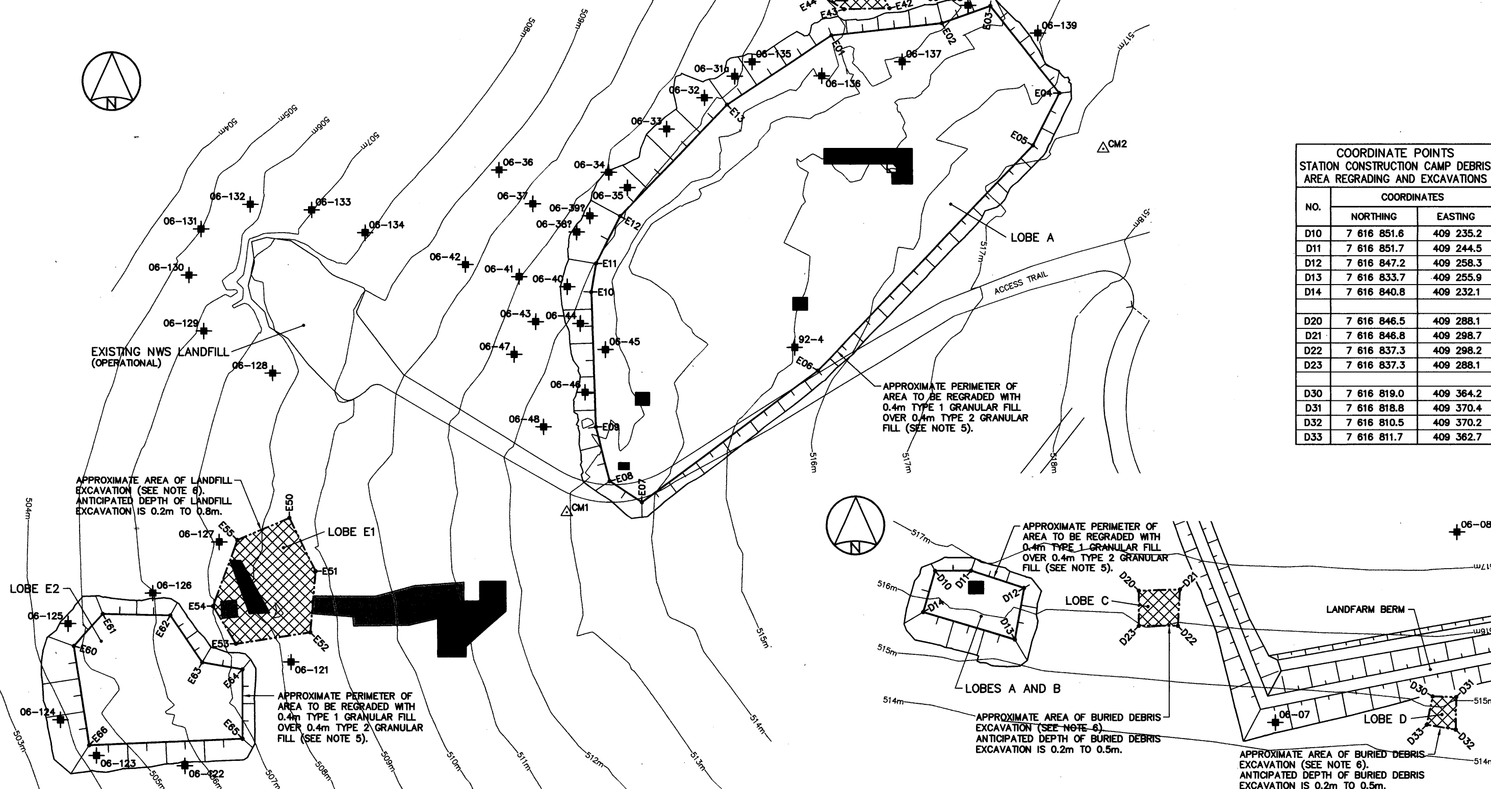
STATION WEST LANDFILL (LOBES A-E) (DWG. 105)
