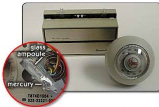
Figure 8 - Home Thermostat
