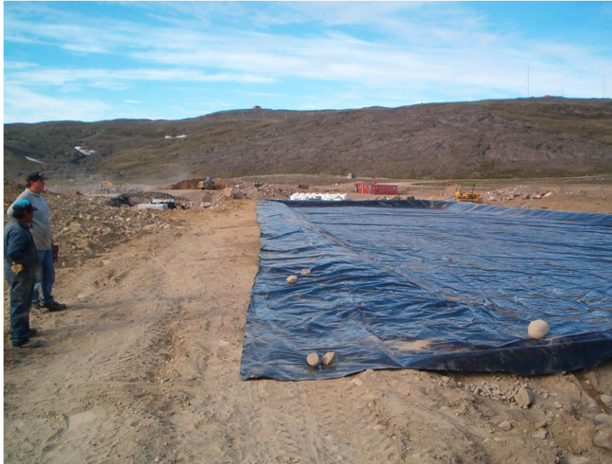
Photograph 3: 30 mil HDPE geomembrane over contour berms
