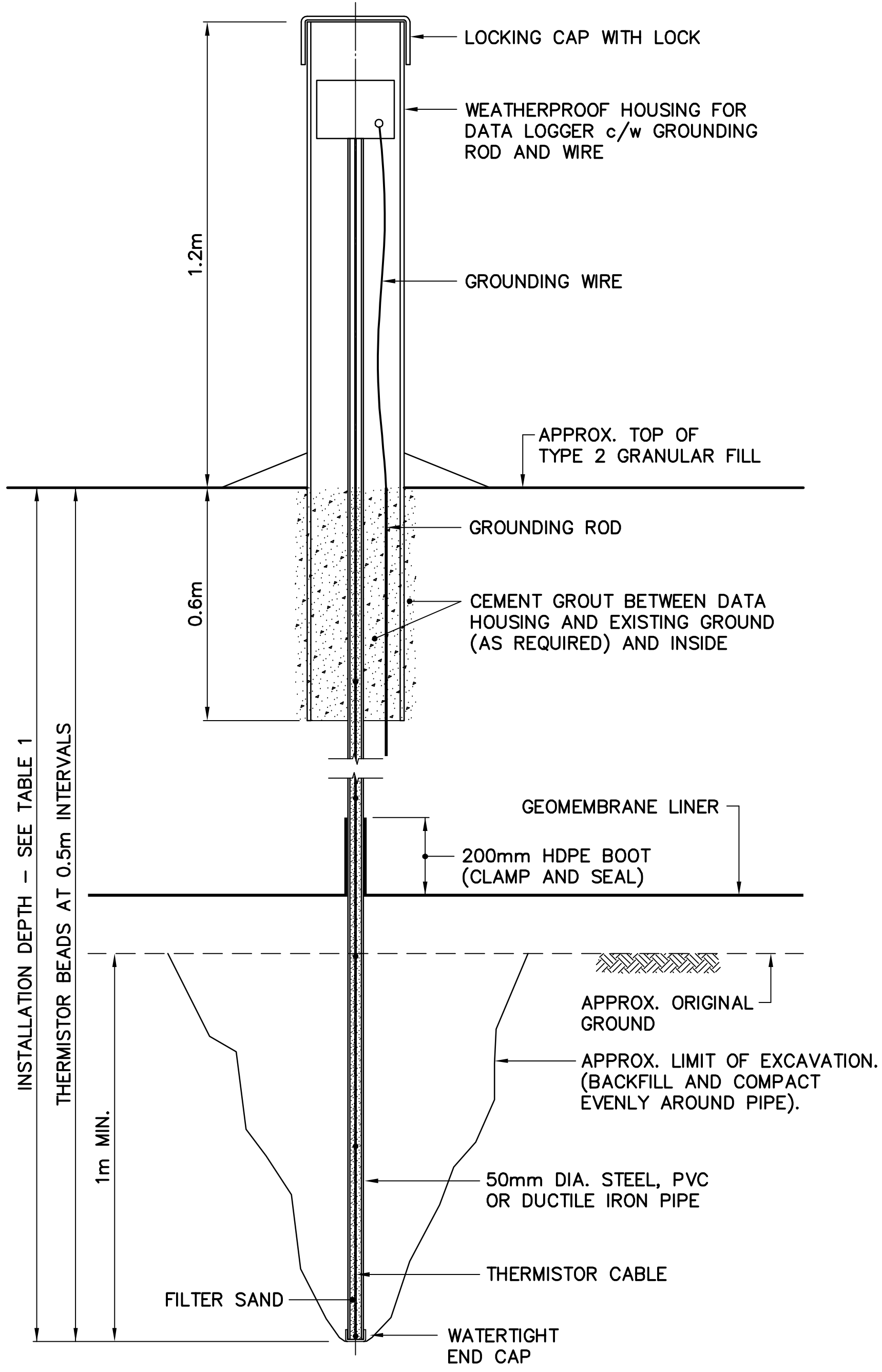
TYPICAL GROUND TEMPERATURE CABLE INSTALLATION – PLATEAU N.T.S.
