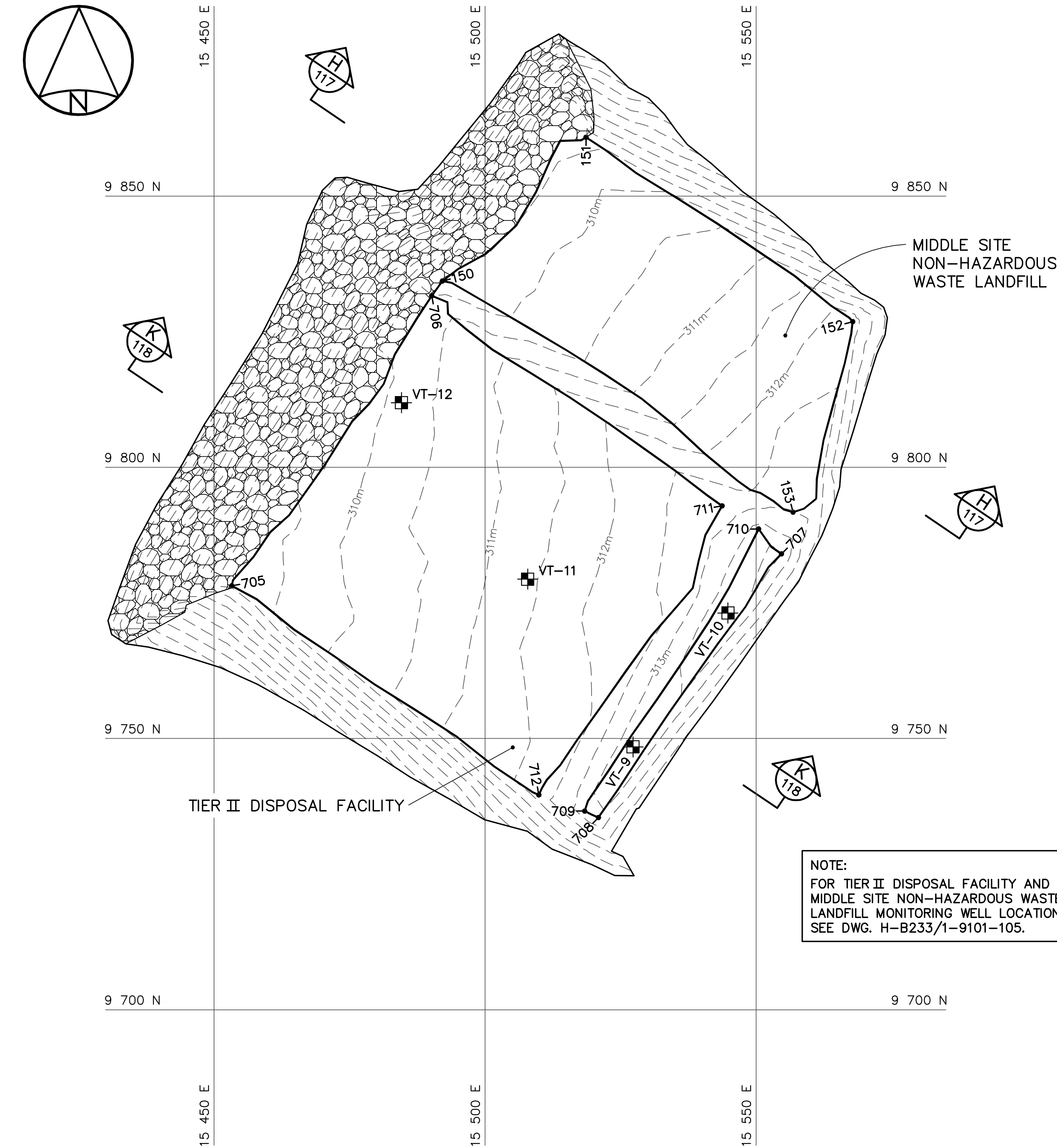
GRADING/INSTRUMENTATION PLAN
