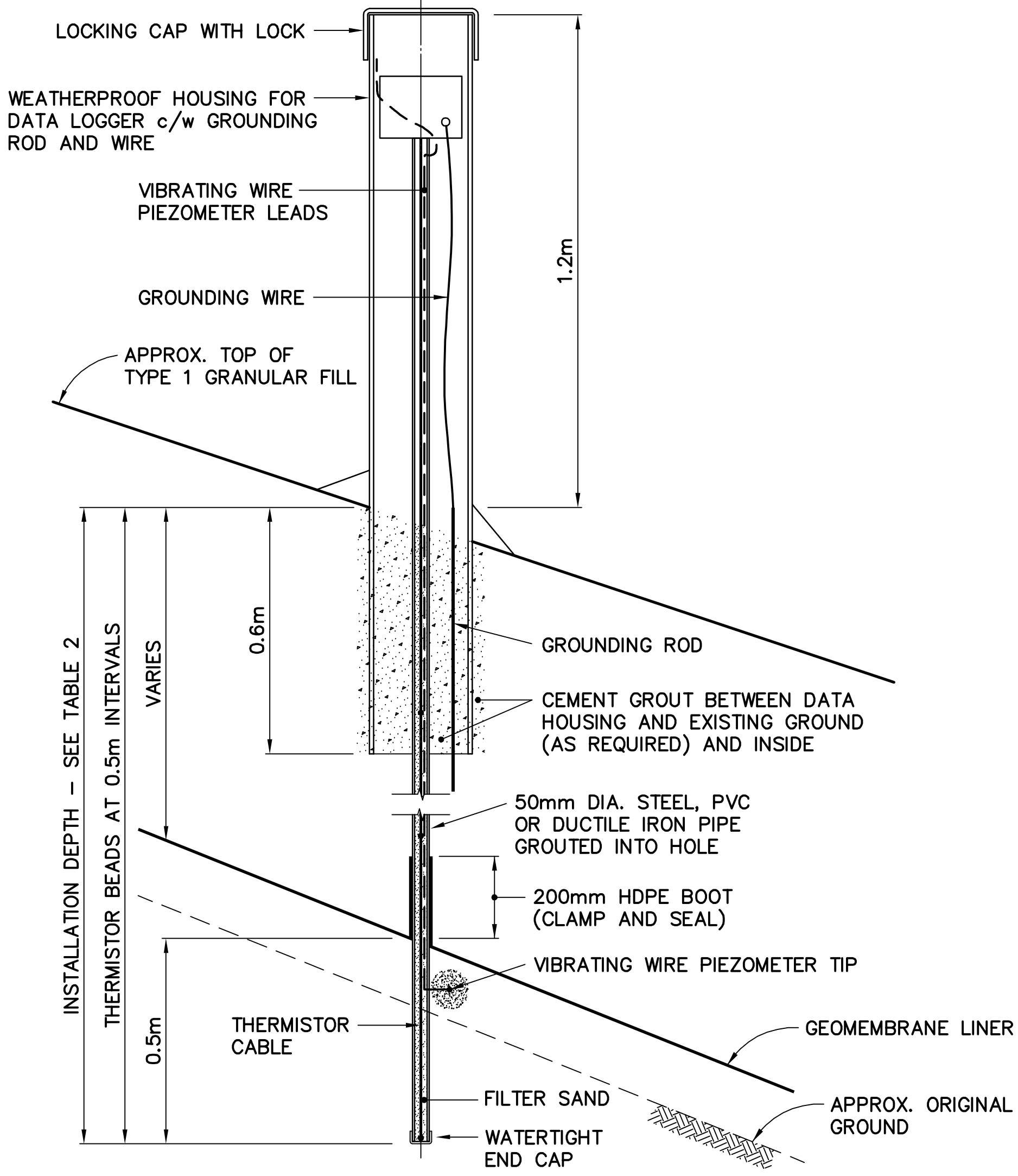
TYPICAL GROUND TEMPERATURE CABLE INSTALLATION – SLOPES (WITH PIEZOMETER) N.T.S.
