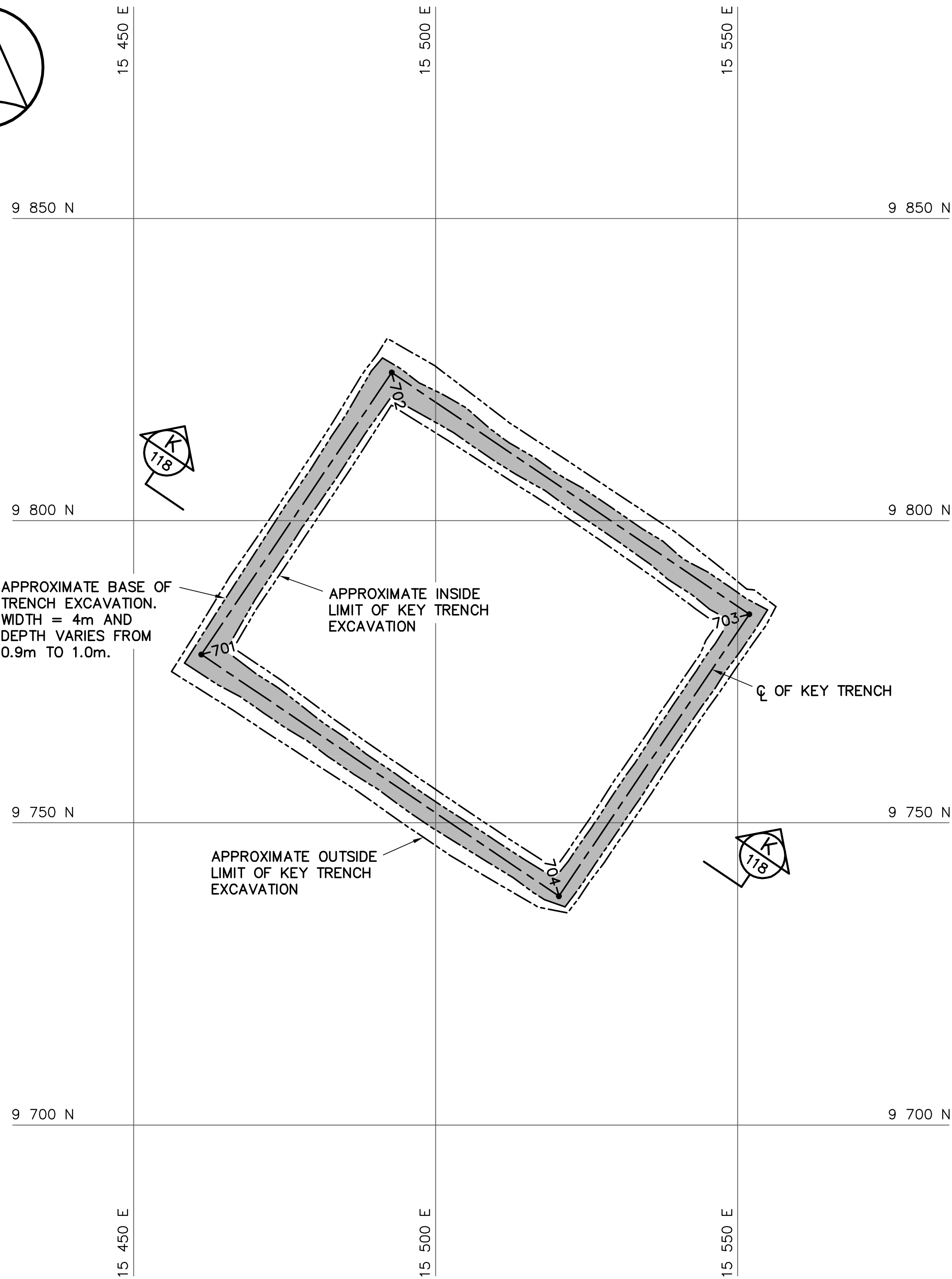
KEY TRENCH EXCAVATION PLAN
