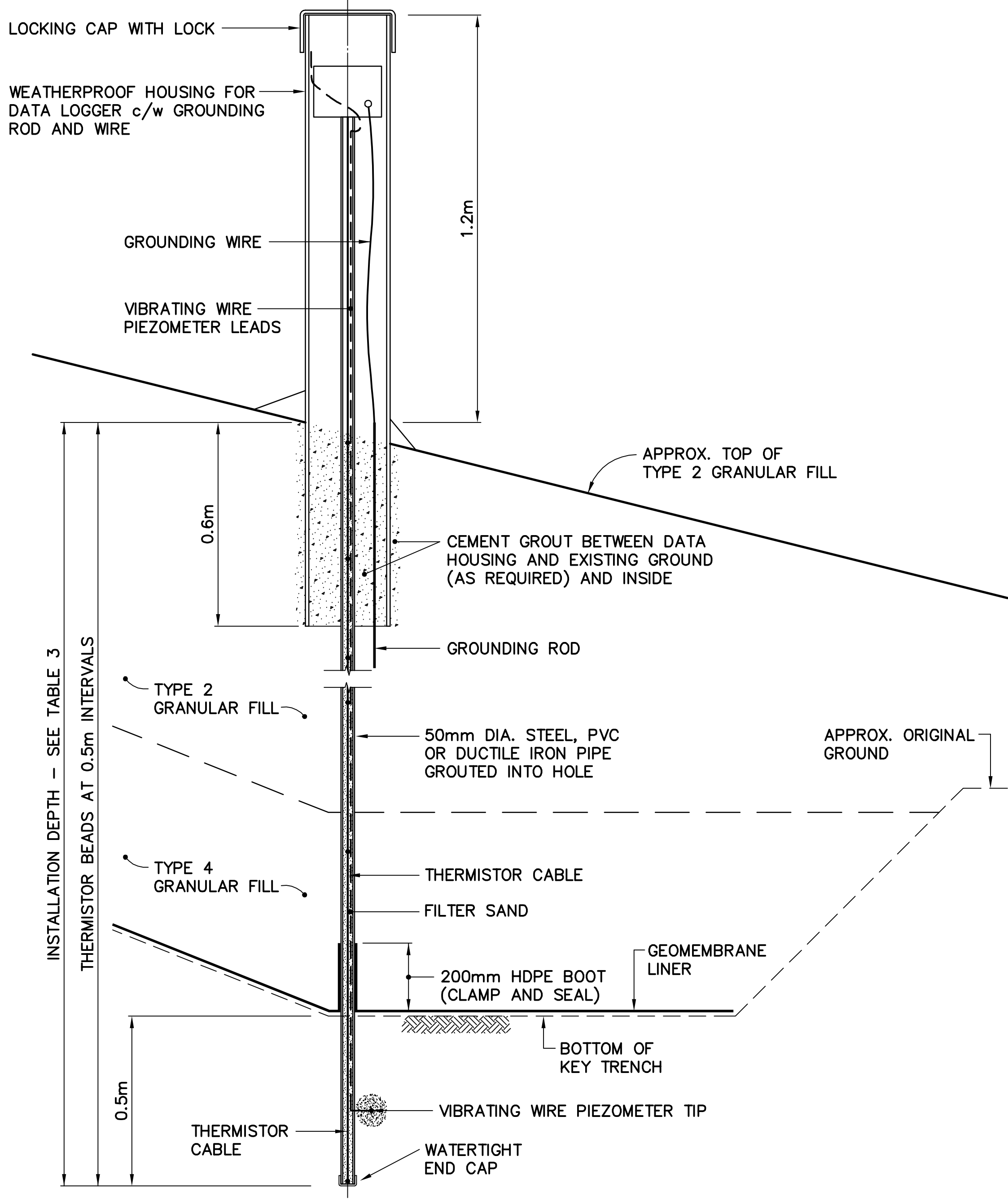
TYPICAL GROUND TEMPERATURE CABLE INSTALLATION – KEY TRENCH (WITH PIEZOMETER) N.T.S.
