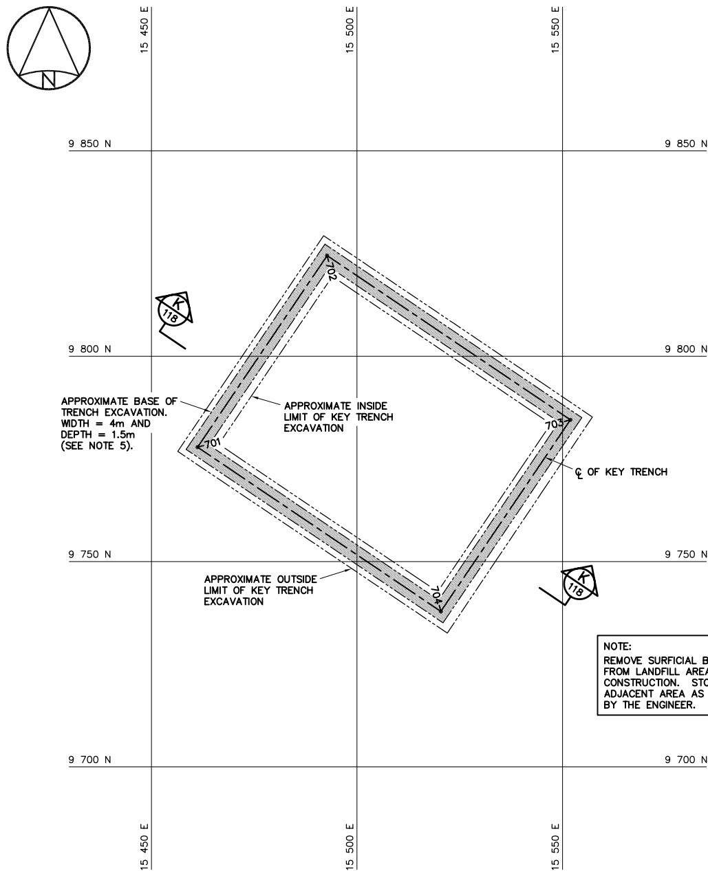
KEY TRENCH EXCAVATION PLAN
