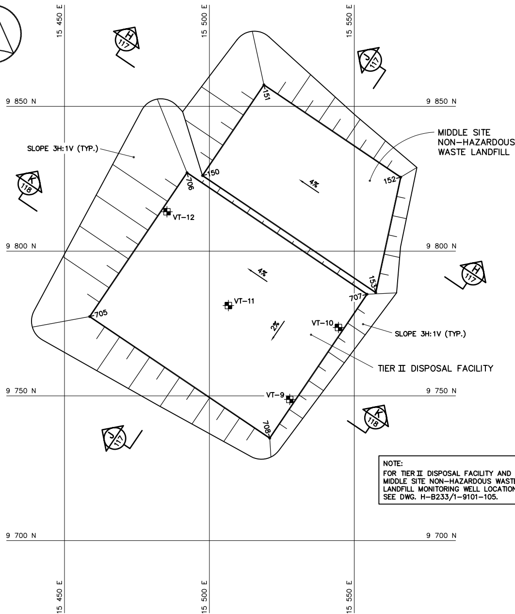
GRADING/INSTRUMENTATION PLAN
