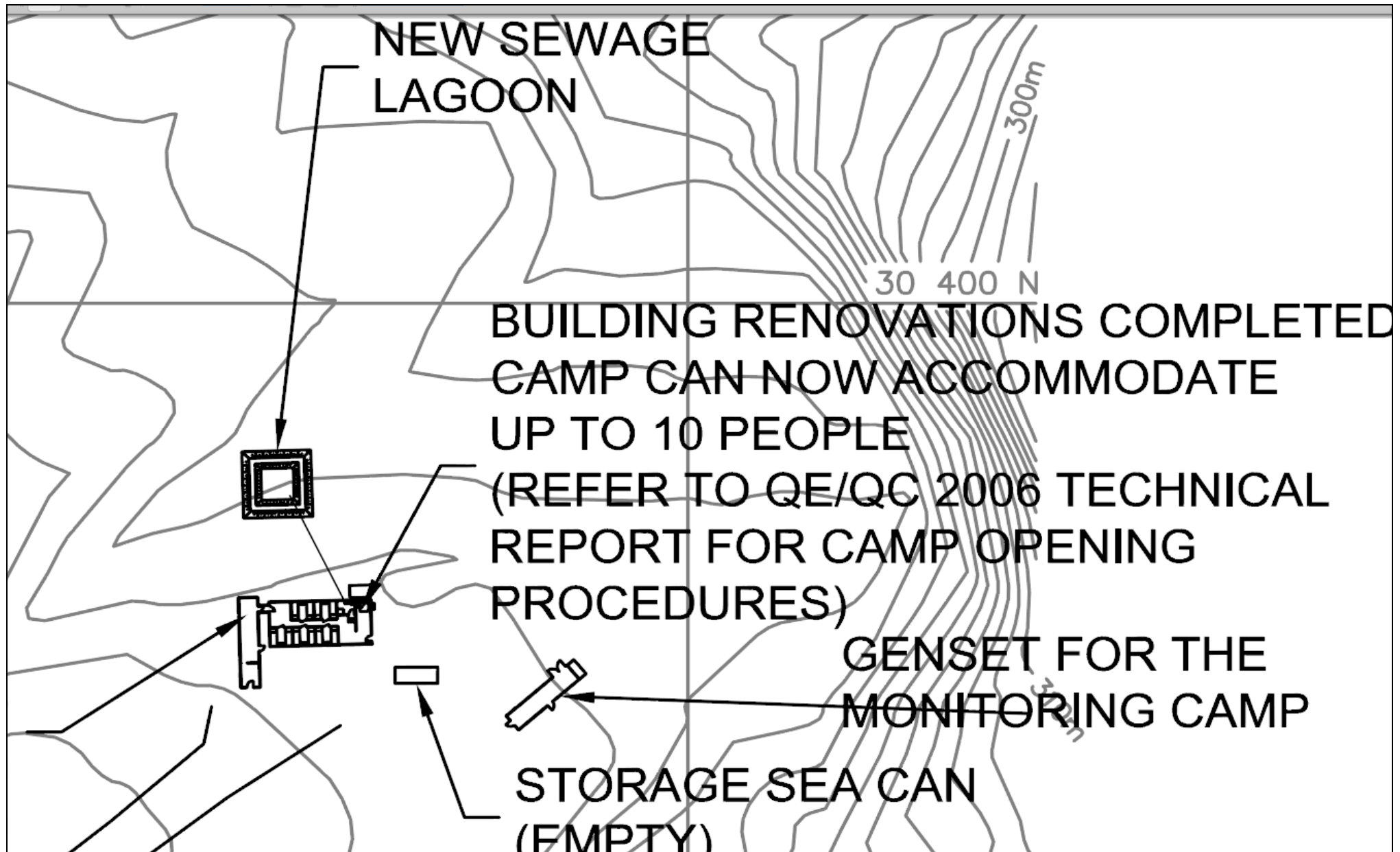
Map 5 - Excerpt from 2007 Final As-Built Drawings for Resolution Island Remediation Project showing Monitoring Camp Layout
