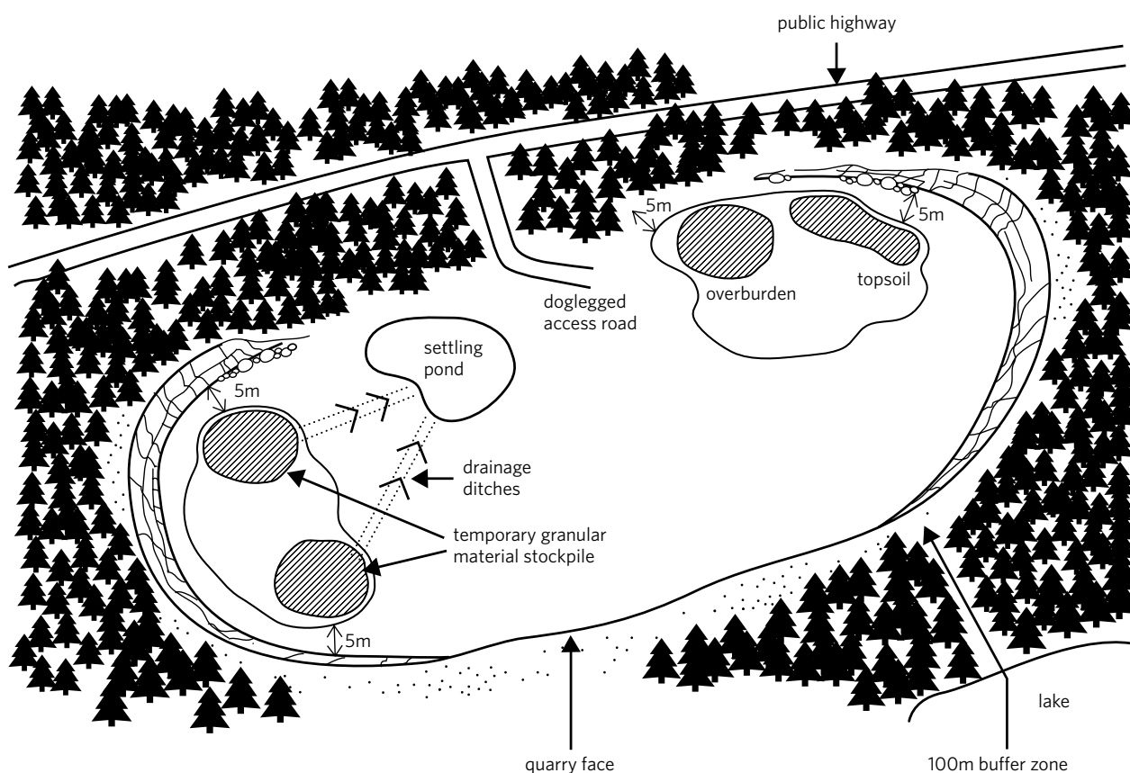
FIGURE 8. A well-designed quarry.
