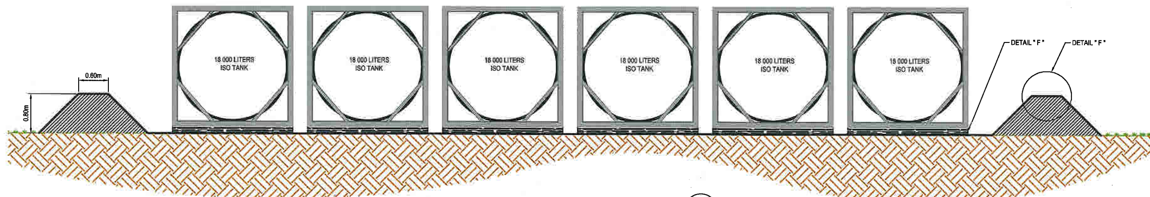
SECTIONAL VIEW OF TYPICAL FUEL CONTAINMENT BASIN C SECTION C-C F 2
