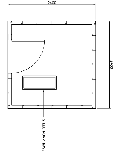
FLOOR PLAN
