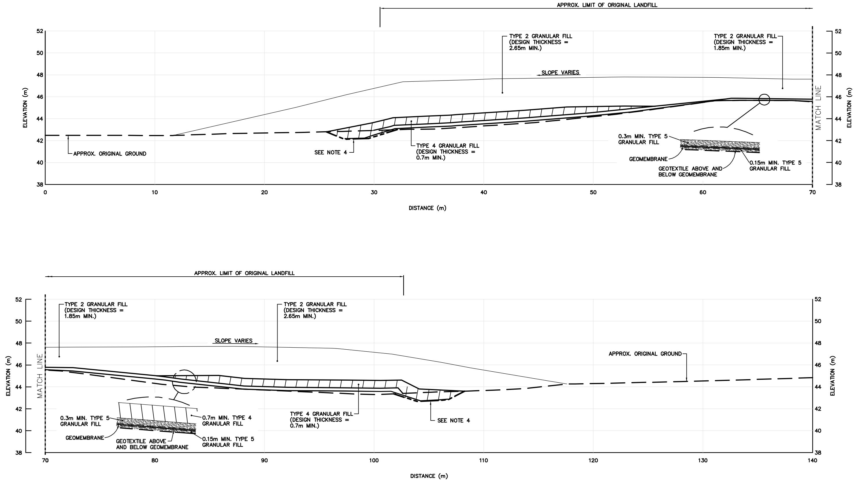
DEW Line Cleanup Landfill Monitoring Plan CAM-3 Shepherd Bay USAF Landfill Cross Section Figure CAM 3.7B
