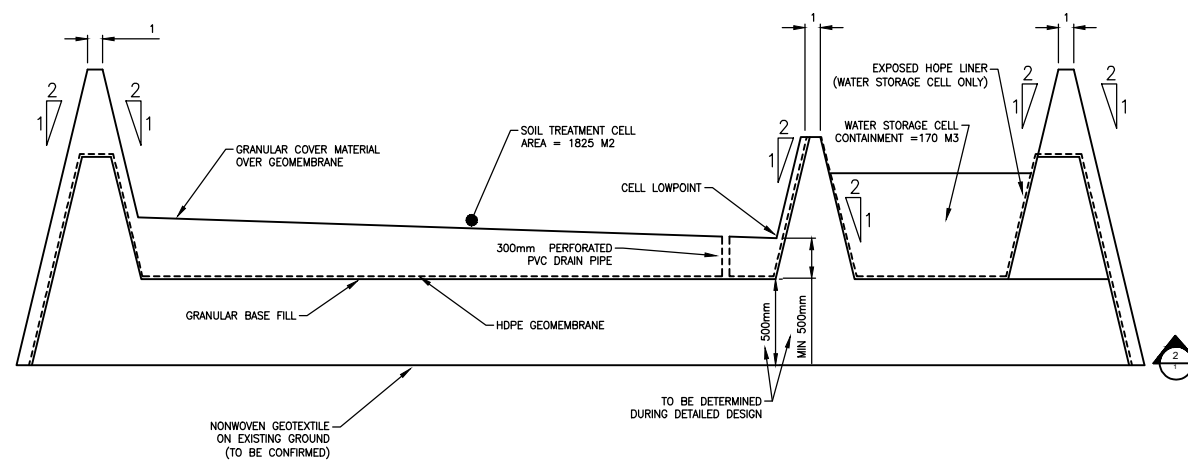
SECTION
