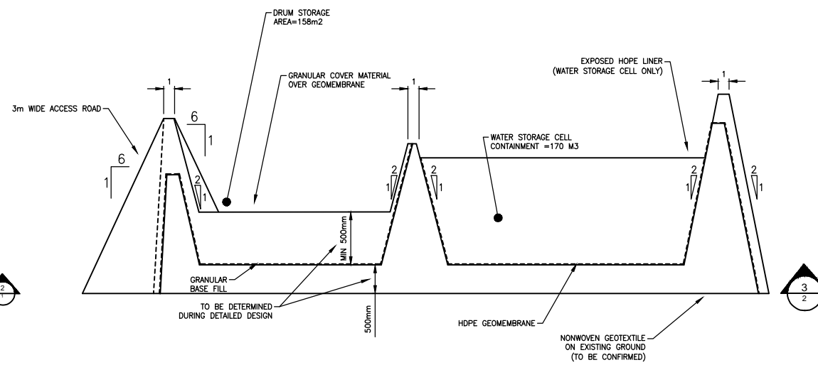
SECTION
