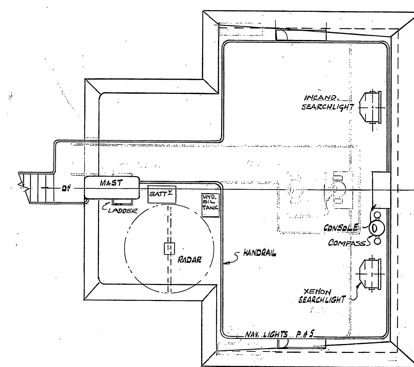
WHEELHOUSE TOP
