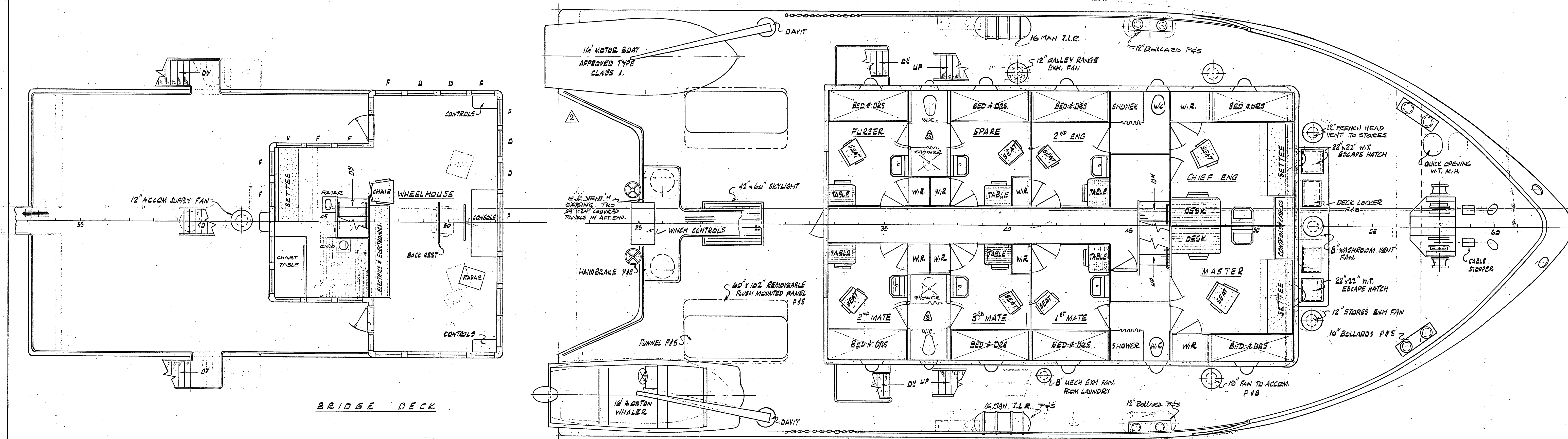
FORECASTLE DECK
