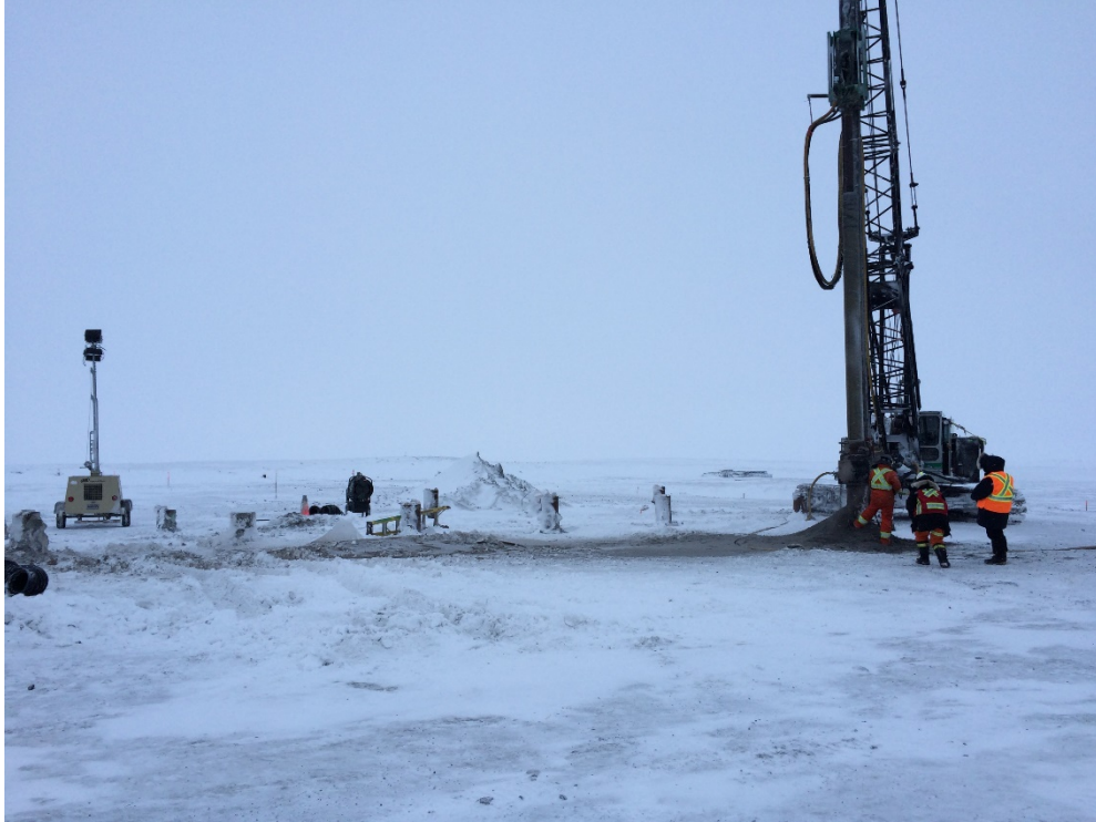
Photo 5 : Piling installation, December 2015
