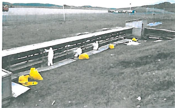
Photo 2: Exposing utilidor for asbestos abatement
