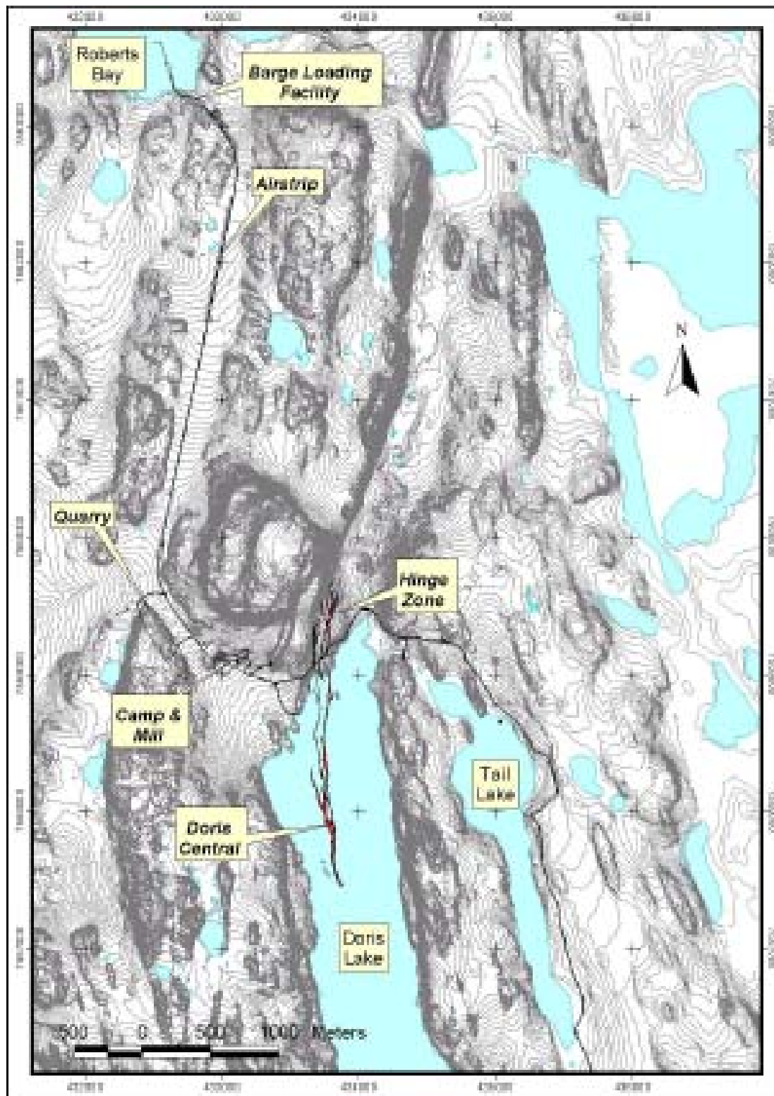
Figure 4-1: Surface Expression of Ore Zones
