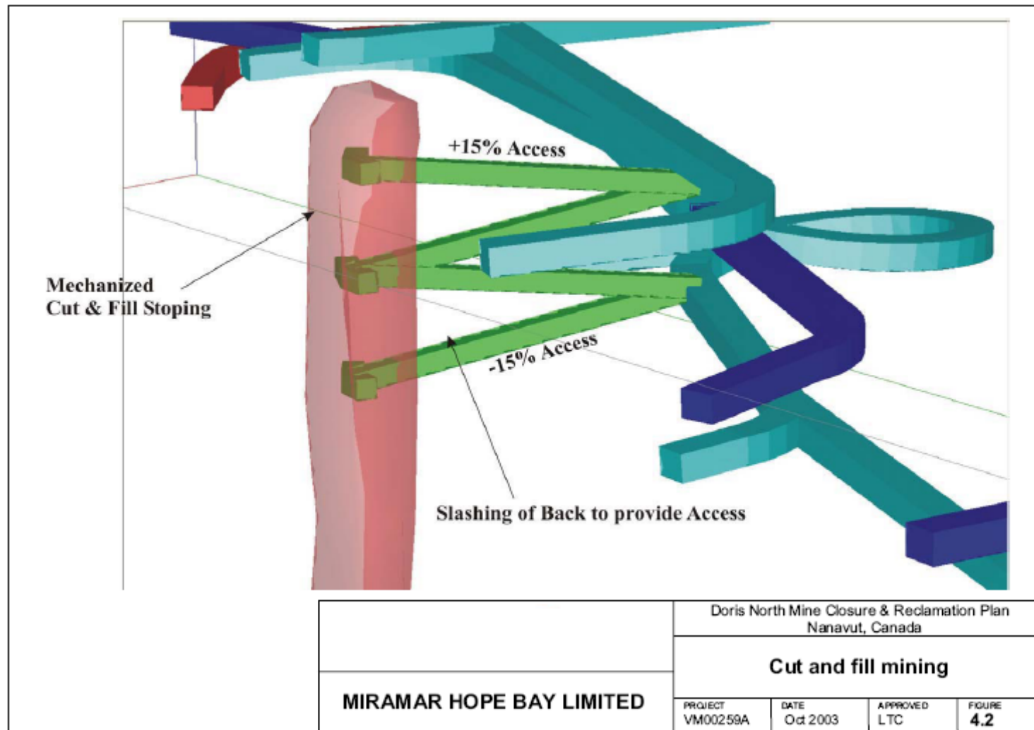
Figure 4-2: Cut and Fill Mining
