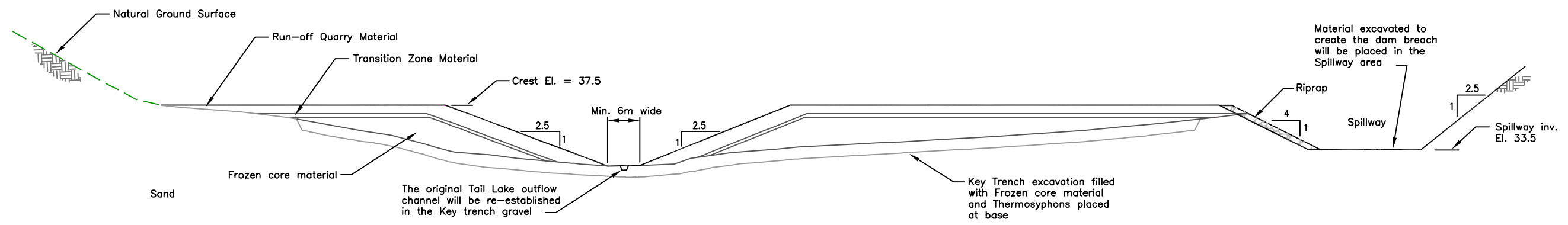
NORTH DAM LONGITUDINAL SECTION A-A' 1:400 0 100 200 300 400 Metres 2x Vertical Exaggeration
