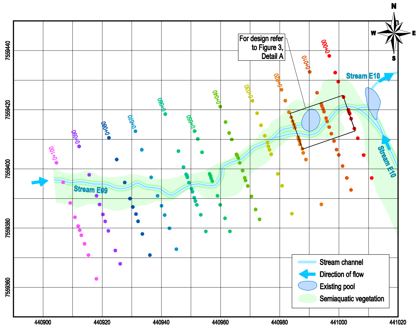
Plan View
