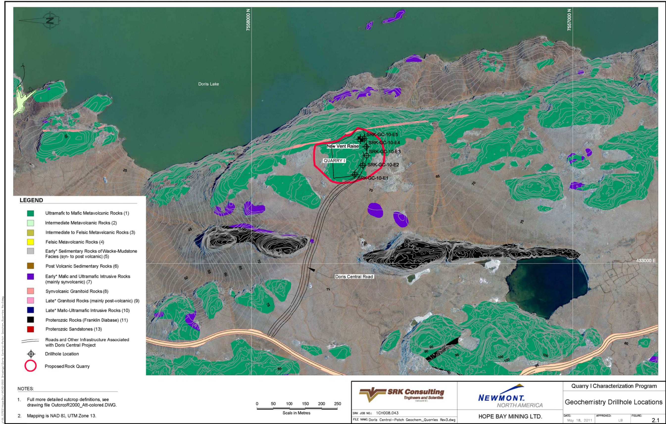
Figure 2.1: Location of Geochemistry Drillholes for Quarry I, Doris
