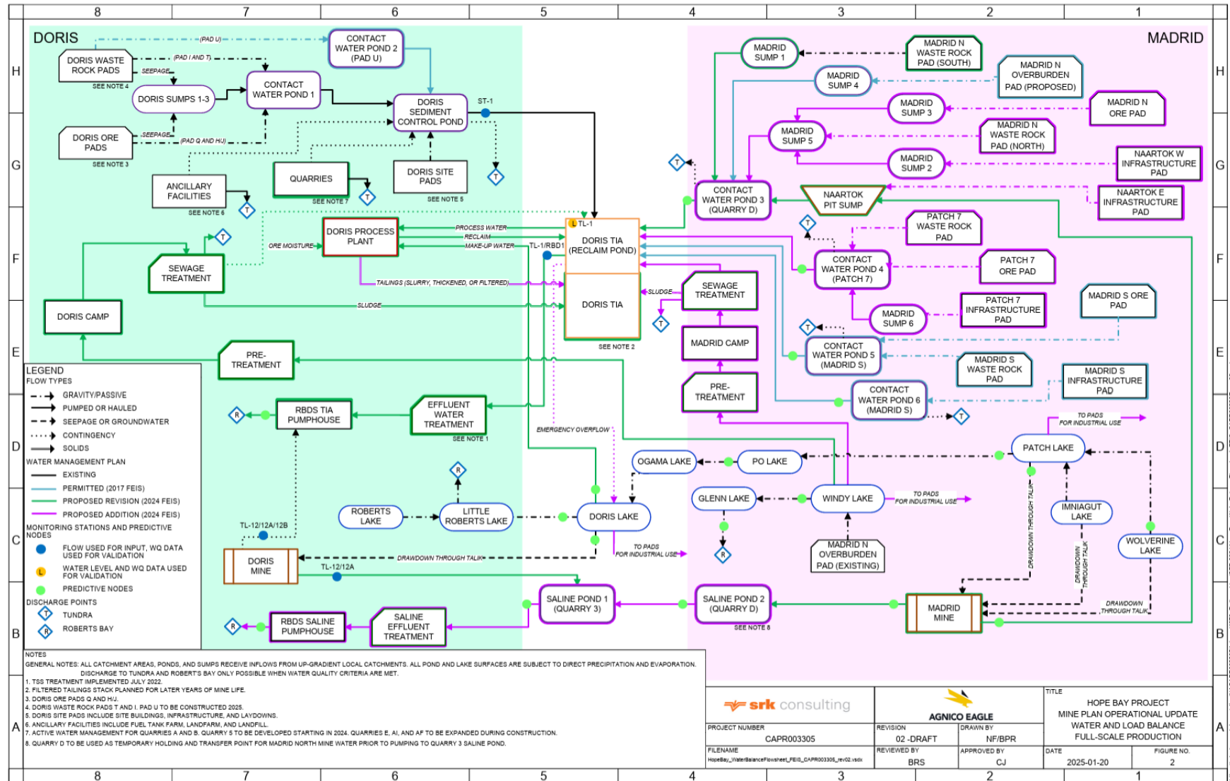
Figure 1 Water Management Flow Diagram-Doris and Madrid
