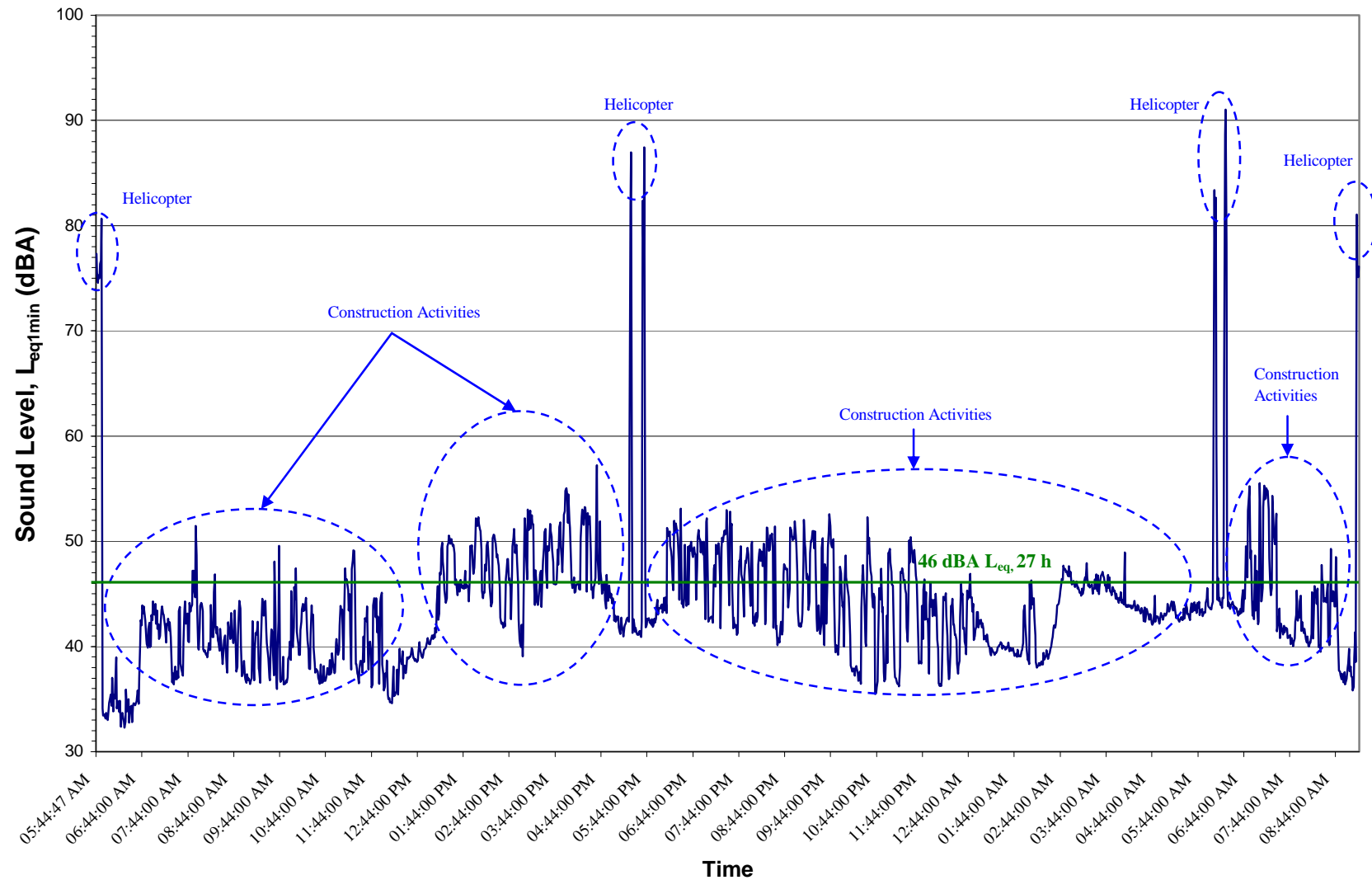
Figure 4.1 One - Minute Noise Levels, NM-1, July 25 and 26, 2007
