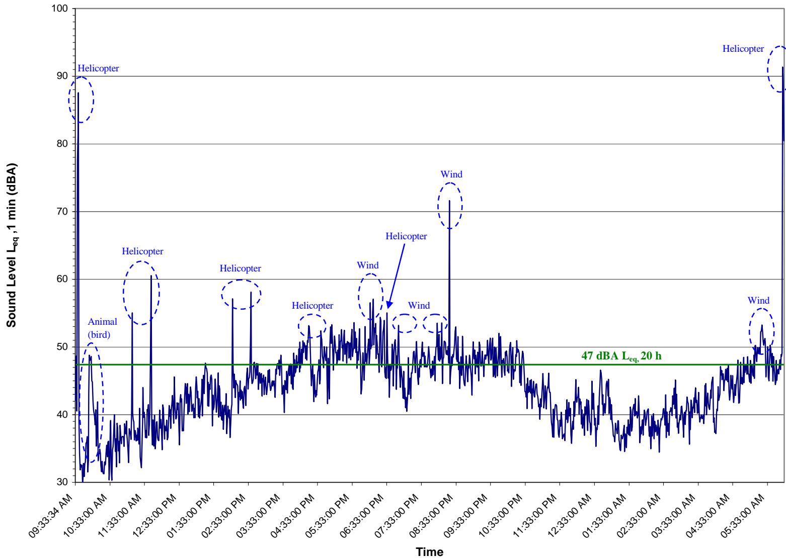
Figure 4.4 One - Minute Noise Levels, NM-4, July 26 and 27, 2007
