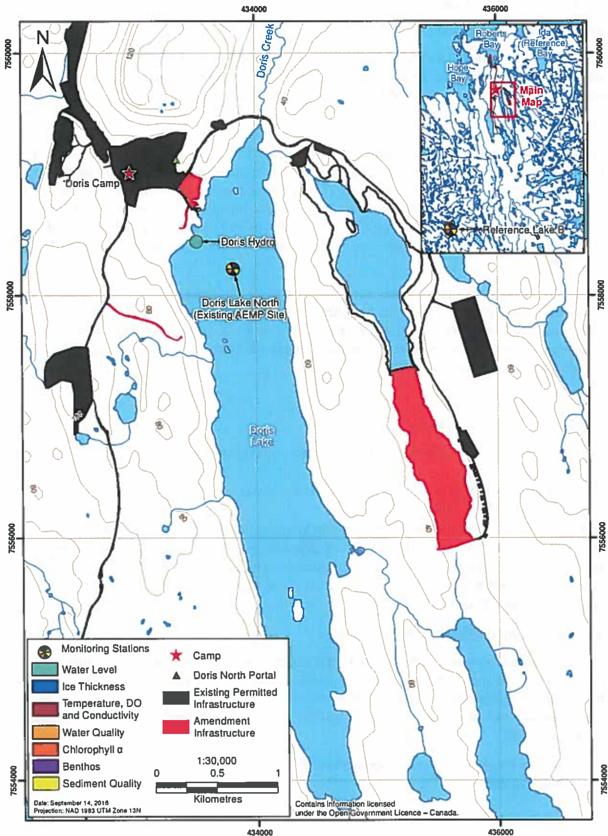
Figure 3.1-1 AEMP Monitoring Stations
