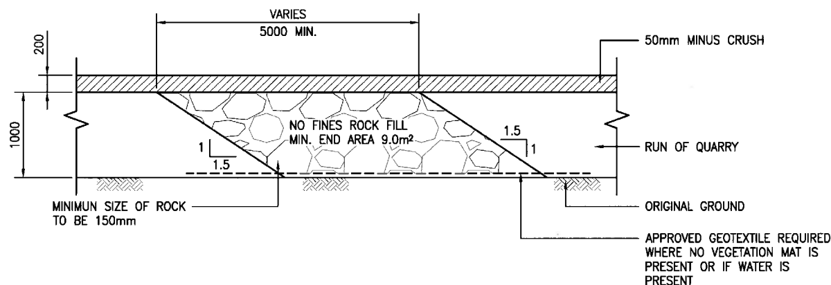
FLOW THROUGH ROCK DRAIN INSTALLATION DETAIL IN PERMAFROST AND NON-PERMAFROST
