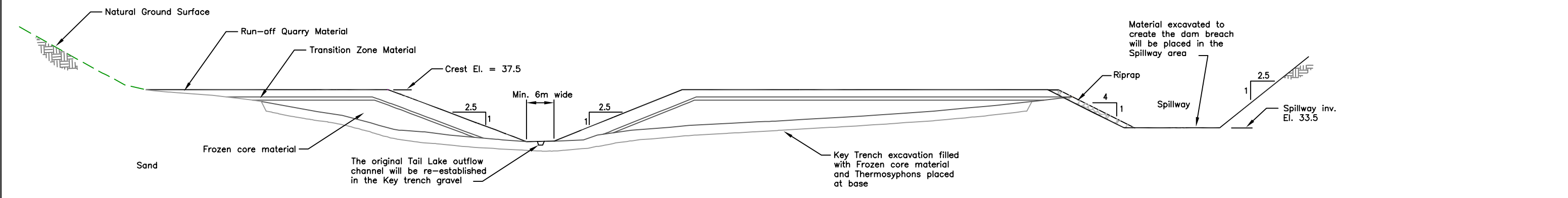
NORTH DAM LONGITUDINAL SECTION A-A' 1:400 0 100 200 300 400 Metres 2x Vertical Exaggeration
