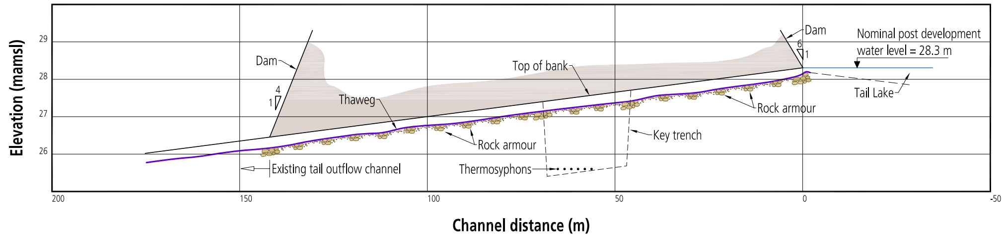
Longitudinal profile view
