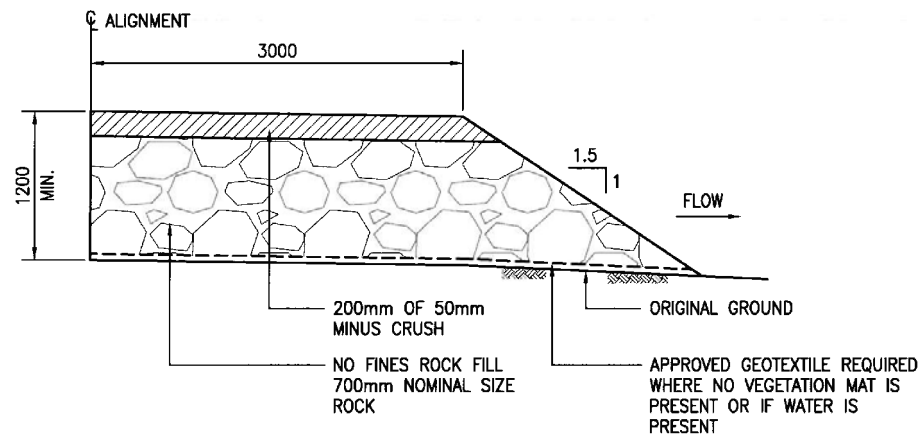
FLOW THROUGH ROCK DRAIN
