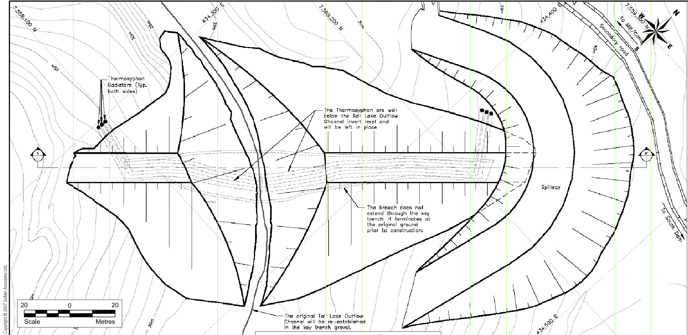
Beached North Dam Plan Layout
