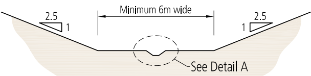
Typical section
