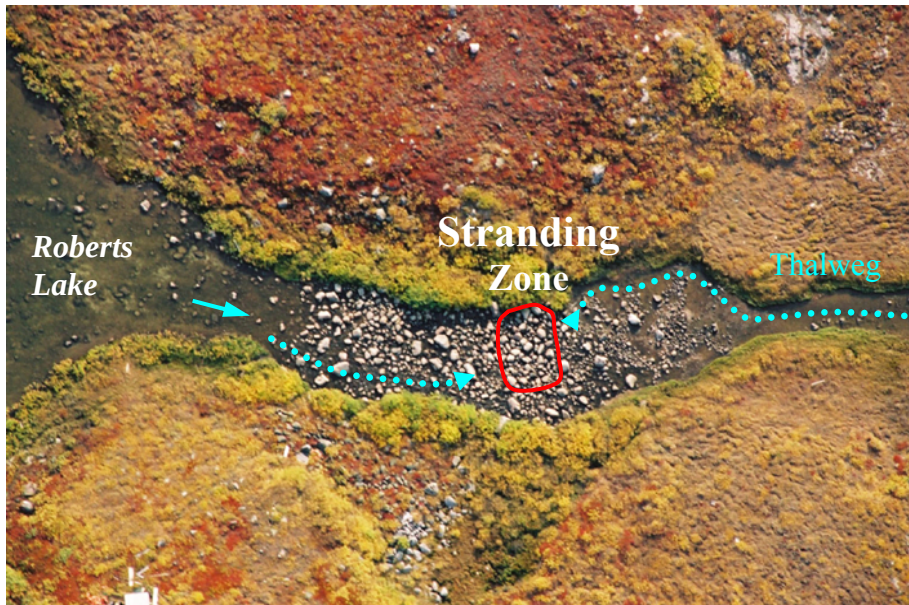
Plate 7 Roberts Outflow, 2 September 2002. Aerial view of boulder garden. Outflow thalweg crosses channel through stranding zone of boulder garden.
