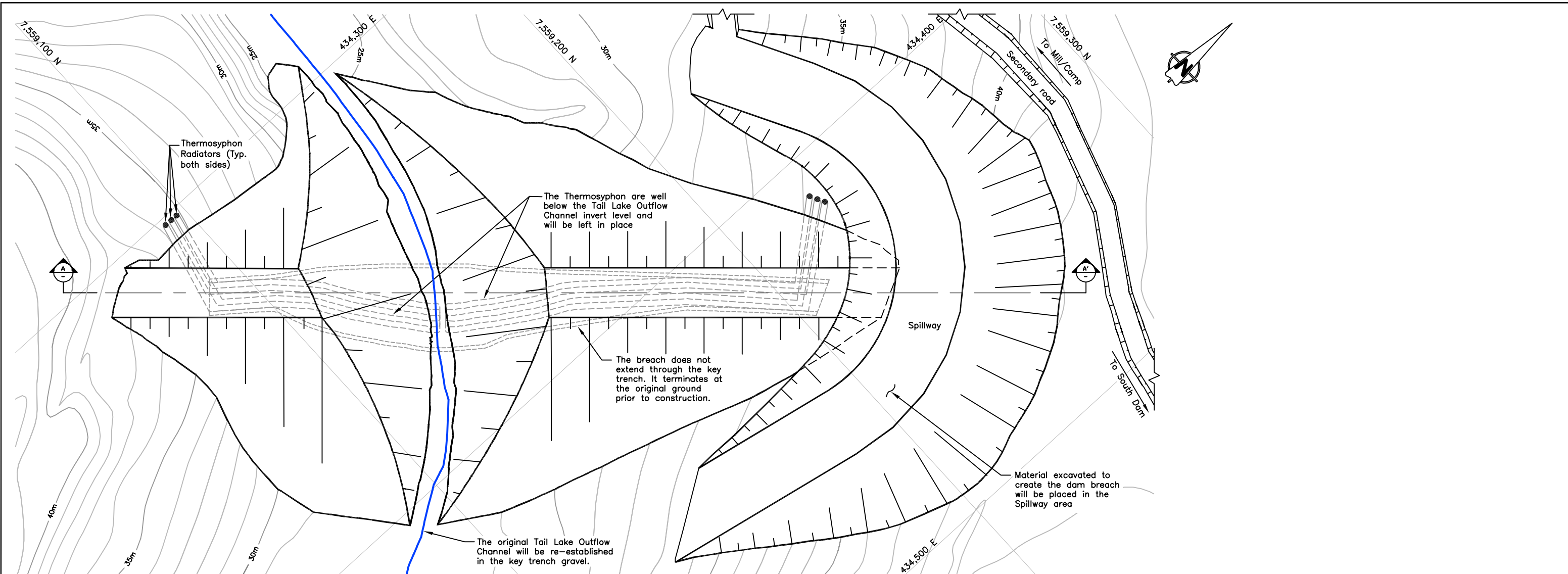
BREACHED NORTH DAM PLAN LAYOUT 1:500 0 10 20 30 40 50 Metres
