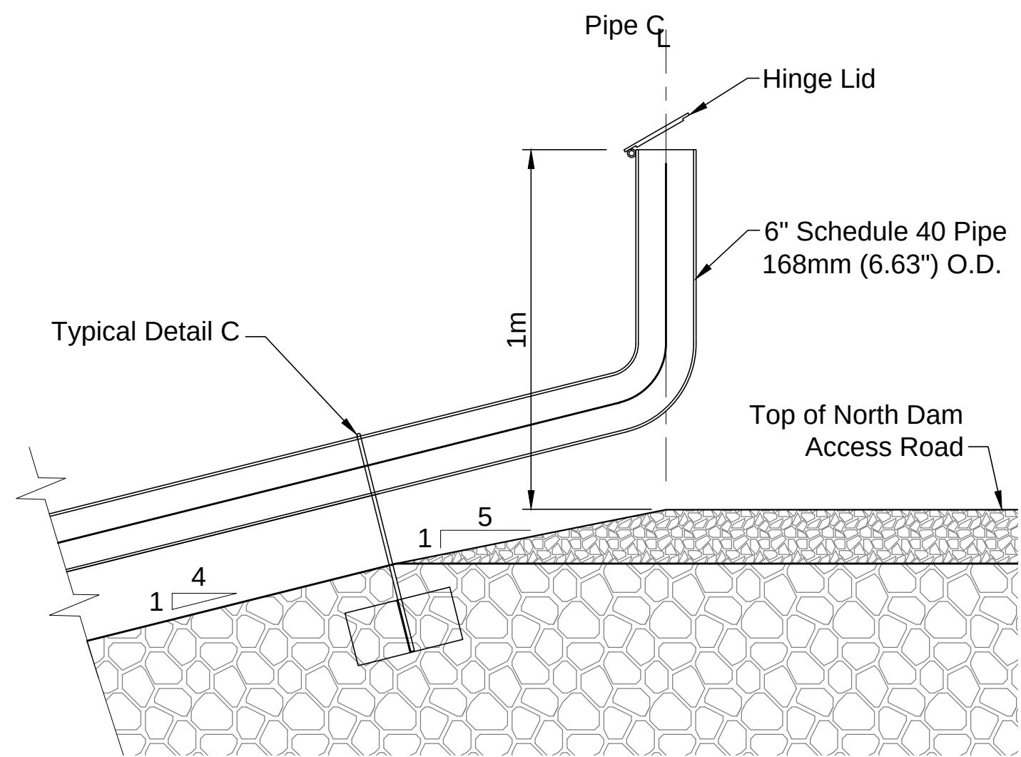
A THERMISTOR TYPICAL DETAIL Not to Scale
