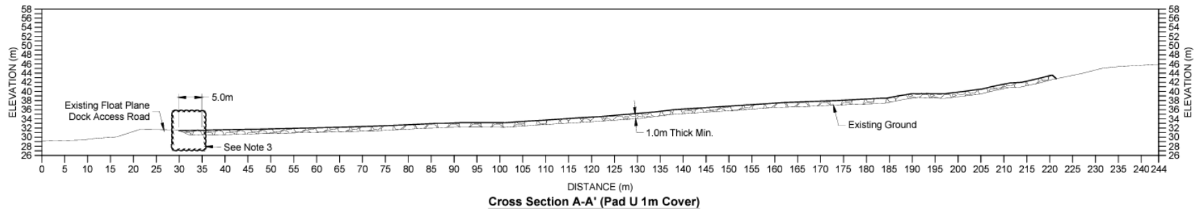
Figure 2 – Cross Section of Pad U Laydown
