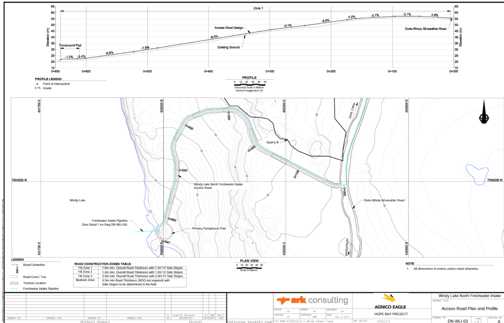
Figure 4 – Windy North Intake Access Road Plan
