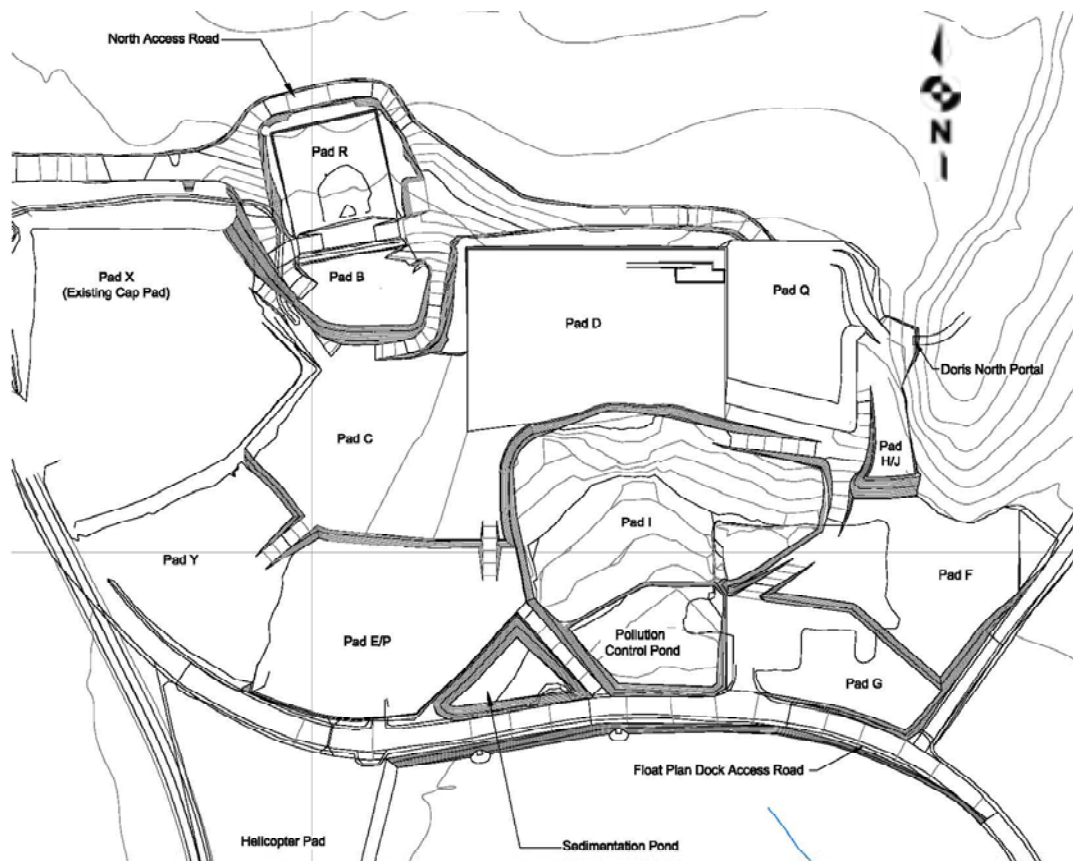
Figure 2: Plan of Surface Facilities
