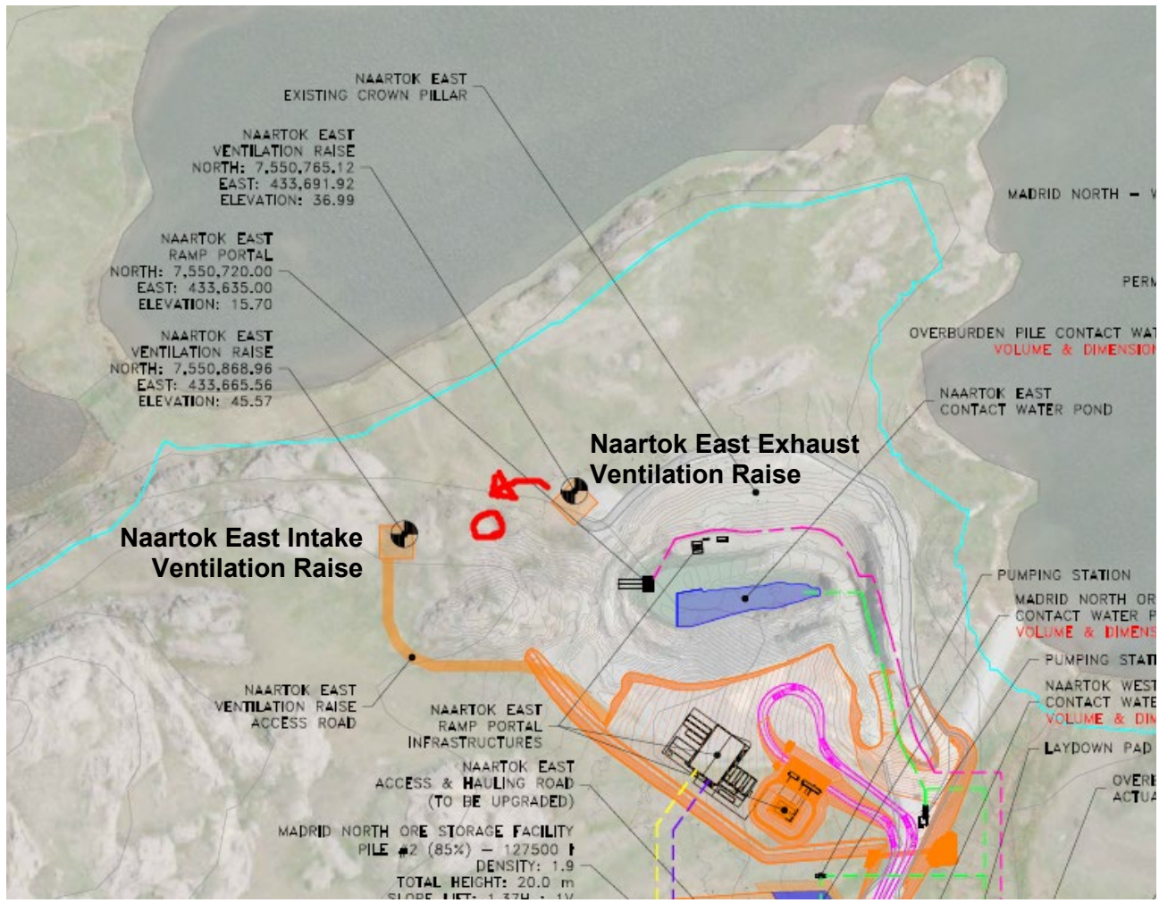
Figure 1 – Naartok East Exhaust Ventilation Raise Move
