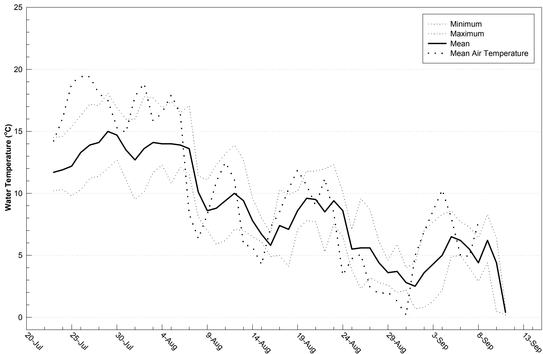
Figure 3.8 Daily water temperatures in Stream C3, Jericho Study Area (July to September 2000).
