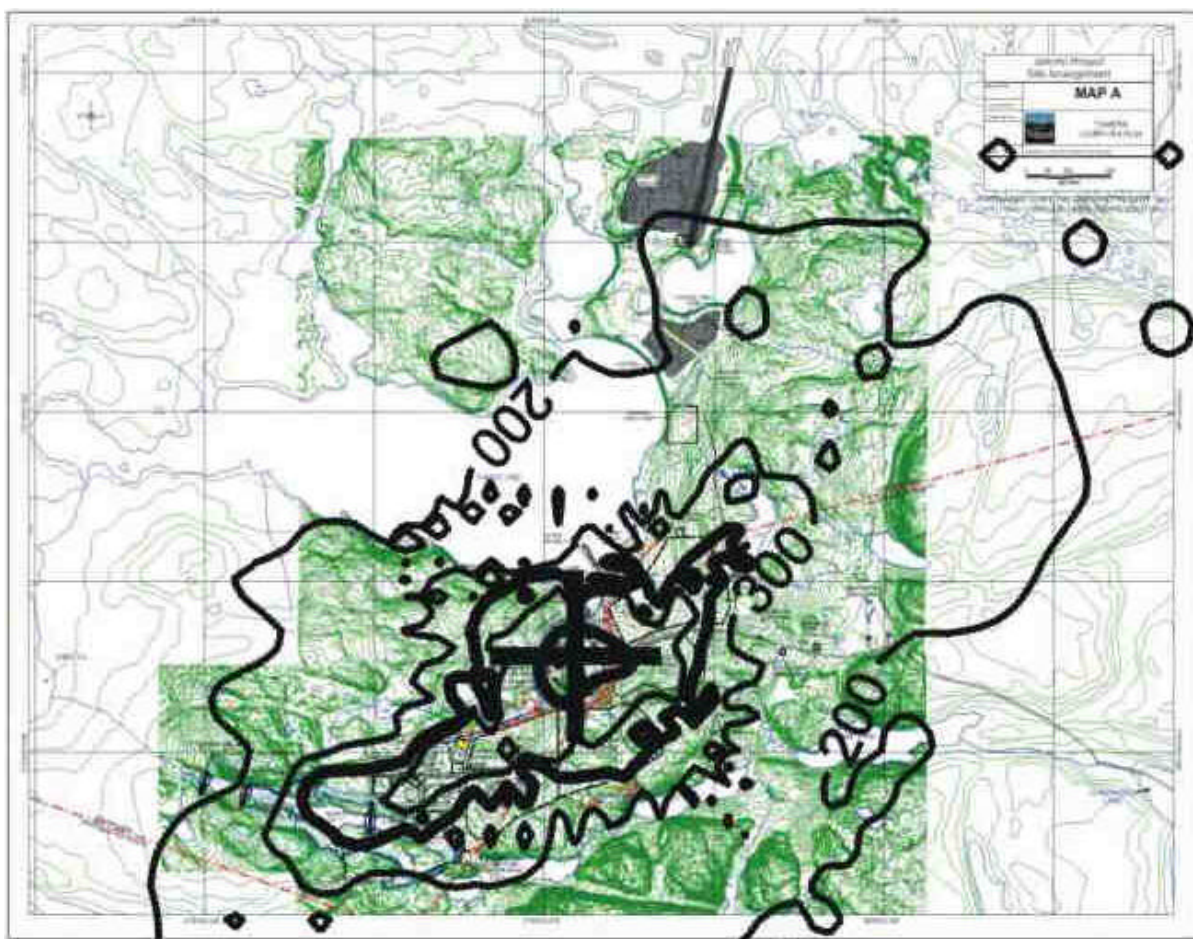
Figure 4.3b Maximum 1-hour NO 2 concentration assuming ozone limiting. The cross indicates the location of the mine pit. Contour plot placed on base map.
