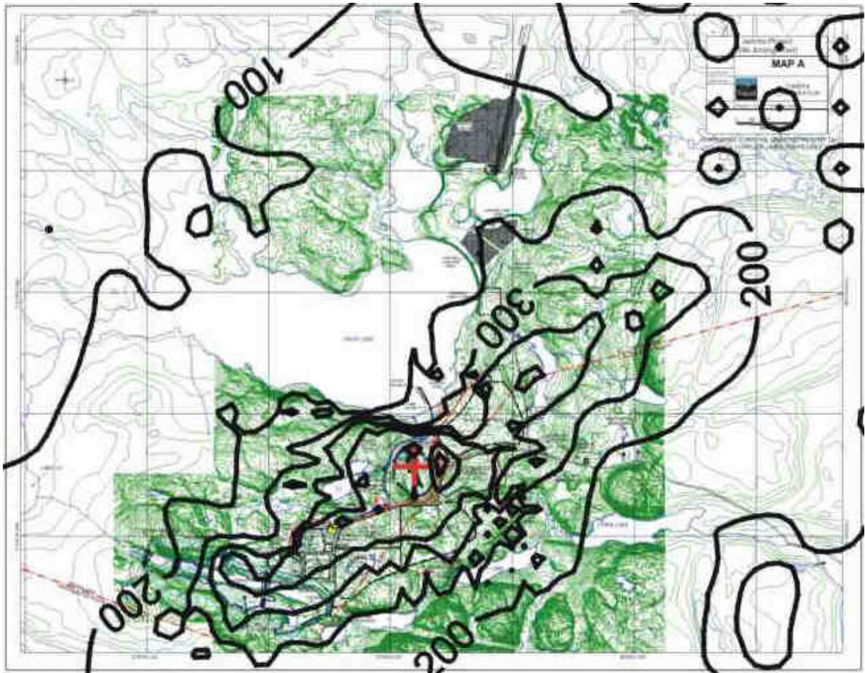
Figure 4.6b Maximum 24-hour concentration of PM10 with water spraying of roads and stockpiles. The cross locates the mine pit. Contour plot placed on base map.
