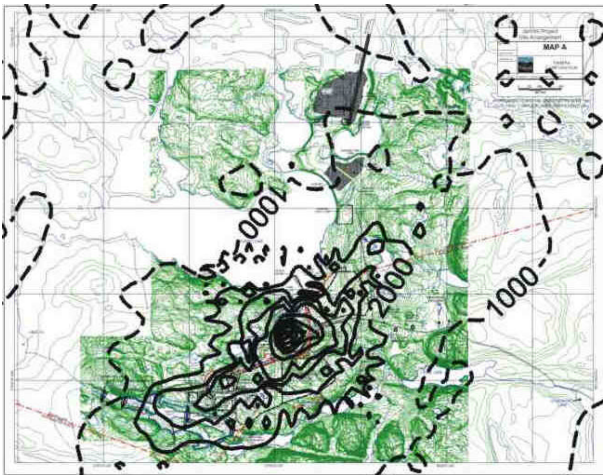
Figure 4.2b Maximum 1-hour \text{NO}_x concentrations for all sources. The dashed contours are for 400 \mu\text{g}/\text{m}^3 and 1000 \mu\text{g}/\text{m}^3 . The cross indicates the centre of the mine pit. Contour plot placed on base map.
