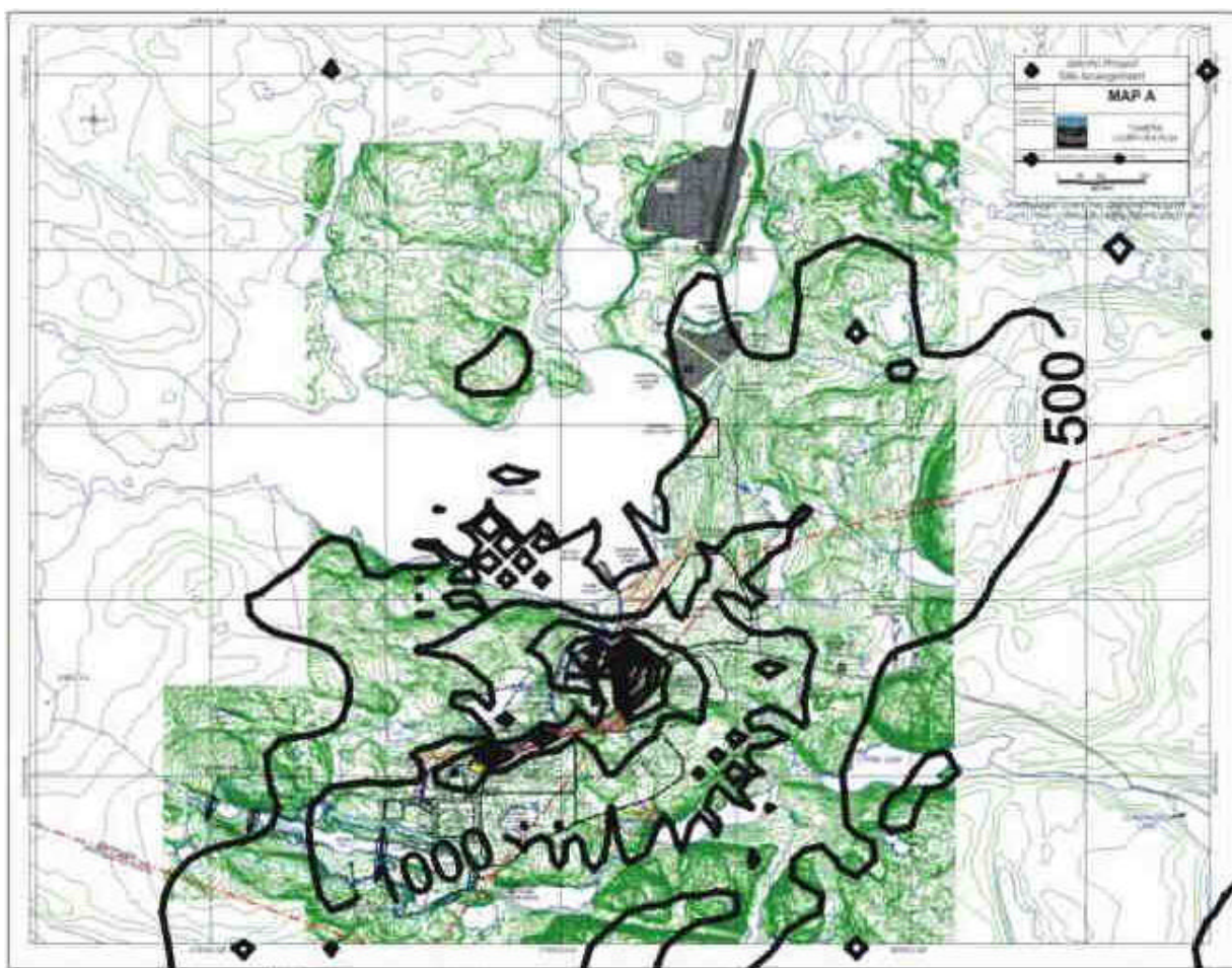
Figure 4.5b Maximum 24-hour concentration of PM 10 . The cross locates the mine pit. Contour plot placed on base map.
