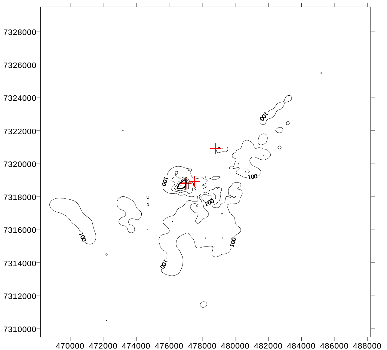
Figure 4.1 Maximum 1-hour NO x concentrations for stationary sources. Contours are every 100 \mu\text{g}/\text{m}^3 . The crosses indicate the locations of the stationary sources.
