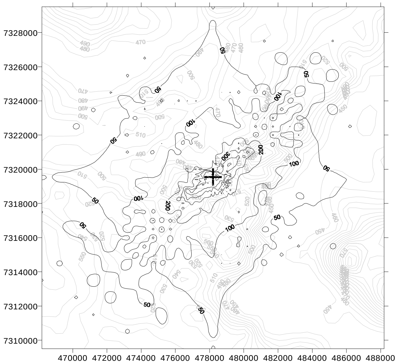
Figure 4.6 Maximum 24-hour concentration of PM10 with water spraying of roads and stockpiles. The light contours show the local topography and the cross locates the mine pit.
