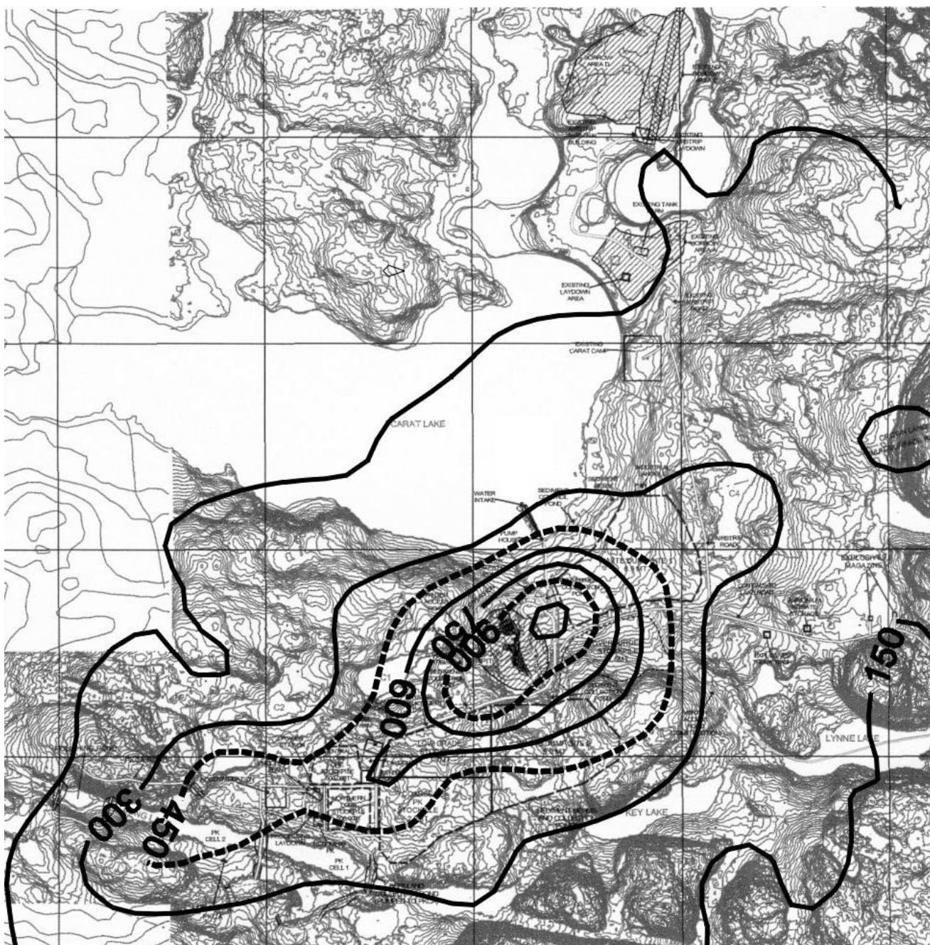
Figure 4.4 Maximum 1-hour concentration of SO 2 superimposed on a base map of the Jericho site. The dashed contour lines indicate 450 µg/m 3 and 900 µg/m 3 .
