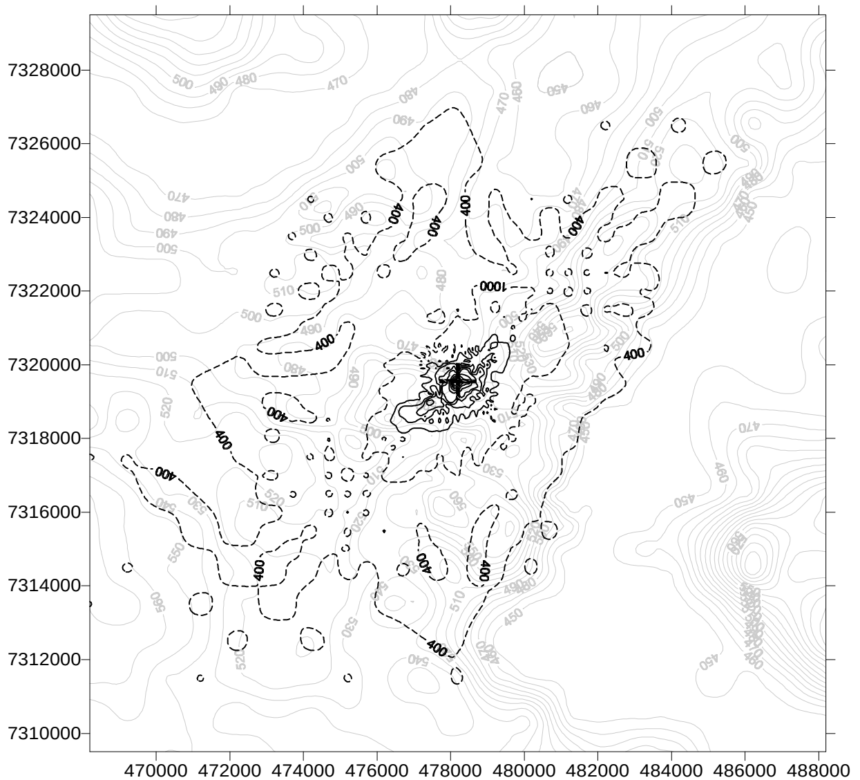
Figure 4.2 Maximum 1-hour NO x concentrations for all sources. The dashed contours are for 400 µg/m 3 and 1000 µg/m 3 . The cross indicates the centre of the mine pit. The light contours show the local topography.
