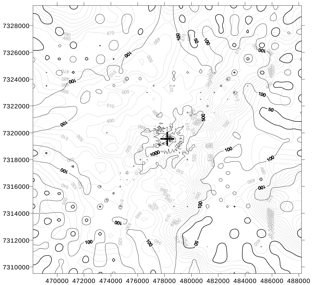
Figure 4.5 Maximum 24-hour concentration of PM 10 . The light contours represent the local topography and the cross locates the mine pit.
