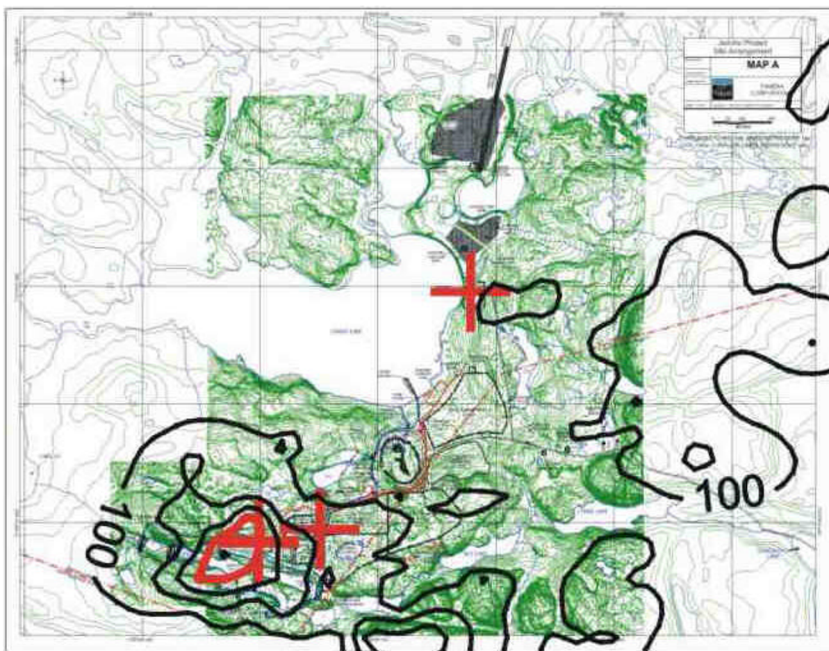
Figure 4.1b Maximum 1-hour \text{NO}_x concentrations for stationary sources. Contours are every 100 \mu\text{g}/\text{m}^3 . The crosses indicate the locations of the stationary sources. Contour plot placed on base map.
