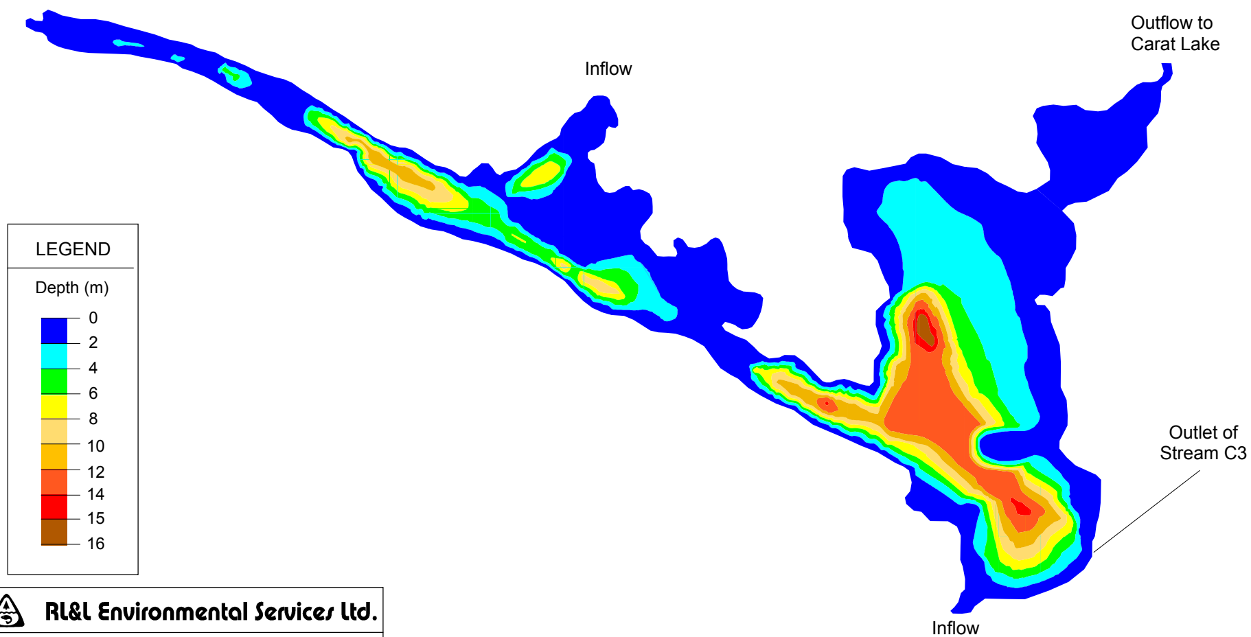
Figure 3.3 Bathymetric map of Lake C3, Jericho Study Area, 2000.
