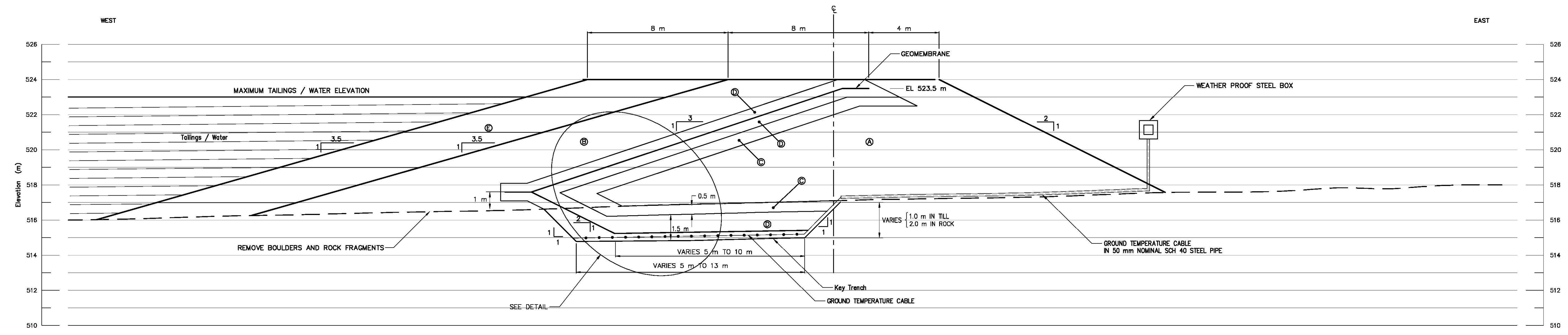
TYPICAL SECTION
