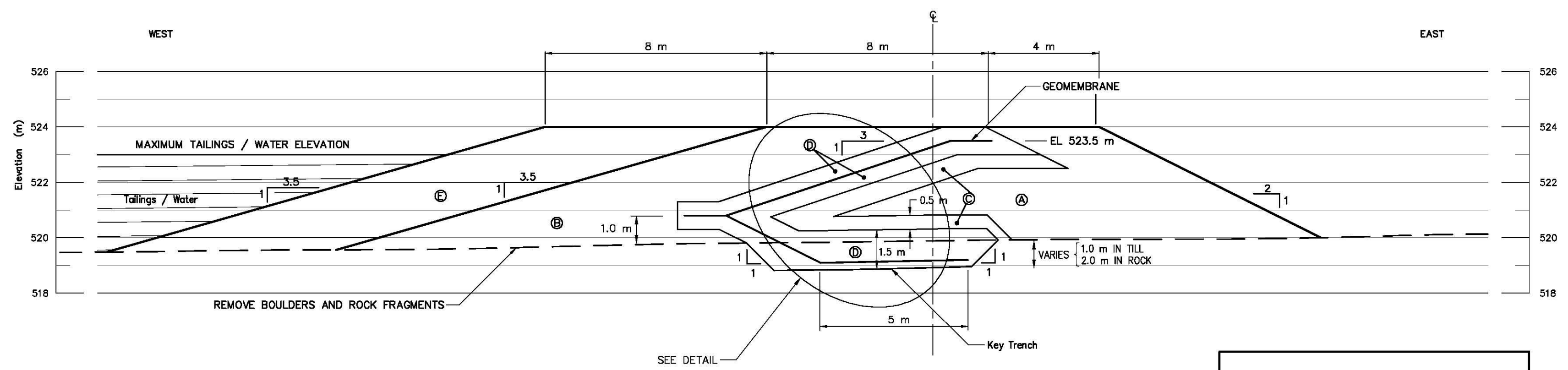
TYPICAL SECTION
