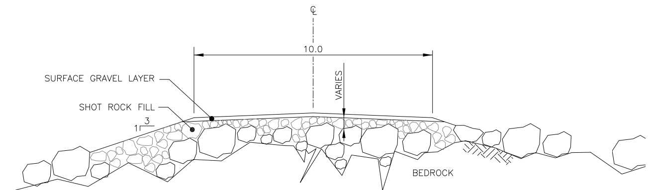
Figure 2.1-6 Typical Road Section on Frost Shattered and Boulder Covered Terrain (Terrain Type 4)
