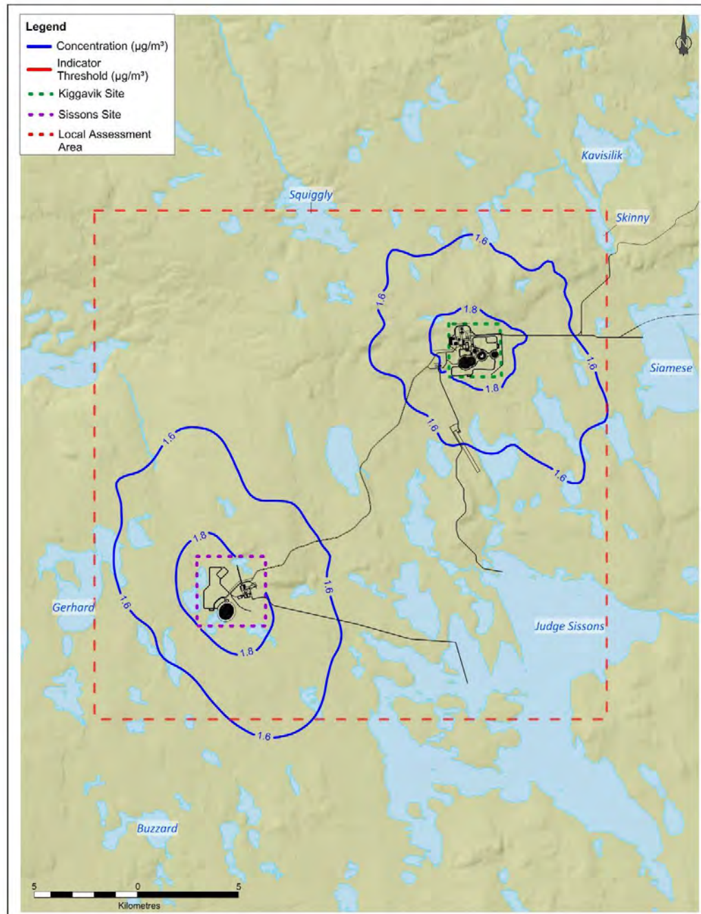
FIGURE D-88 Operation Assessment - Phase 4 Annual \text{PM}_{10} Concentration ( \mu\text{g}/\text{m}^3 ) ENVIRONMENTAL IMPACT STATEMENT VOLUME 4: ATMOSPHERIC ENVIRONMENT Technical Appendix 4B: AIR QUALITY AND CLIMATE
