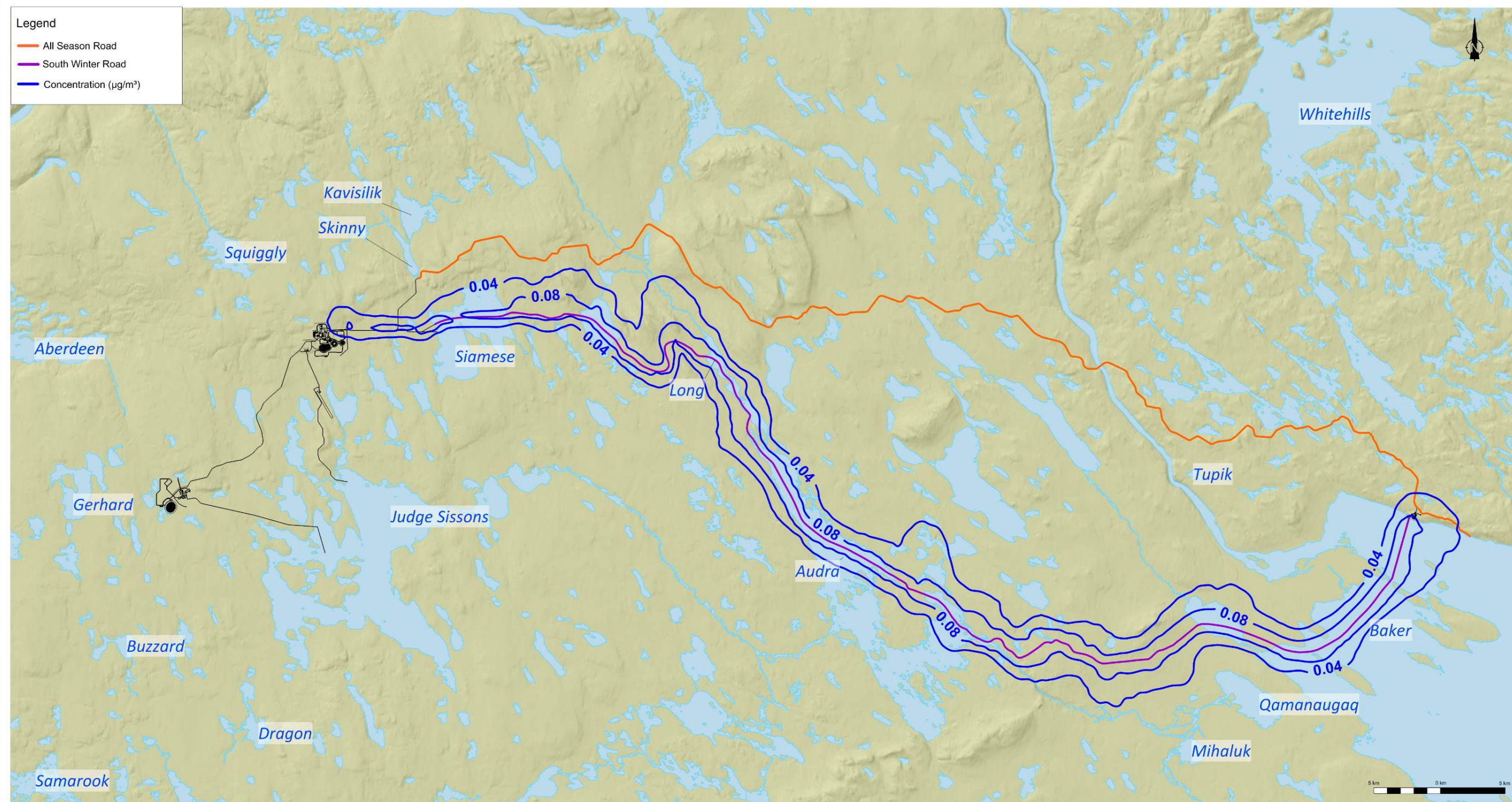
FIGURE D-149 Winter Road Option Assessment 24-hour \text{NO}_2 Concentration ( \mu\text{g}/\text{m}^3 )
