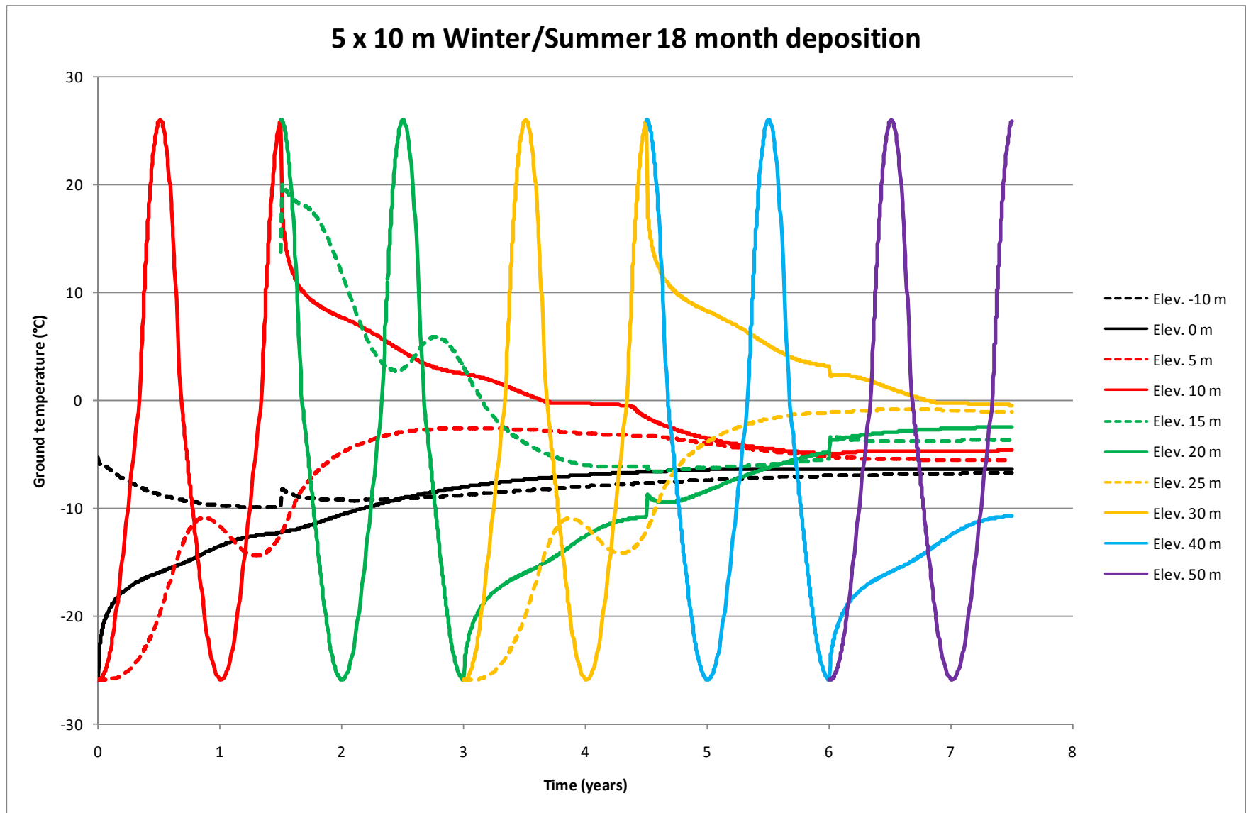
Figure 8: 5 lifts of 10m, winter/summer 18 month deposition - 0 to 8 years
