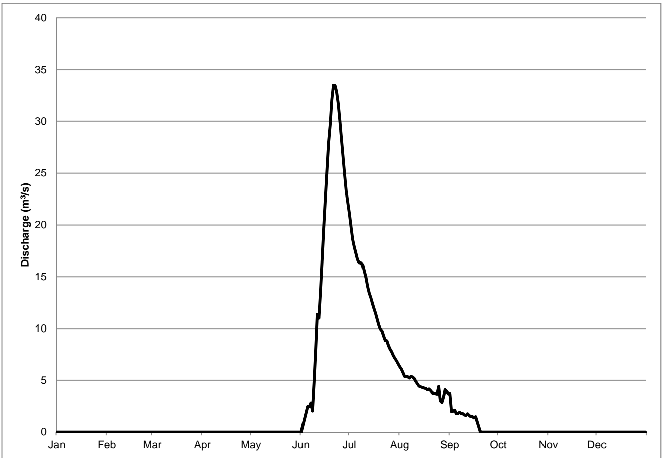
Figure 2.2-1 Estimated mean annual hydrograph for Judge Sissons Outflow
