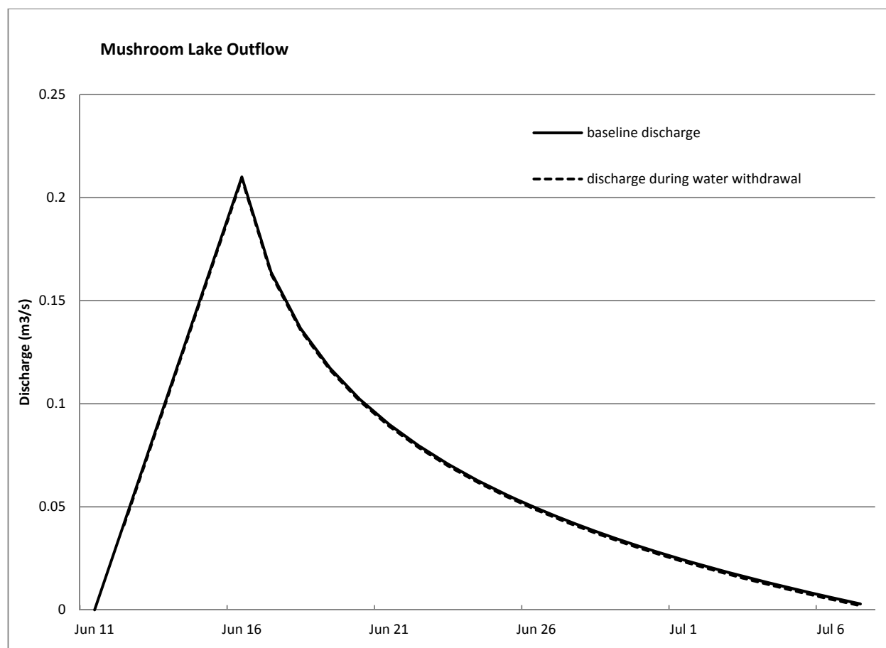
Figure 3.5-2 Mushroom Lake Outflow during summer water withdrawal
