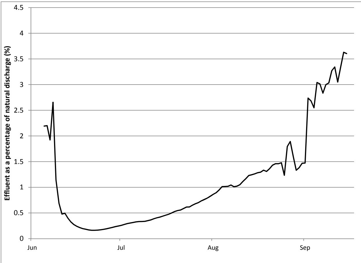
Figure 2.3-1 Effluent as a percentage of natural discharge under normal and maximum discharge conditions.
