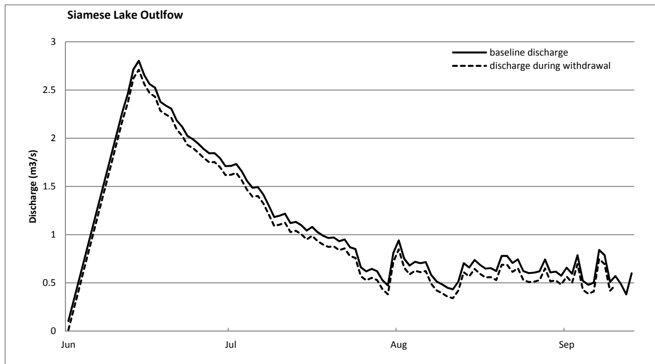
Figure 3.5-1 Siamese Lake Outflow during summer water withdrawal
