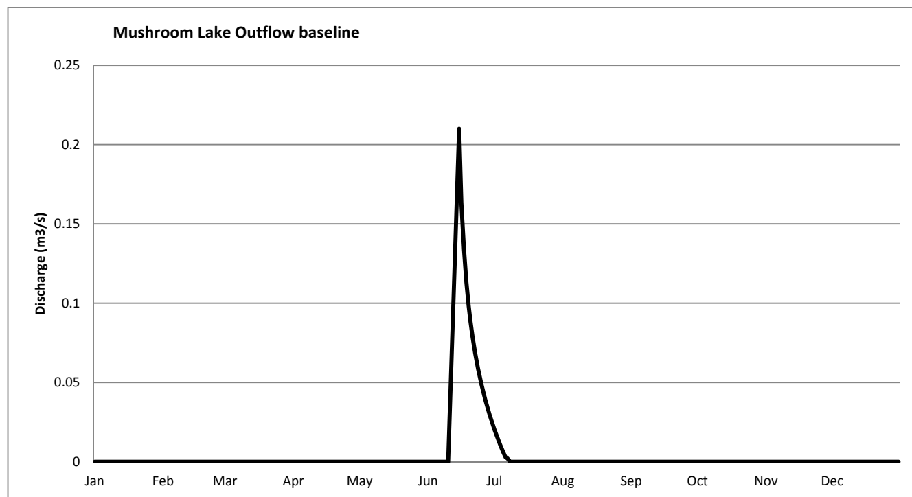
Figure 3.2-2 Mushroom Lake Outflow baseline discharge
