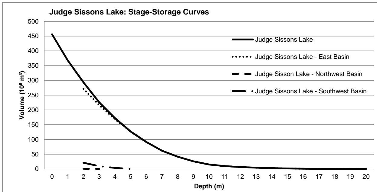
Figure 2.2-2 Judge Sissons Lake East Basin stage-storage volume curve
