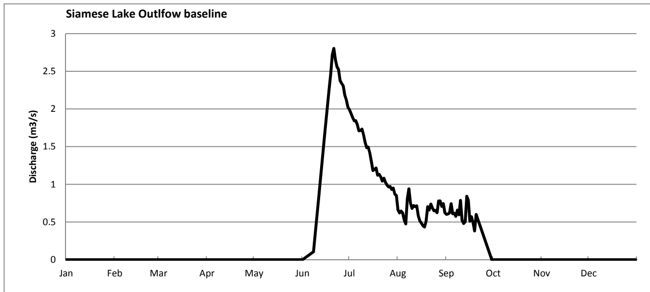
Figure 3.2-1 Siamese Lake Outflow baseline discharge
