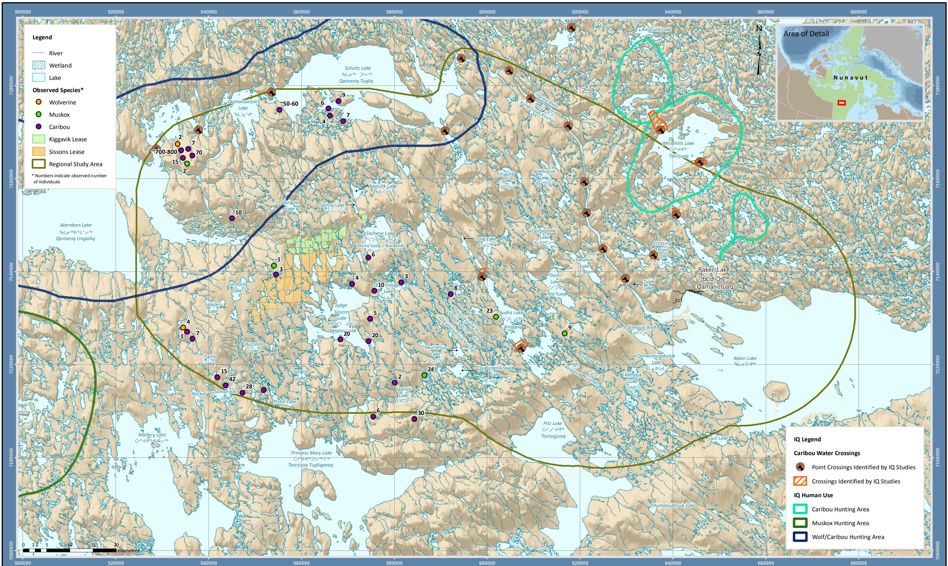
FIGURE 5.1-2 AERIAL RECONNAISSANCE SURVEY RESULTS IN THE REGIONAL STUDY AREA (NOVEMBER 2009)
