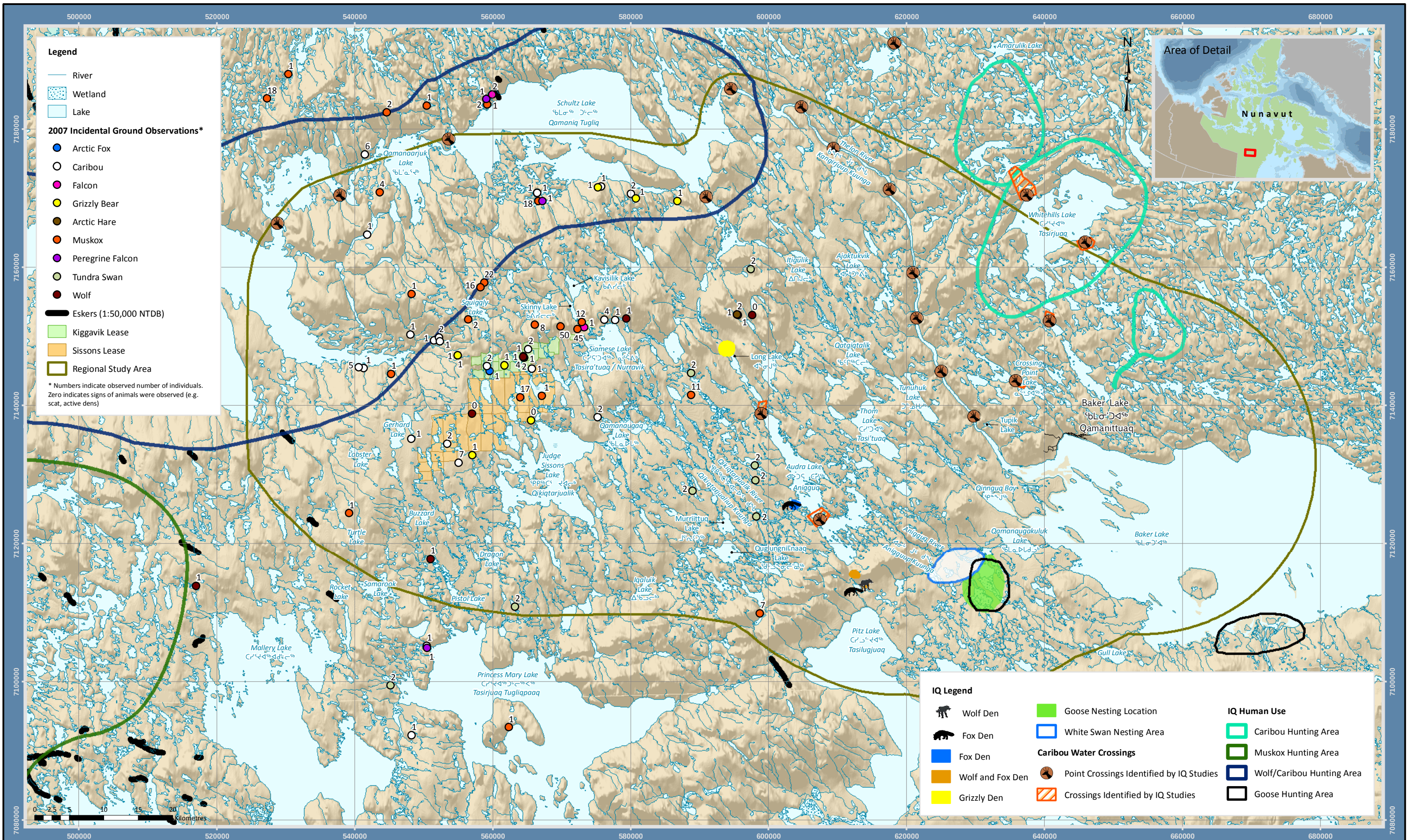
FIGURE 5.1-3 INCIDENTAL GROUND OBSERVATIONS FOR THE REGIONAL STUDY AREA (2007)
