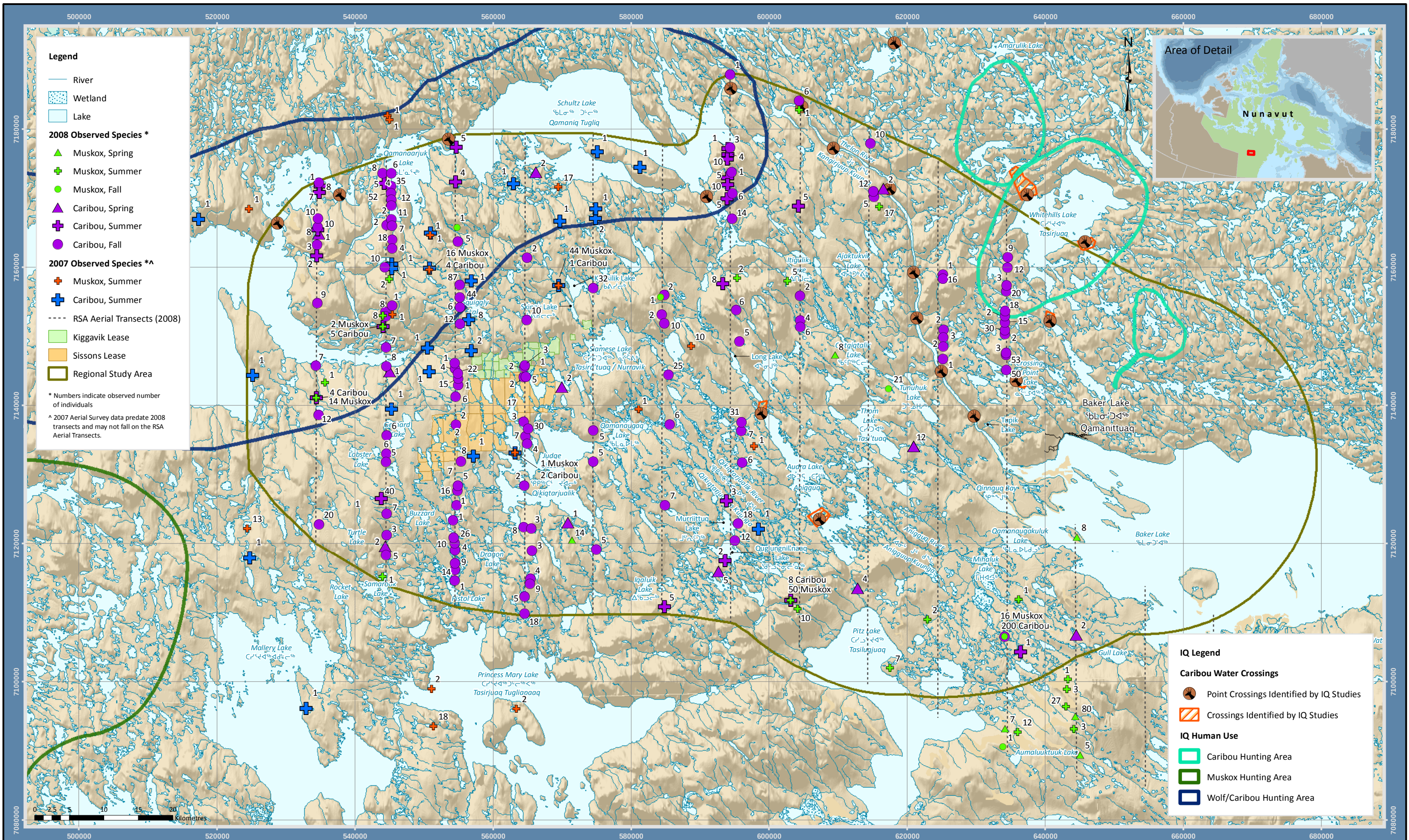
FIGURE 5.1-1 G 2007 AND 2008 AERIAL SURVEY RESULTS FOR THE REGIONAL STUDY AREA - CARIBOU AND MUSKOX
