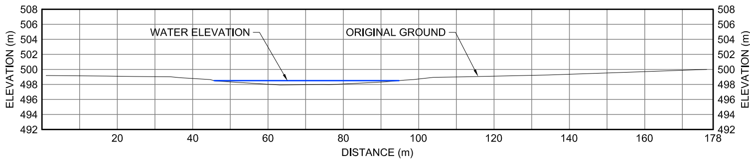
20DS XII-13 CROSS-SECTION
