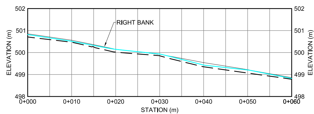
KM 140.0 STREAM PROFILE - RIGHT BANK
