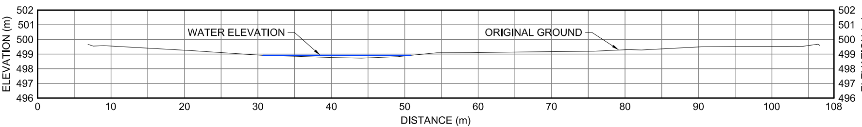
20US XII-4 CROSS-SECTION
