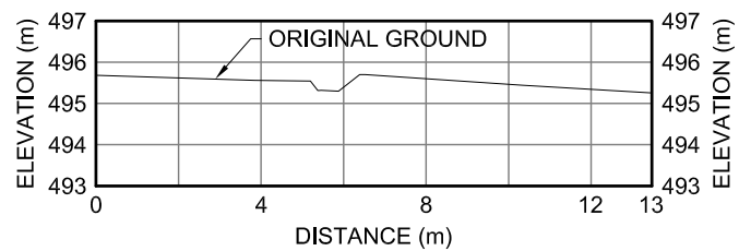
LC-4 XII-22 CROSS-SECTION
