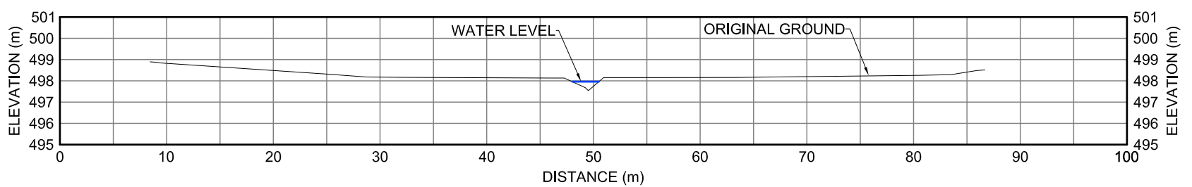
30US XII-25 CROSS-SECTION
