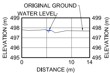
RC-1 XII-19 CROSS-SECTION
