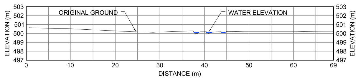
10DS XII-7 CROSS-SECTION
