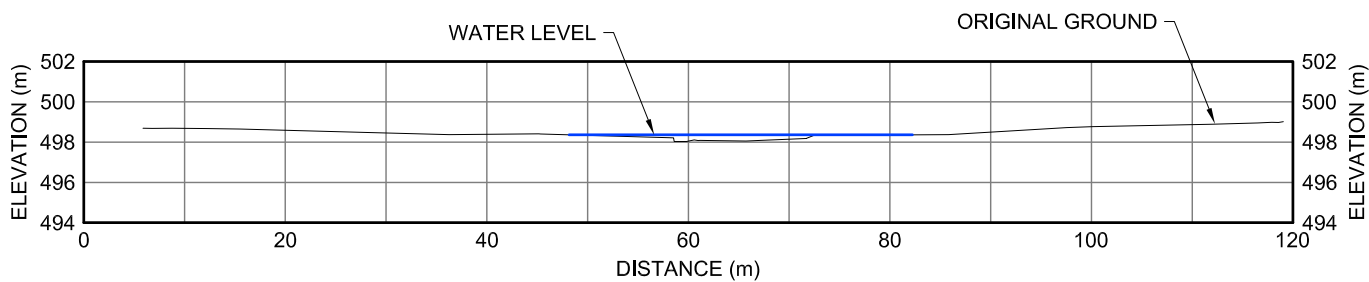
20DS XII-30 CROSS-SECTION
