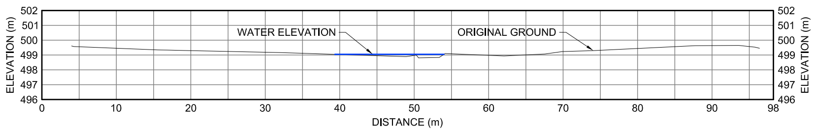
10DS XII-4 CROSS-SECTION
