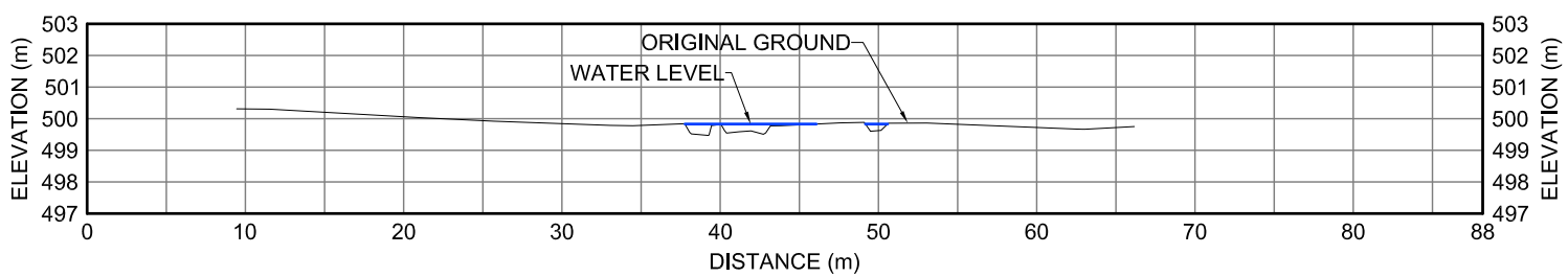
0 XII-28 CROSS SECTION
