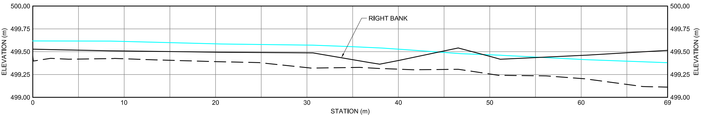
KM 195.1 STREAM PROFILE - RIGHT BANK
