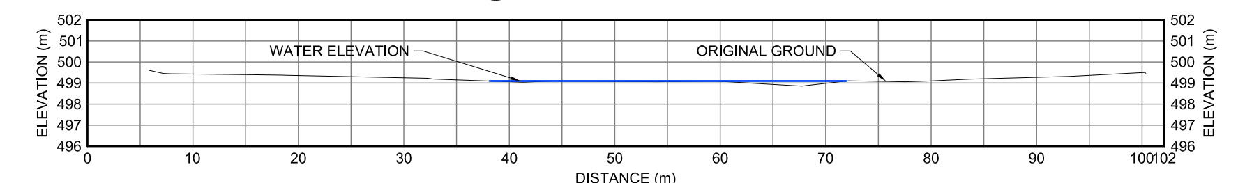
0 XII-4 CROSS-SECTION
