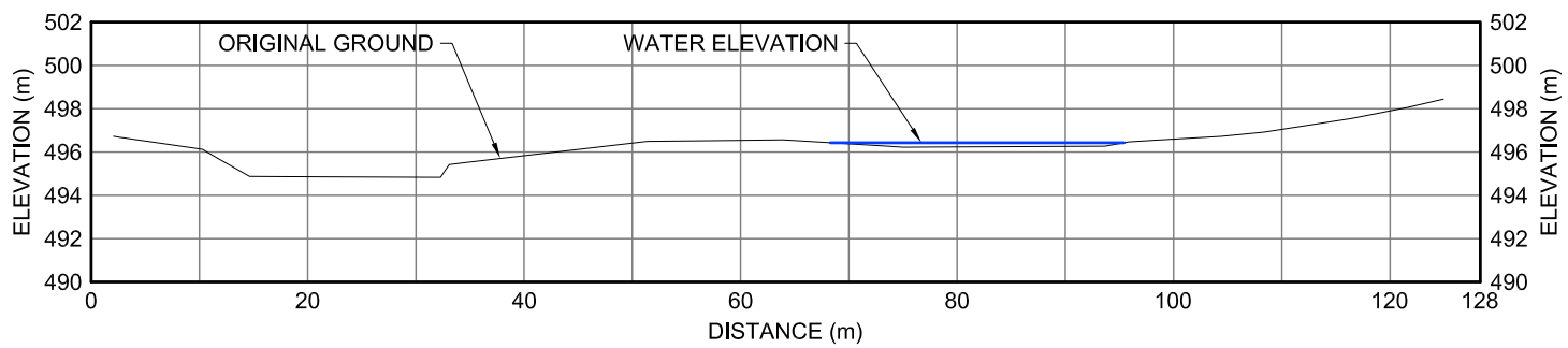
10DS XII-20 CROSS-SECTION
