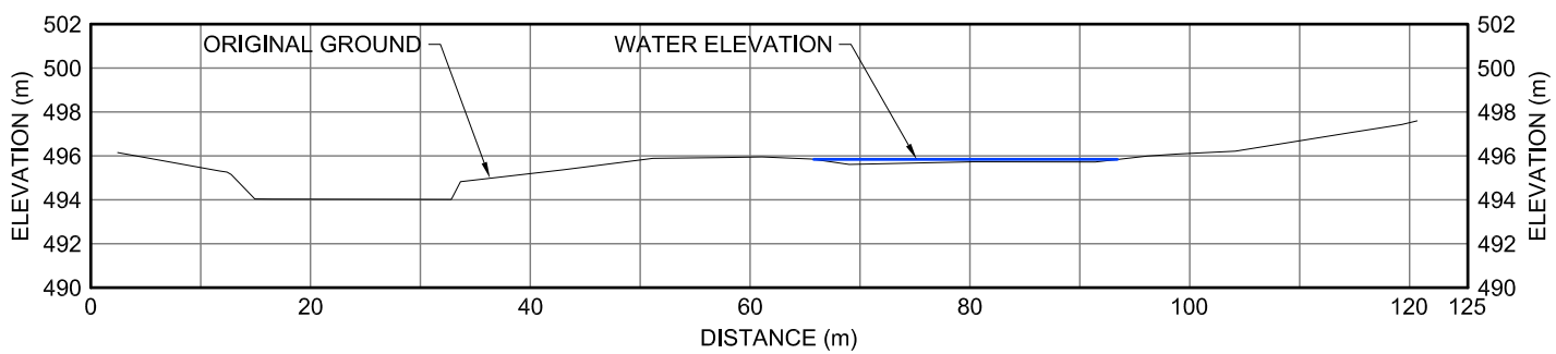
30DS XII-20 CROSS-SECTION
