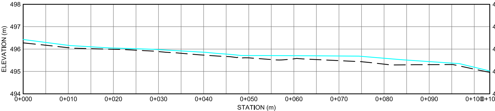
KM 108.8 STREAM PROFILE - CENTERLINE
