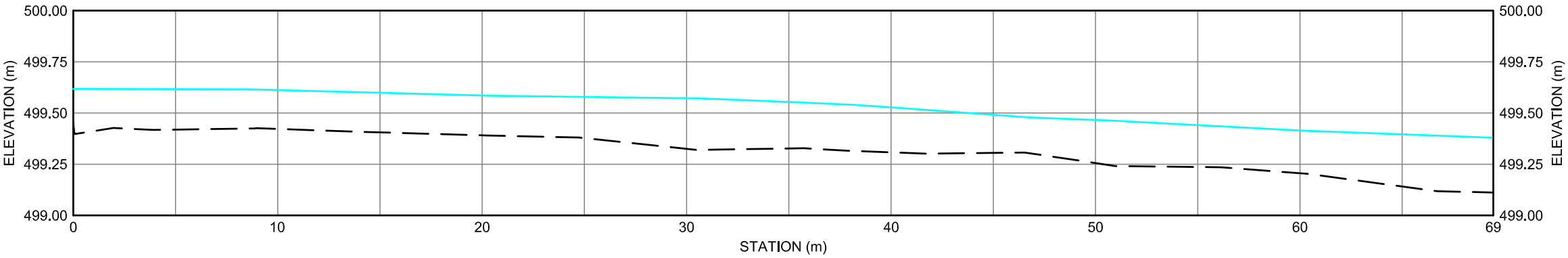
KM 195.1 STREAM PROFILE - CENTERLINE
