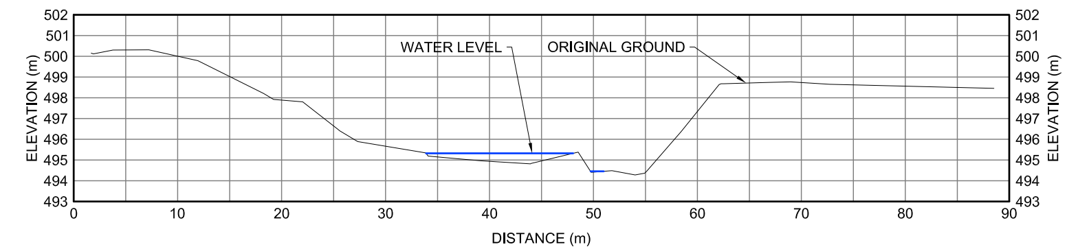
0 XII-1 CROSS-SECTION
