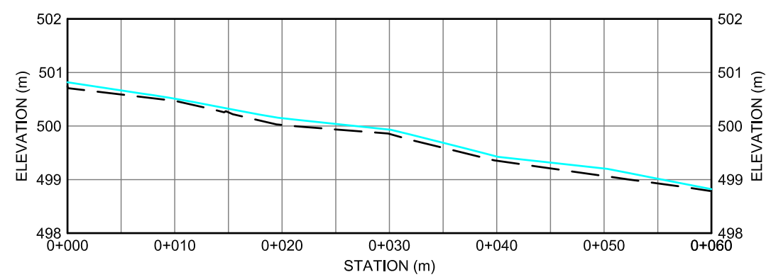
KM 140.0 STREAM PROFILE - CENTERLINE
