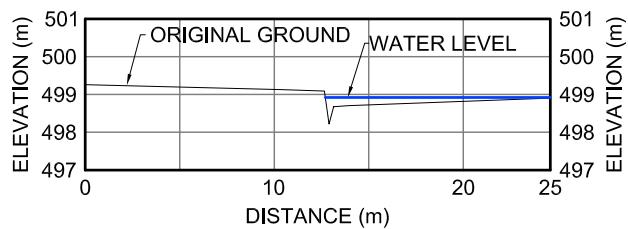
RC-6 XII-19 CROSS-SECTION
