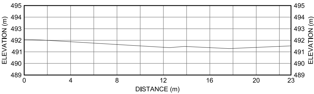
30US XII-22 CROSS-SECTION
