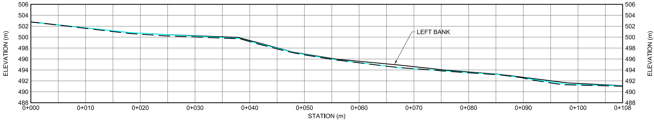
KM 212.2 WEST STREAM PROFILE - LEFT BANK
