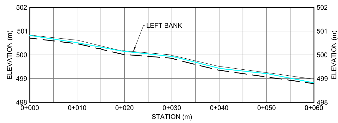
KM 140.0 STREAM PROFILE - LEFT BANK
