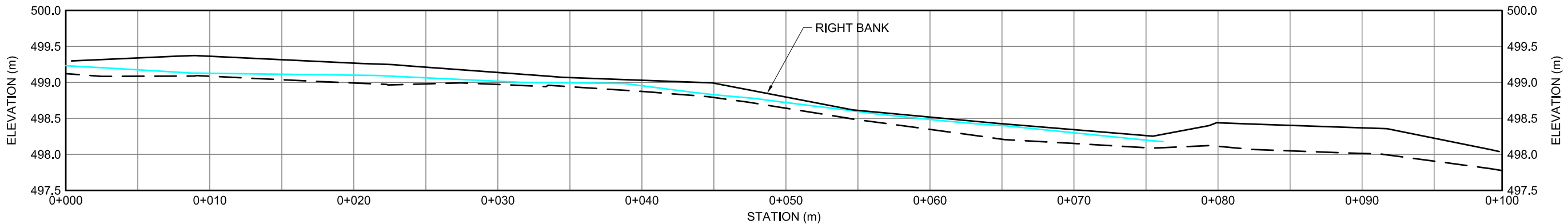
ALTERNATE EC22 STREAM PROFILE - RIGHT BANK
