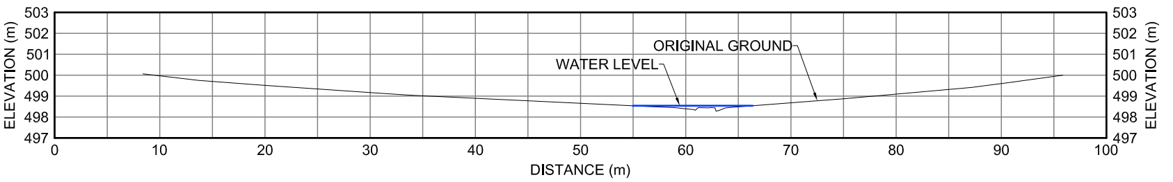
30DS XII-25 CROSS-SECTION
