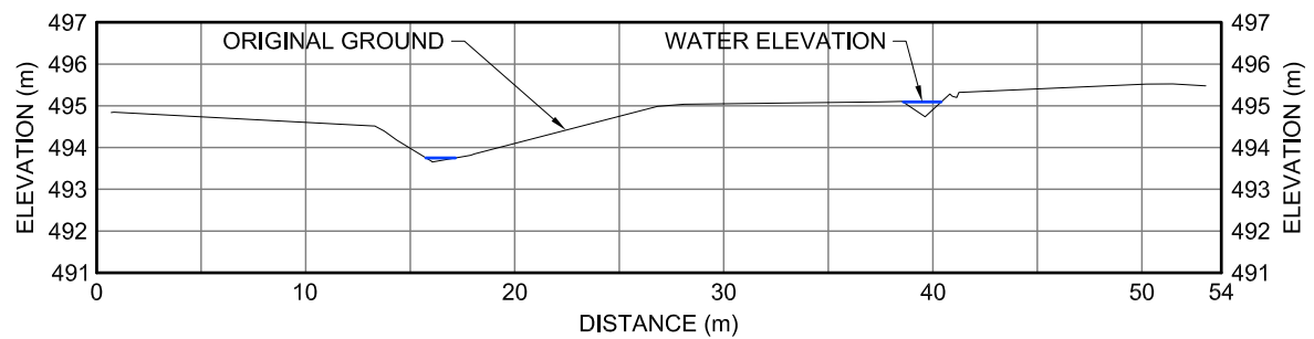
10DS XII-2 CROSS-SECTION
