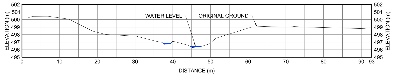
20US XII-1 CROSS-SECTION
