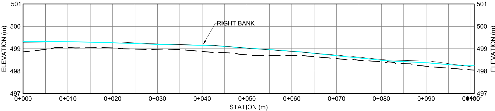
KM 147.1 STREAM PROFILE - RIGHT BANK
