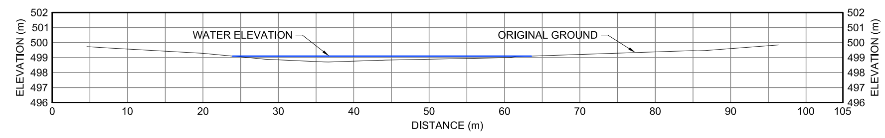
50US XII-4 CROSS-SECTION
