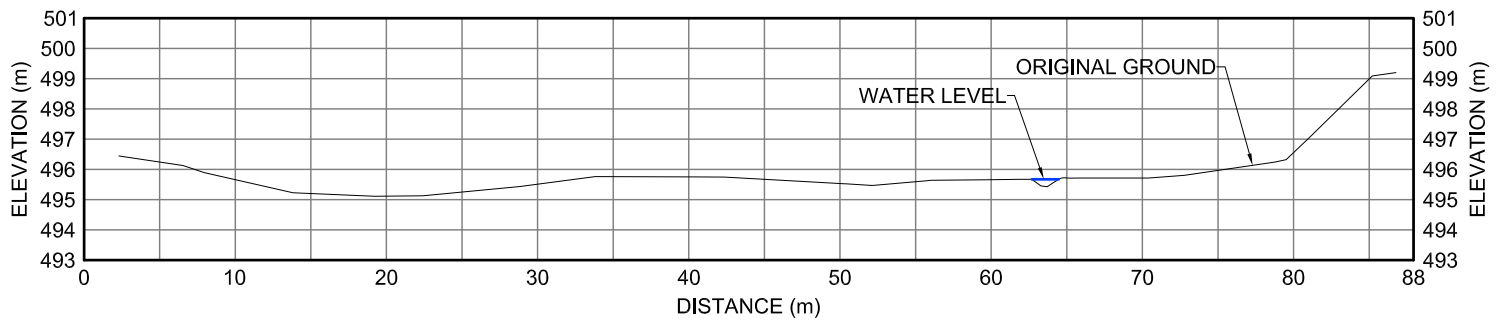
20DS XII-24 CROSS-SECTION
