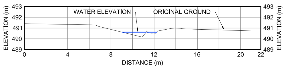
10DS XII-22 CROSS-SECTION
