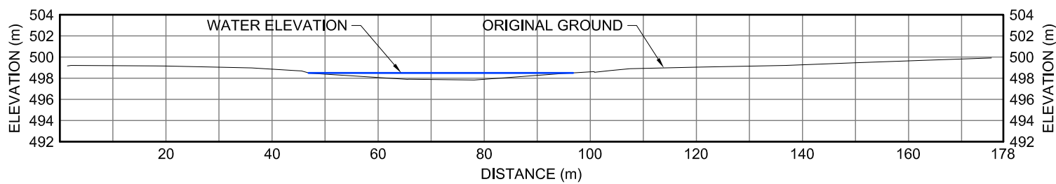
30DS XII-13 CROSS-SECTION
