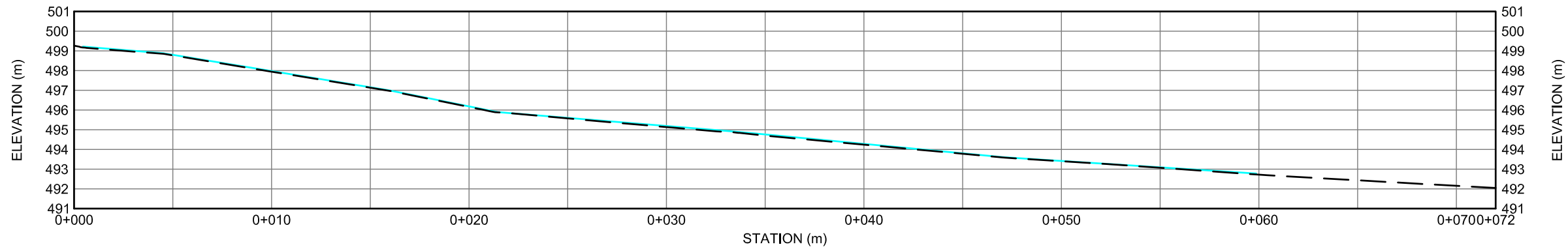
KM 212.2 EAST STREAM PROFILE - CENTERLINE
