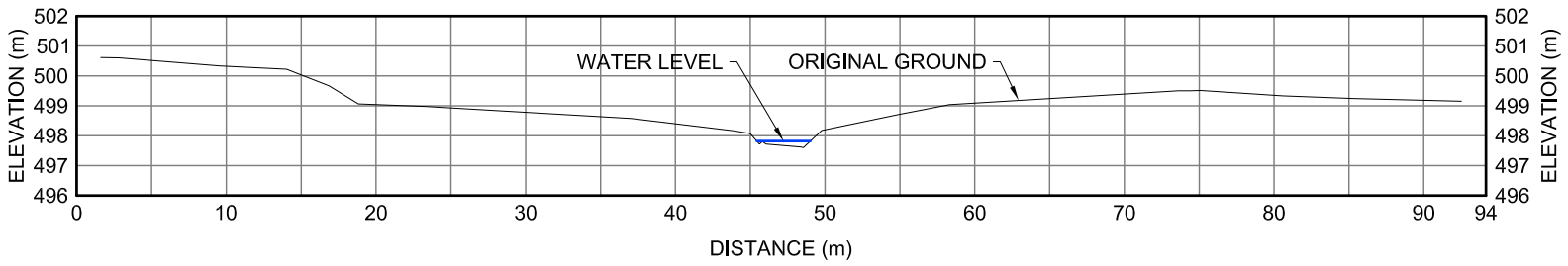
40US XII-1 CROSS-SECTION
