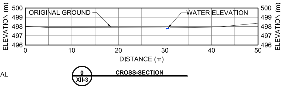
FIGURE XII-41 KM 209.4 CROSS-SECTIONS
