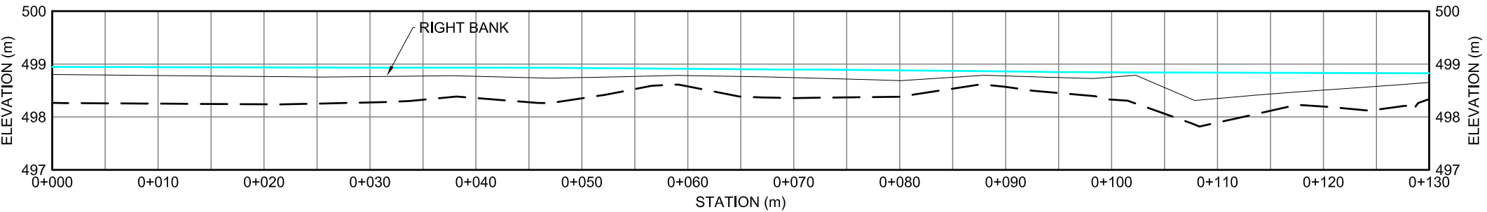
KM 145.3 STREAM PROFILE - RIGHT BANK
