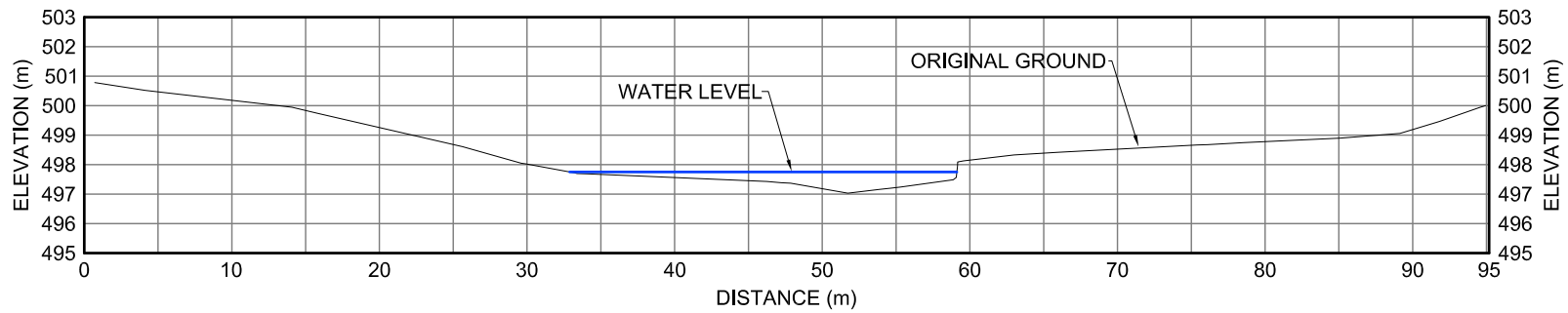
10DS XII-17 CROSS-SECTION
