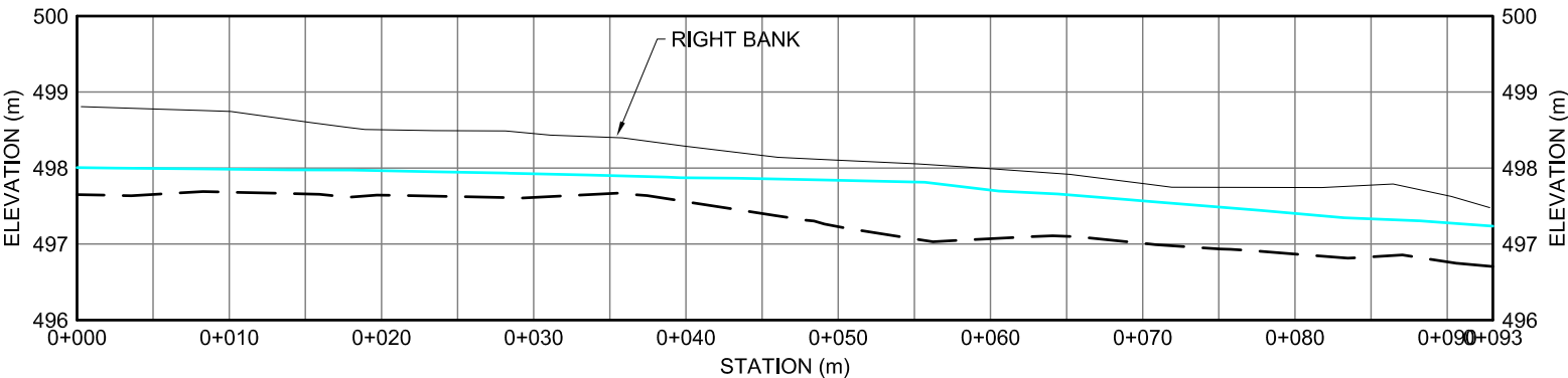
KM 129.2 STREAM PROFILE - RIGHT BANK
