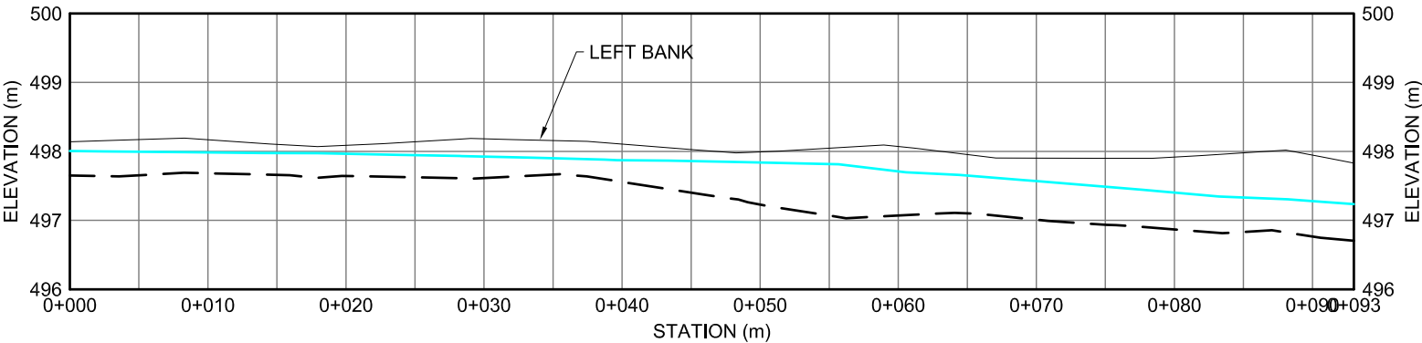
KM 129.2 STREAM PROFILE - LEFT BANK
