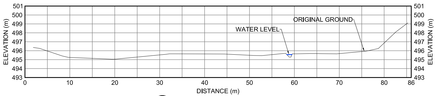
30DS XII-24 CROSS-SECTION
