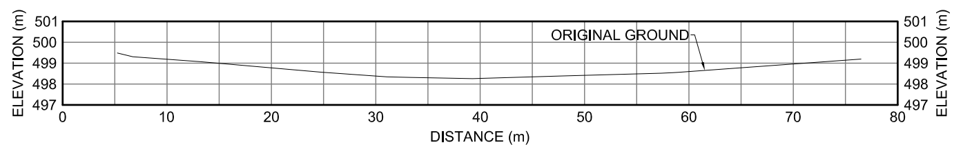
20US XII-26 CROSS-SECTION
