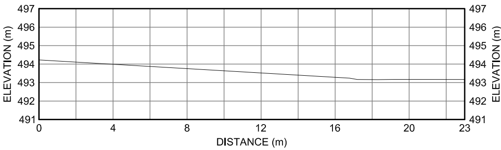
50US XII-22 CROSS-SECTION
