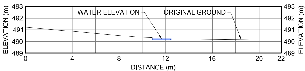
30DS XII-22 CROSS-SECTION
