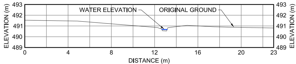
0 XII-22 CROSS-SECTION
