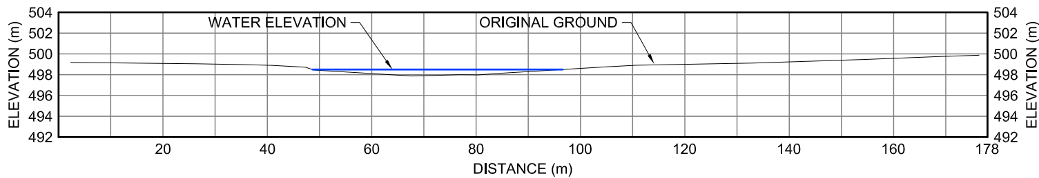
40DS XII-13 CROSS-SECTION
