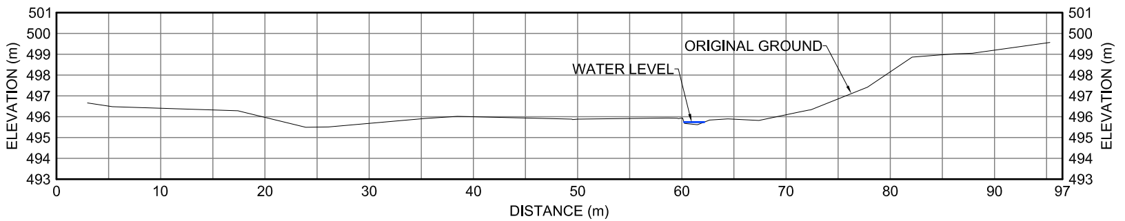
0 XII-24 CROSS-SECTION
