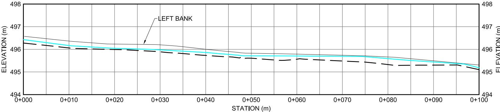
KM 108.8 STREAM PROFILE - LEFT BANK
