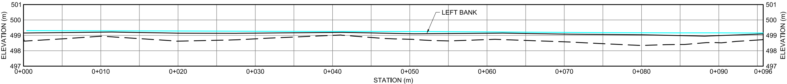
KM 2.0 STREAM PROFILE - LEFT BANK
