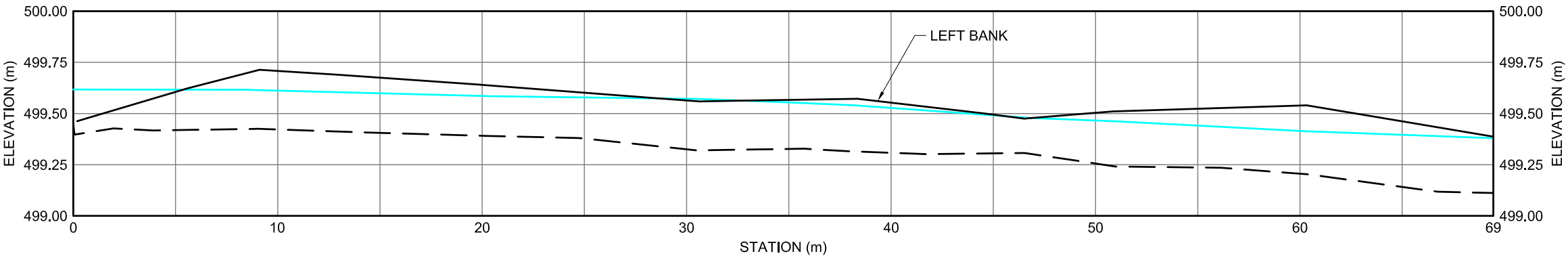
KM 195.1 STREAM PROFILE - LEFT BANK
