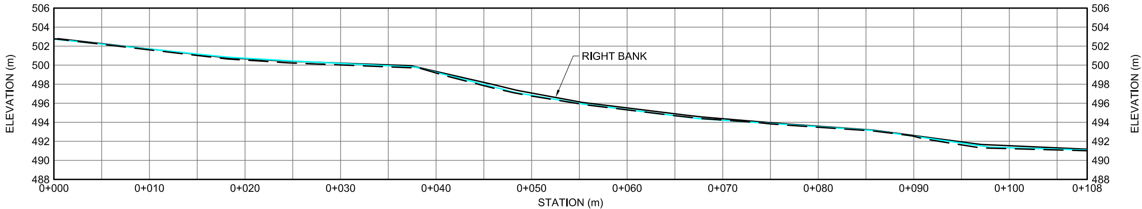
KM 212.2 WEST STREAM PROFILE - RIGHT BANK
