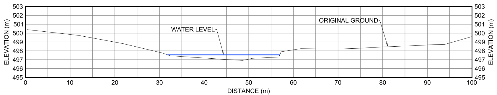
30DS XII-17 CROSS-SECTION
