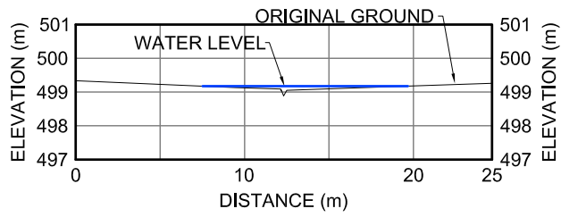
RC-7 XII-19 CROSS-SECTION
