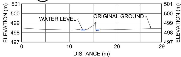
RC-3 XII-19 CROSS-SECTION
