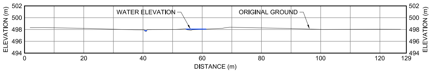
40DS XII-20 CROSS-SECTION
