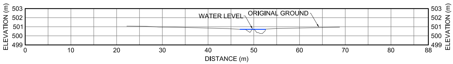
40US XII-28 CROSS SECTION
