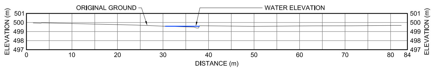
20DS XII-6 CROSS-SECTION
