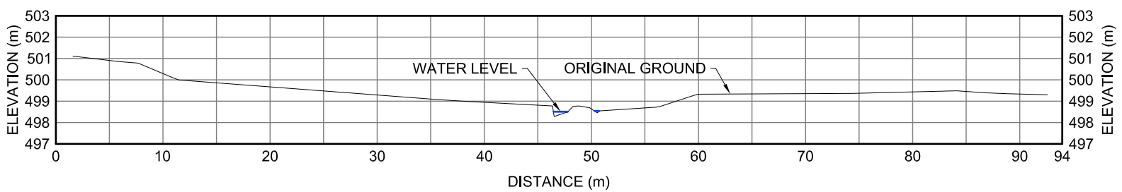
50US XII-1 CROSS-SECTION
