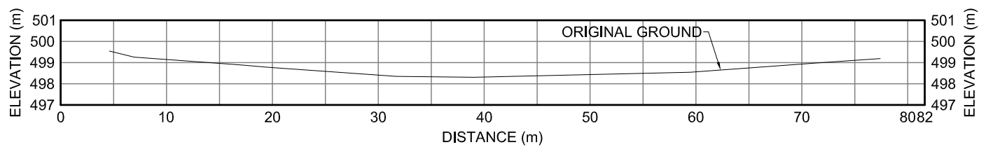
30US XII-26 CROSS-SECTION
