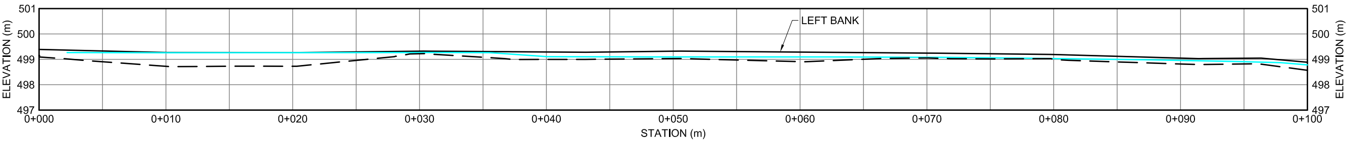
KM 6.7 STREAM PROFILE - LEFT BANK
