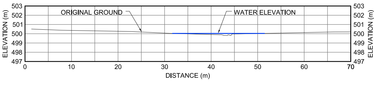
20DS XII-7 CROSS-SECTION
