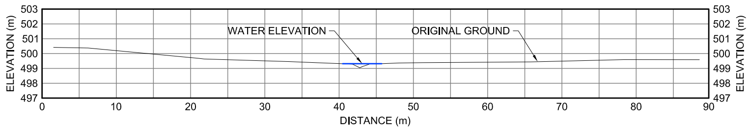
40US XII-14 CROSS-SECTION
