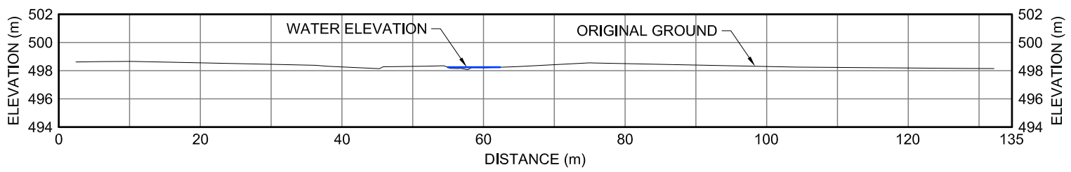
30DS XII-20 CROSS-SECTION
