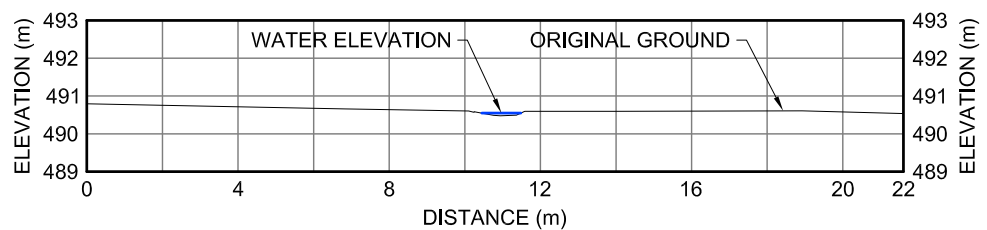
20DS XII-22 CROSS-SECTION
