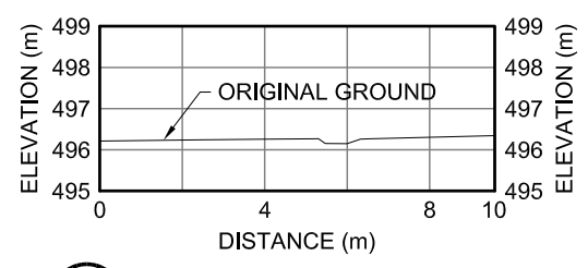
LC-2 XII-22 CROSS-SECTION
