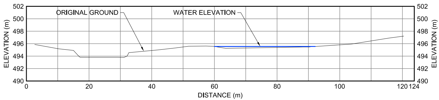
40DS XII-20 CROSS-SECTION
