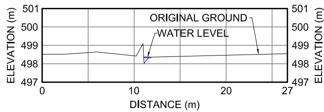
RC-4 XII-19 CROSS-SECTION
