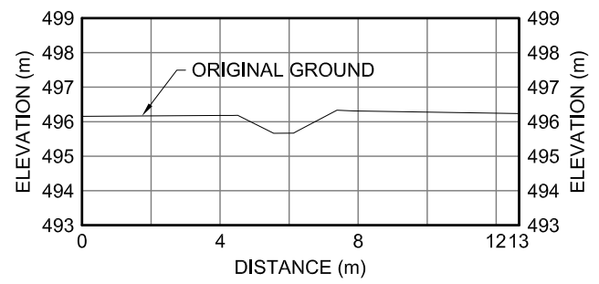
RC-1 XII-22 CROSS-SECTION
