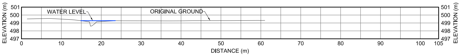
40US XII-32 CROSS-SECTION
