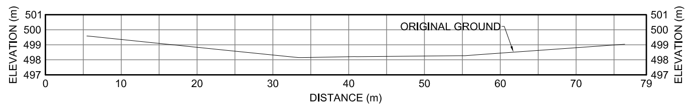
50US XII-2 CROSS SECTION
