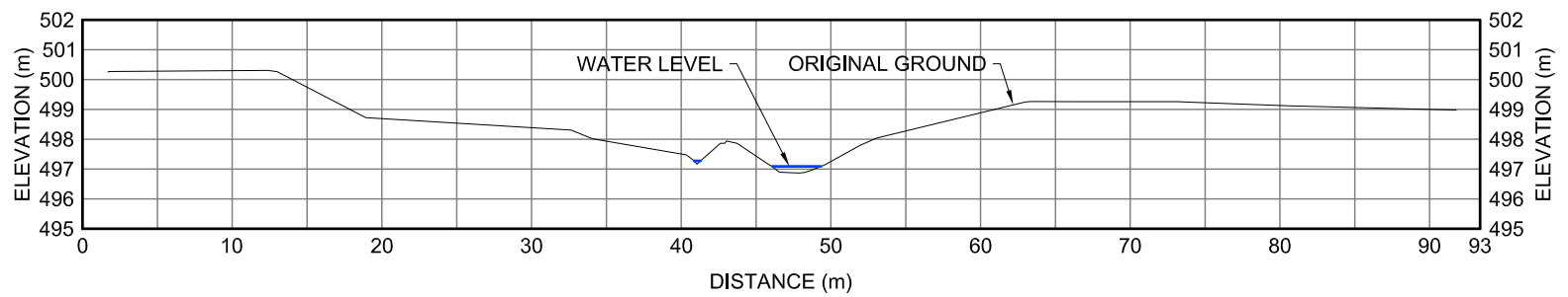
30US XII-1 CROSS-SECTION
