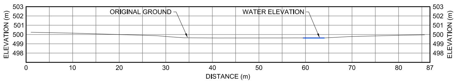
0 XII-21 CROSS-SECTION
