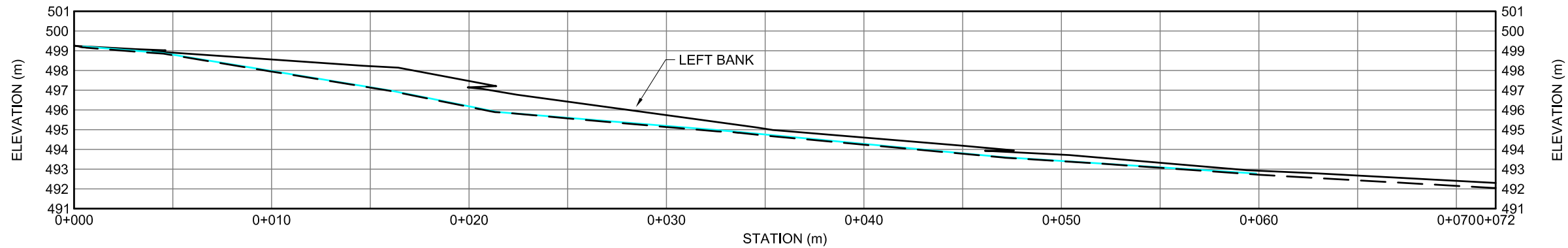
KM 212.2 EAST STREAM PROFILE - LEFT BANK
