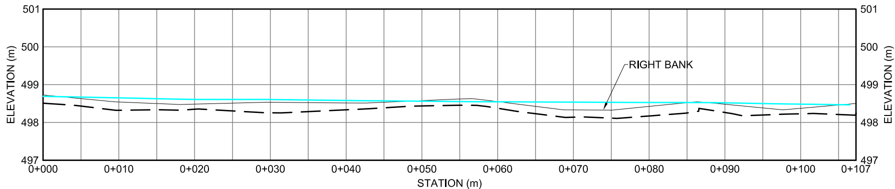
KM 127.5 STREAM PROFILE - RIGHT BANK
