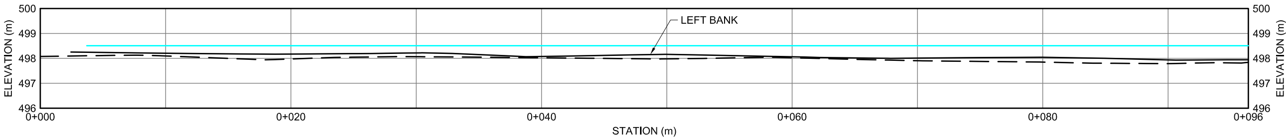
KM 11.3 STREAM PROFILE - LEFT BANK
