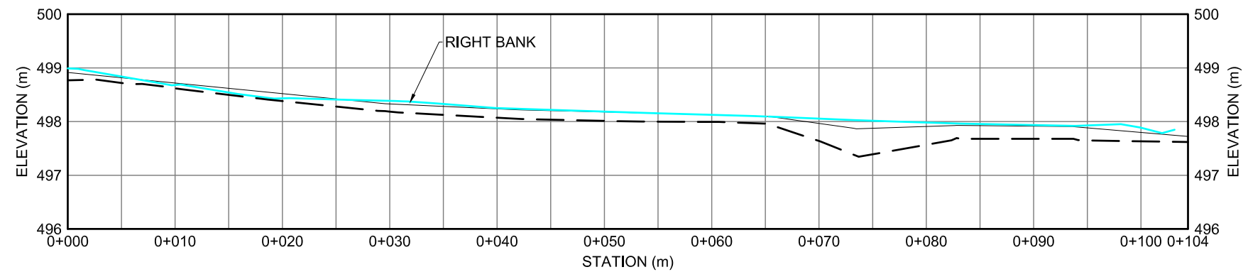
KM 107.8 STREAM PROFILE - RIGHT BANK
