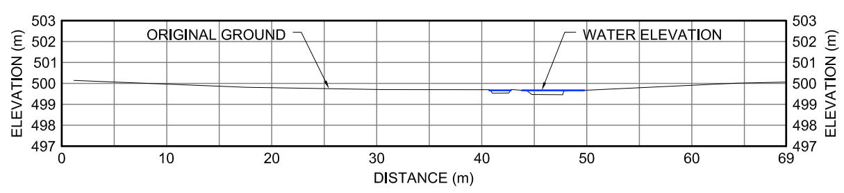
40DS XII-7 CROSS-SECTION
