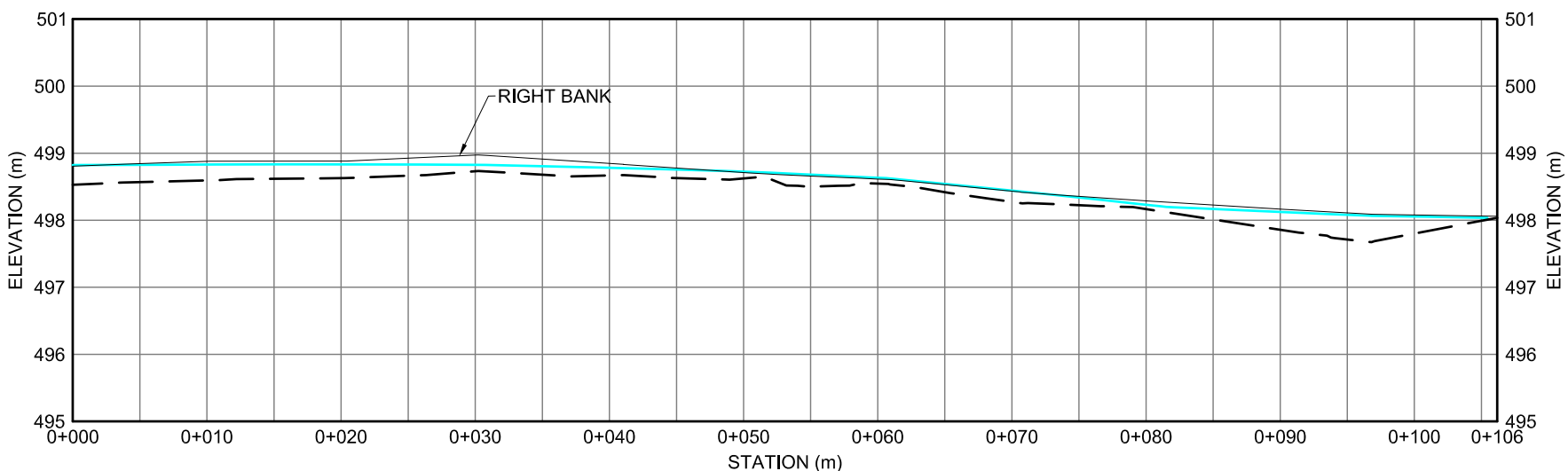
KM 157.7 STREAM PROFILE - RIGHT BANK
