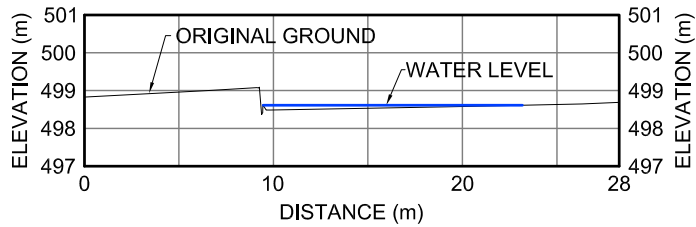
RC-5 XII-19 CROSS-SECTION
