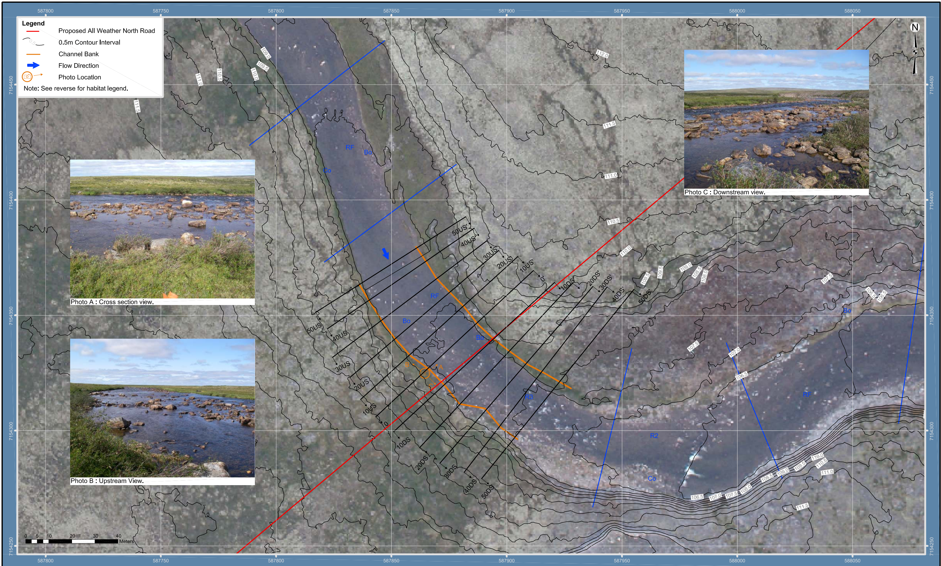
FIGURE XII-17 KM 129.2 PLAN VIEW
