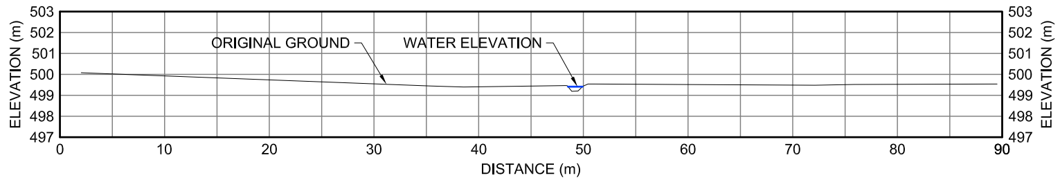
30US XII-6 CROSS-SECTION
