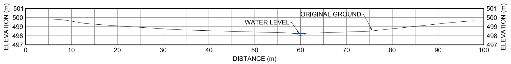
10DS XII-25 CROSS-SECTION
