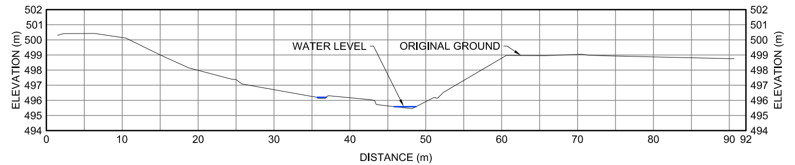
10US XII-1 CROSS-SECTION
