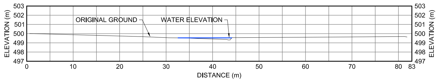
0 XII-6 CROSS-SECTION
