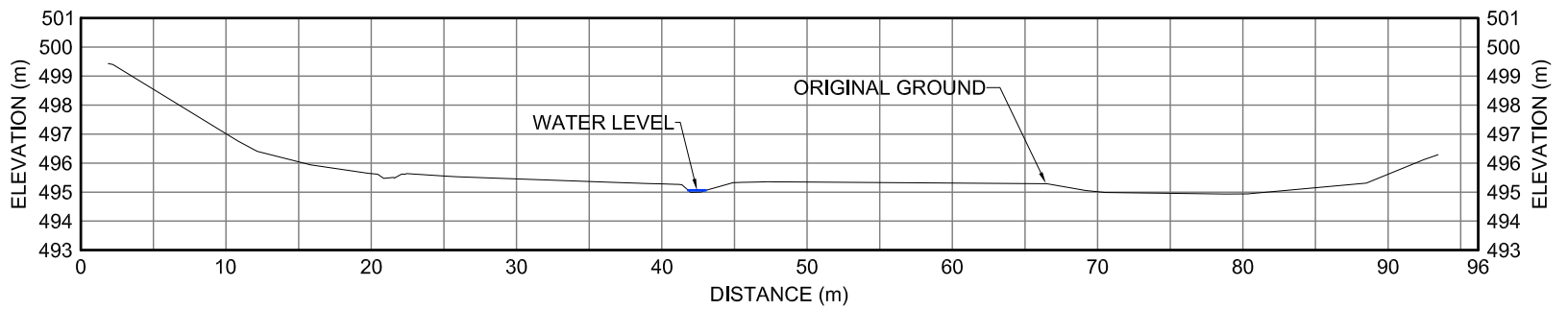
50DS XII-24 CROSS-SECTION
