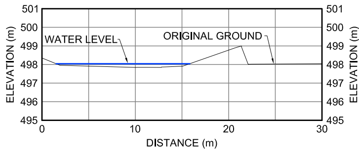
RC-2 XII-19 CROSS-SECTION
