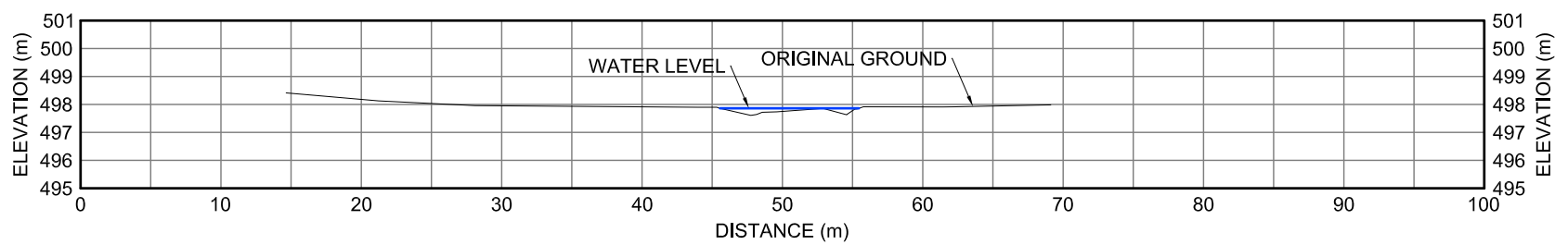
50US XII-25 CROSS-SECTION
