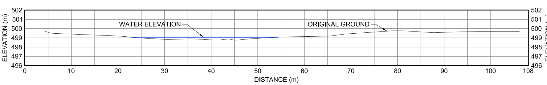
30US XII-4 CROSS-SECTION
