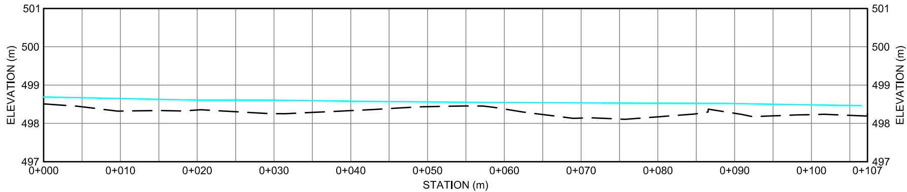
KM 127.5 STREAM PROFILE - CENTERLINE
