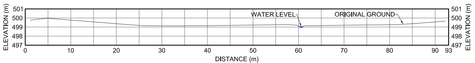
30DS XII-31 CROSS-SECTION
