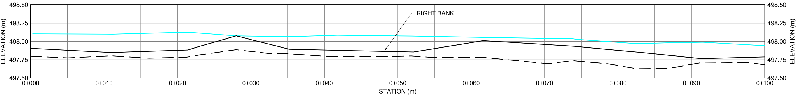
KM 197.5 STREAM PROFILE - CENTERLINE
