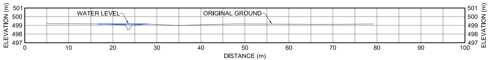
20DS XII-32 CROSS-SECTION
