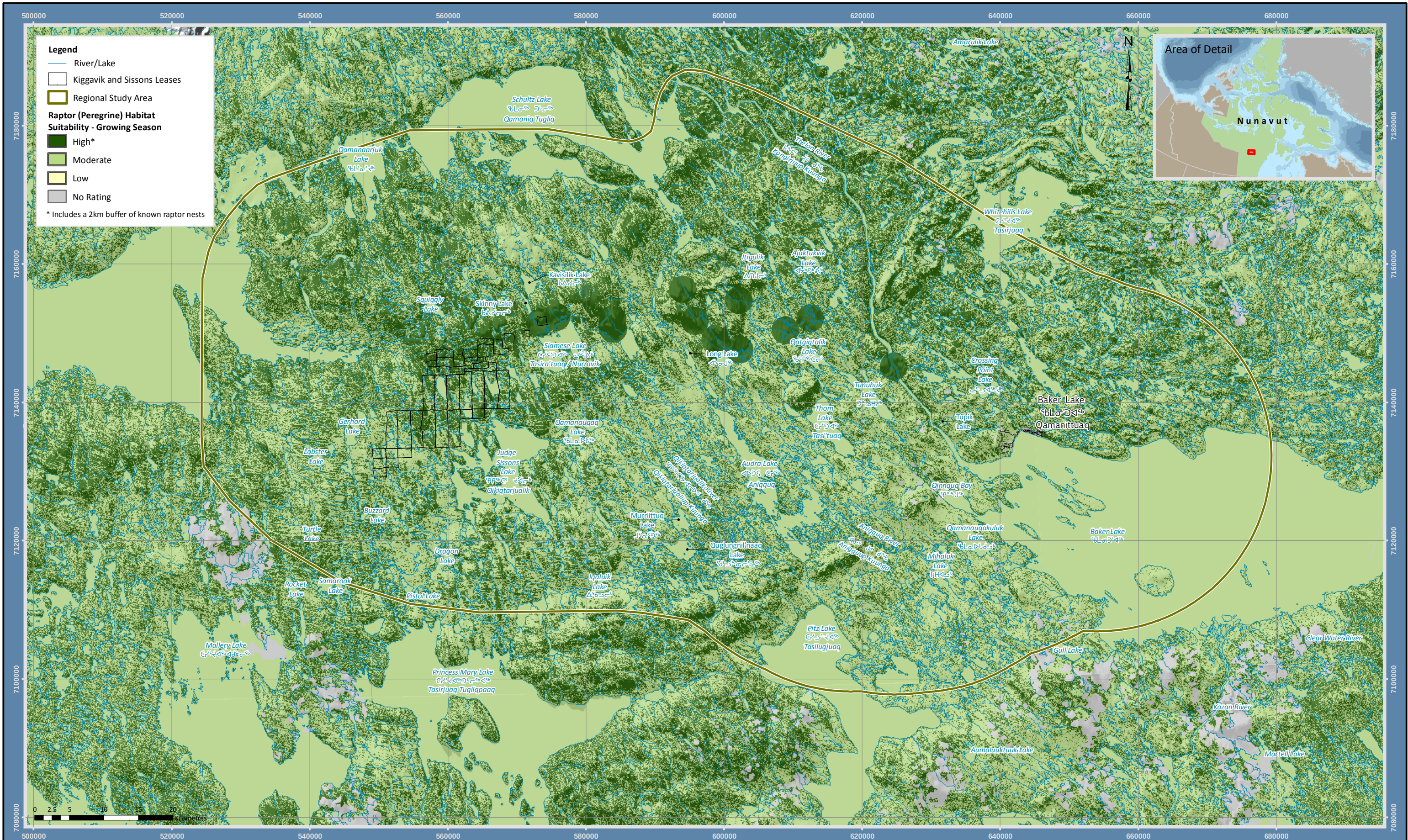
FIGURE 5.6-6 RAPTOR (PEREGRINE) HABITAT SUITABILITY - GROWING SEASON KIGGAVIK PROJECT - EIS
