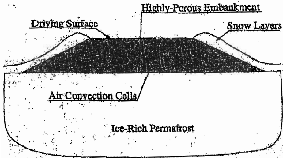
Figure 3 Pattern of air circulation in an embankment (Gaering 1998)
