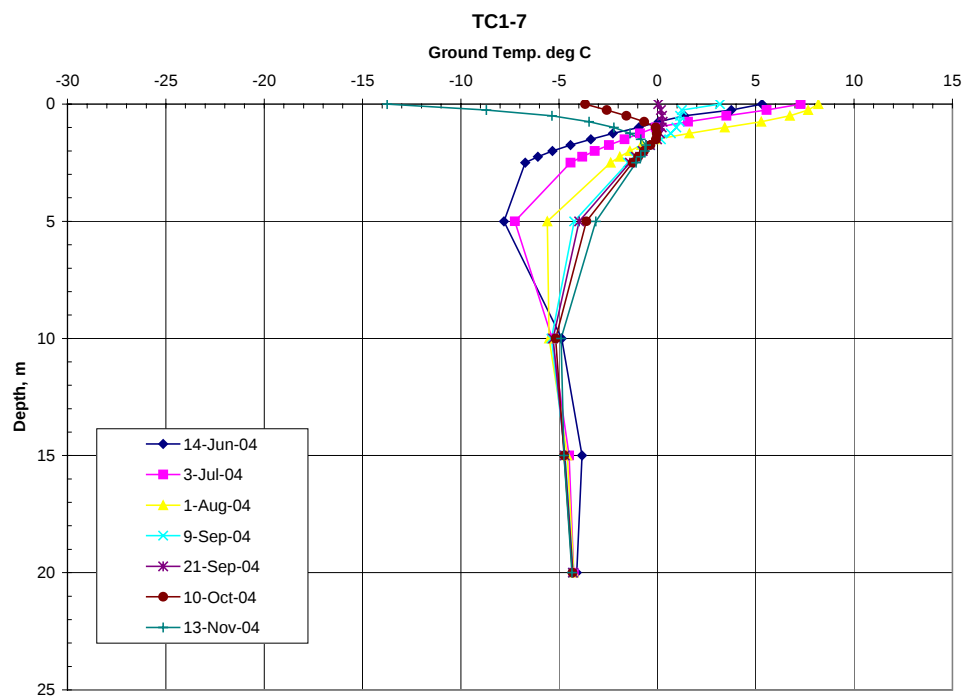
Figure C 18. Ground temperature regime in tailings Cell 1, near 3D Dam (Thermistor TC1-7)
