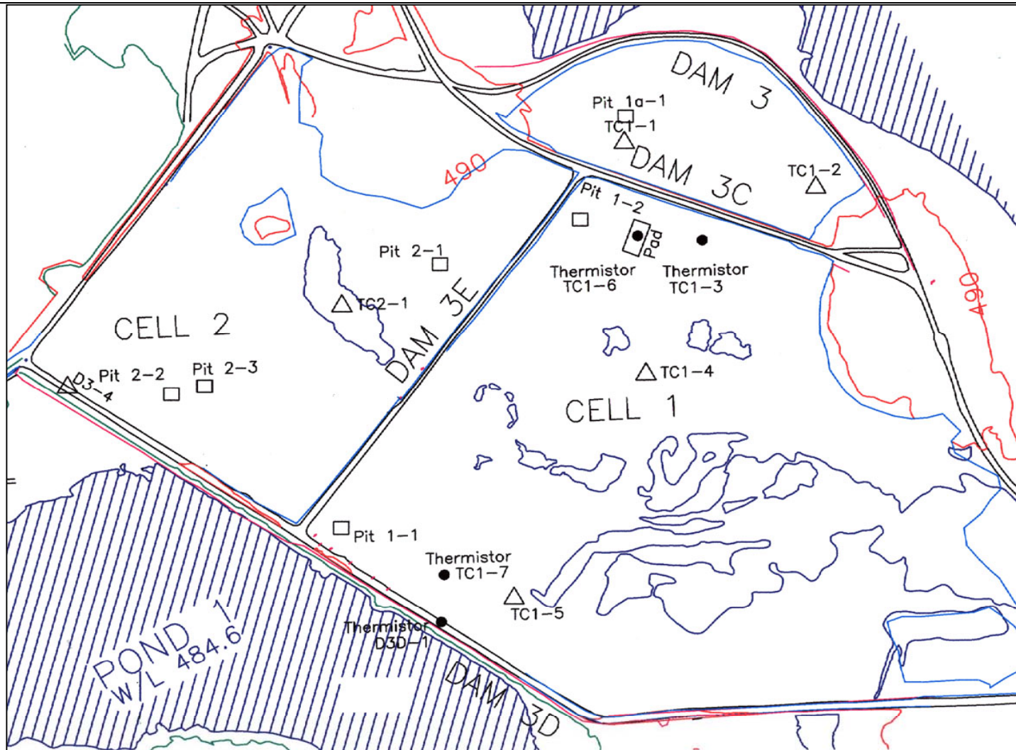
Figure C 5. Thermistors in Cell 1 and Dam 3D
