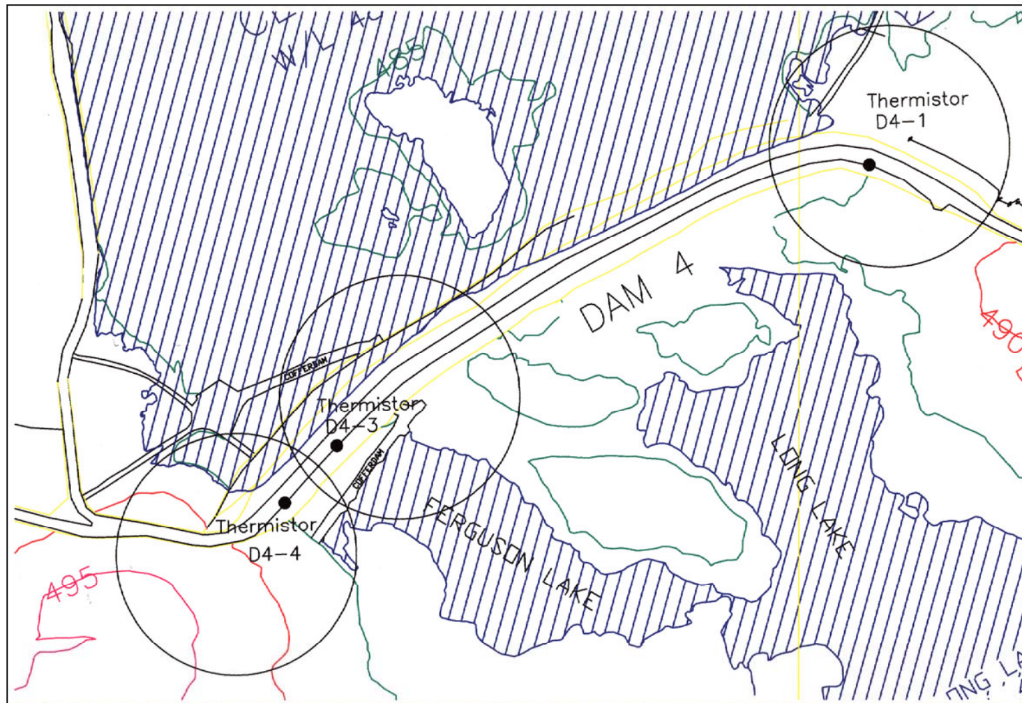
Figure C 4. Thermistors at Dam 4
