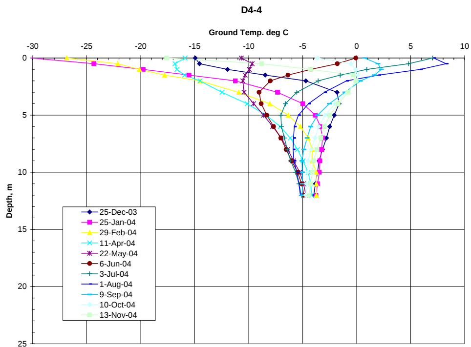
Figure C 13. Ground temperature regime at Dam 4 (Thermistor D4-4)
