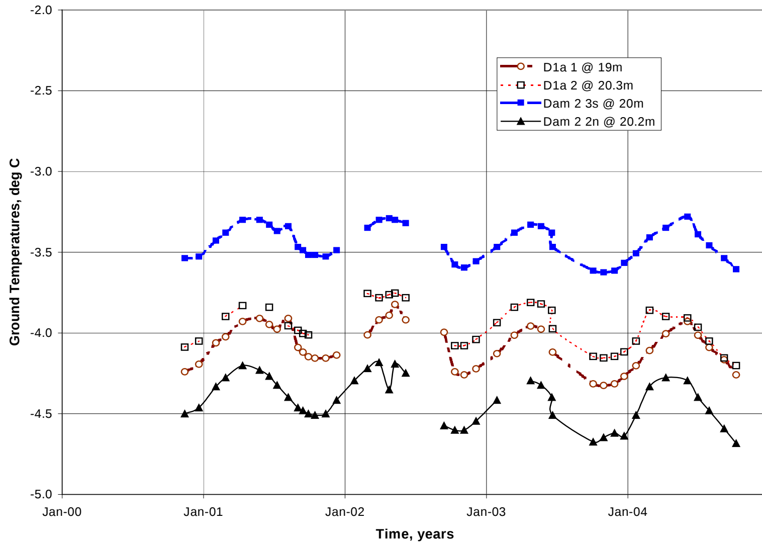
Figure C 7. Ground temperatures at 20m depth at Dams 1 and 2
