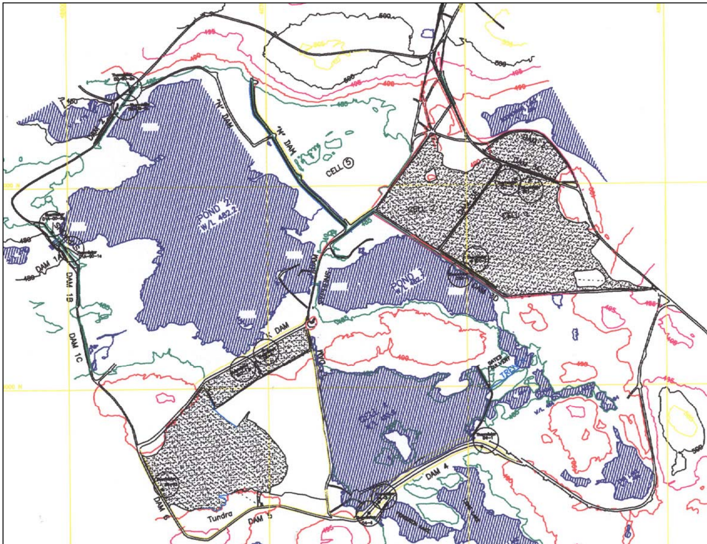
Figure C 1. General thermistor location plan
