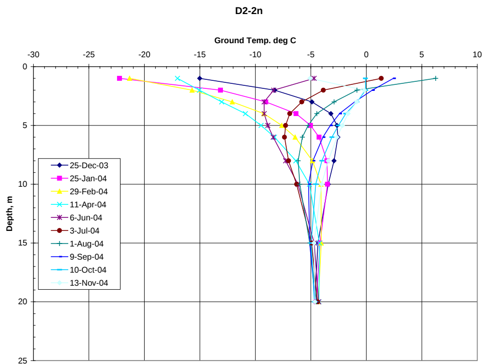
Figure C 10. Ground temperature regime at Dam 2 (Thermistor D2-00-2n)
