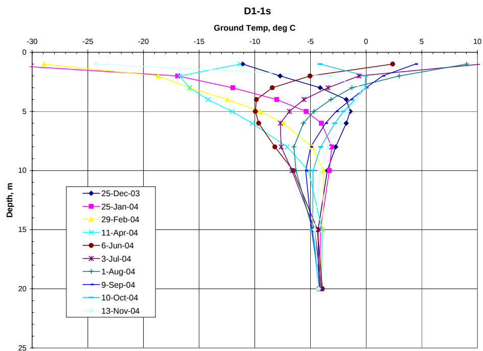
Figure C 9. Ground temperature regime at Dam 1a (Thermistor D1A-00-1s)
