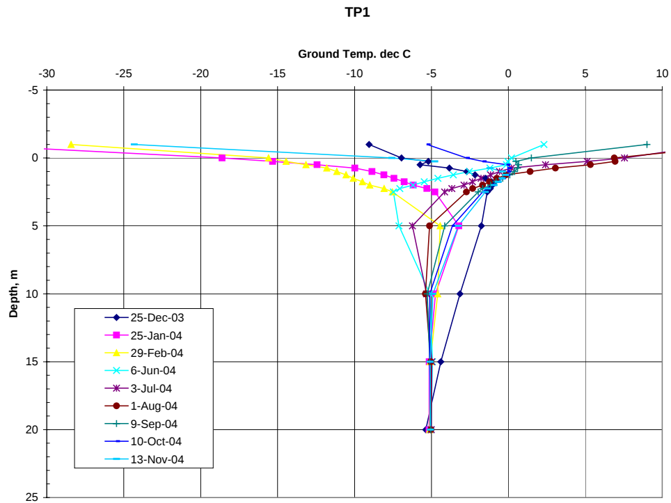
Figure C 15. Ground temperature regime at Cell 1 Test Pad (Thermistor TC1-3)
