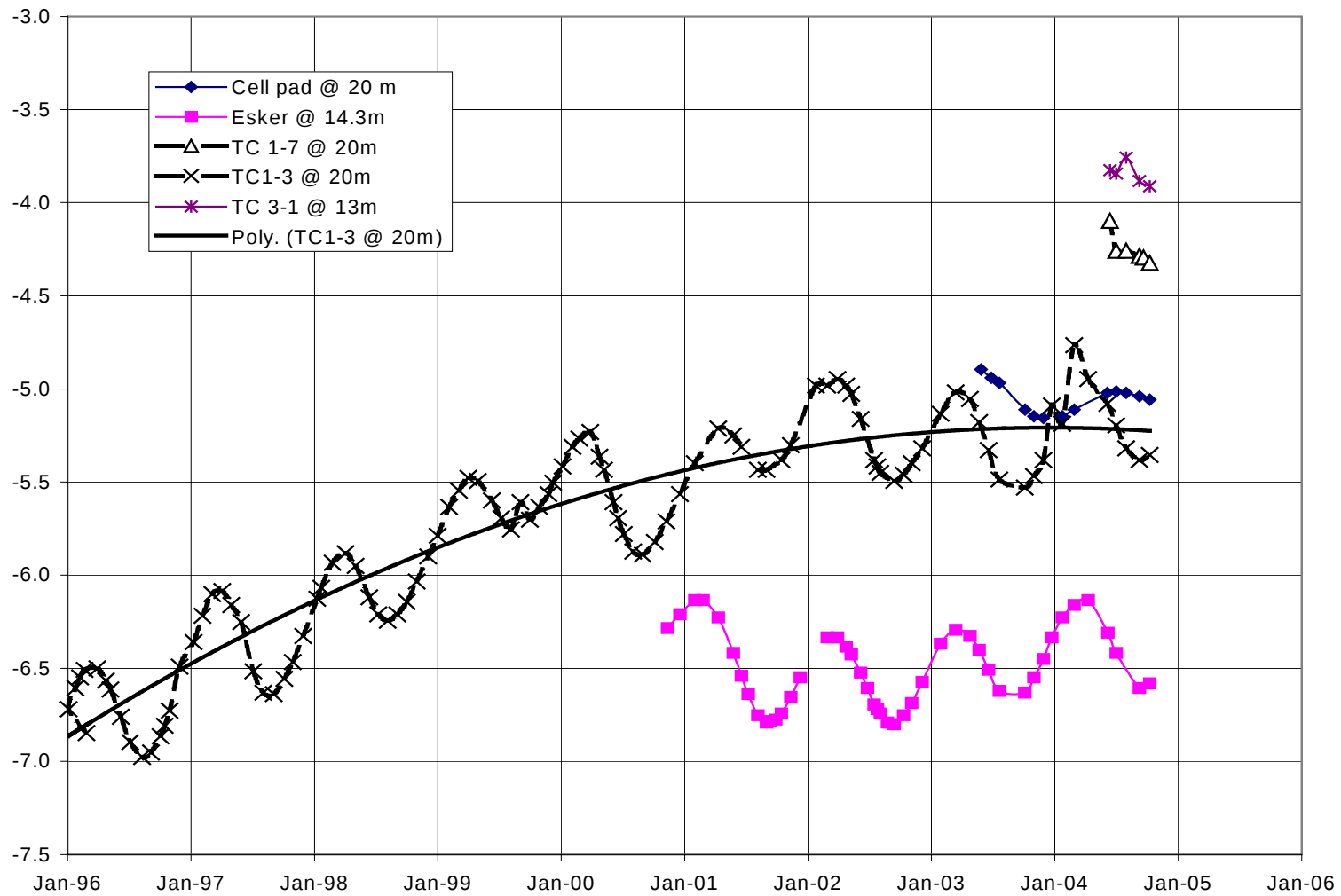
Figure C 8. Ground temperatures in Cells at 12 to 20m depth ground temperatures in Cell 1 from 1980 to 2004
