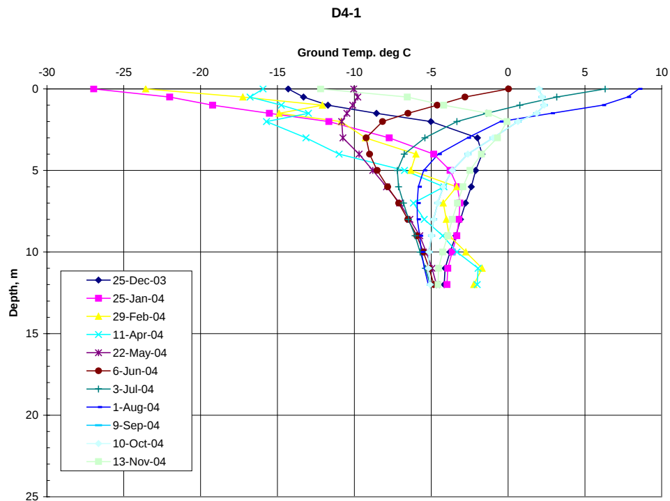
Figure C 11. Ground temperature regime at Dam 4 (Thermistor D4-1)
