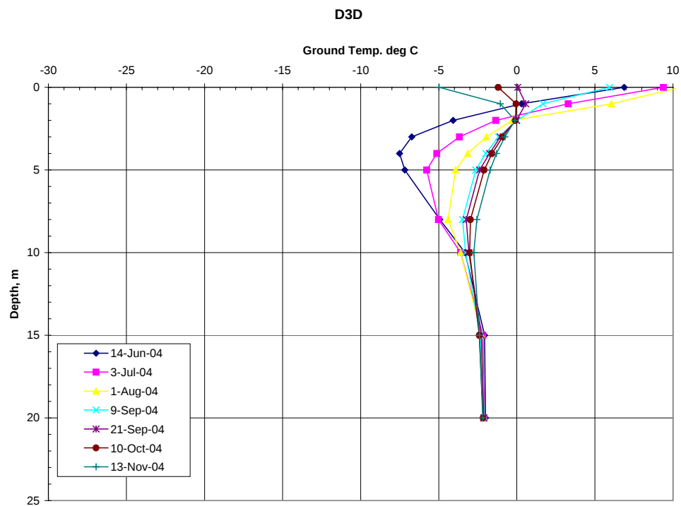
Figure C 17. Ground temperature regime at Dam 3D (Thermistor D3D -1)
