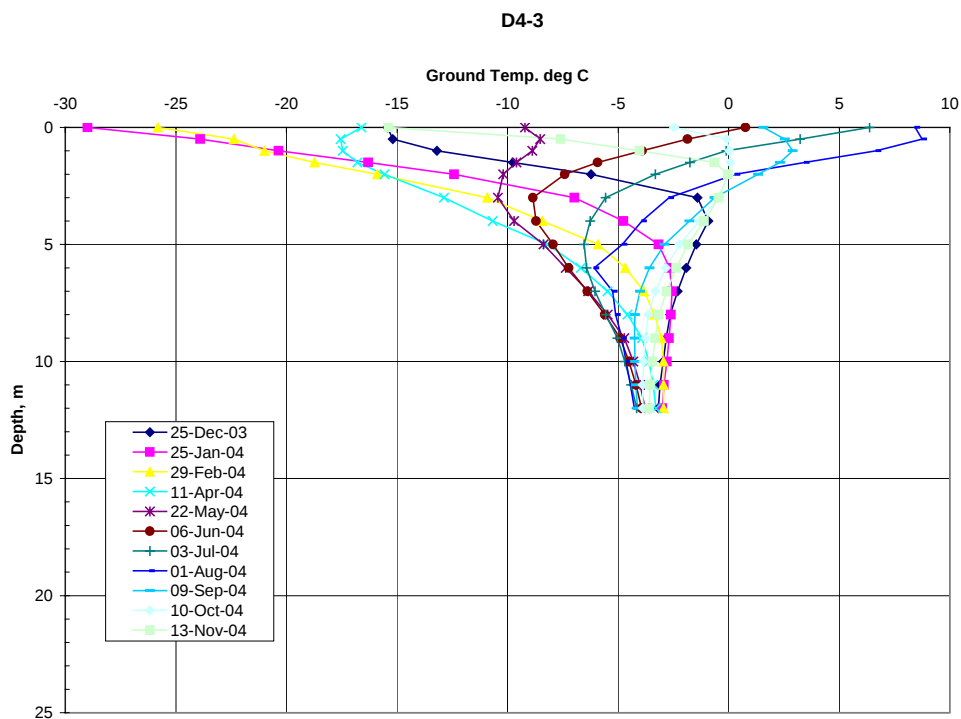
Figure C 12. Ground temperature regime at Dam 4 (Thermistor D4-3)
