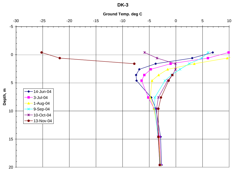
Figure C 14. Ground temperature regime at K Dam (Thermistor DK-3)
