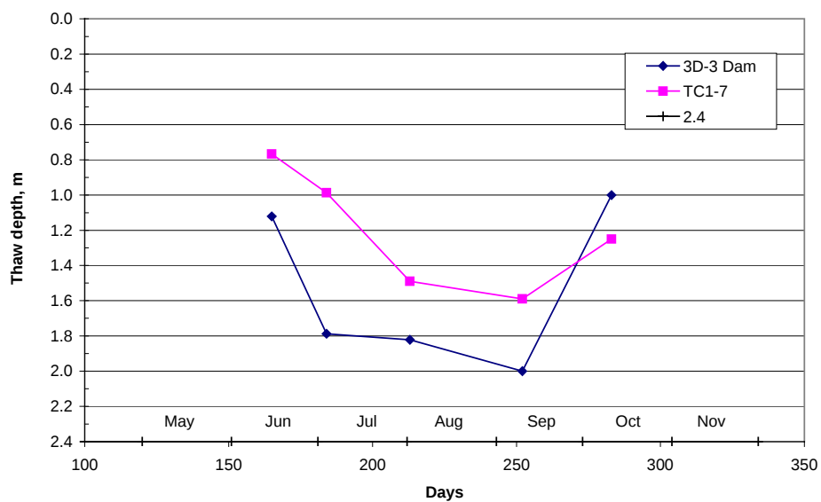
Figure C 20. Thaw surface progress with time near Dam 3D
