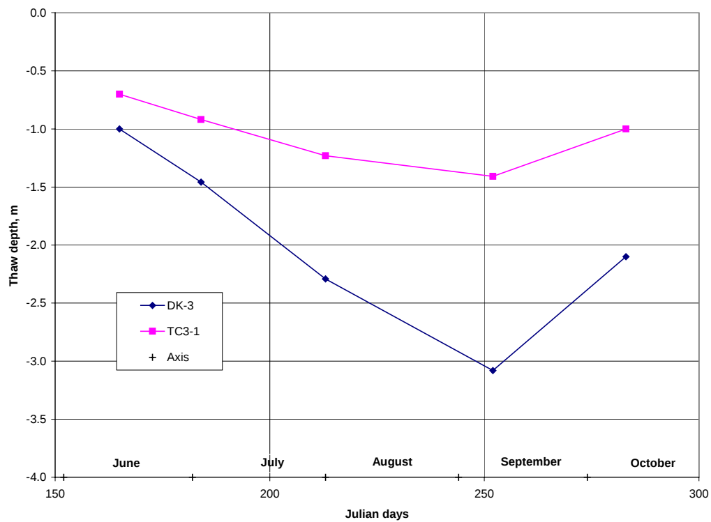
Figure C 21. Thaw depth with time at K Dam (Thermistors DK-3 and TC3-1)
