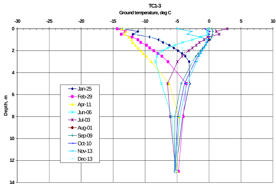
Figure C 19 Ground temperature regime at Cell 1, north end (TC1-3)
