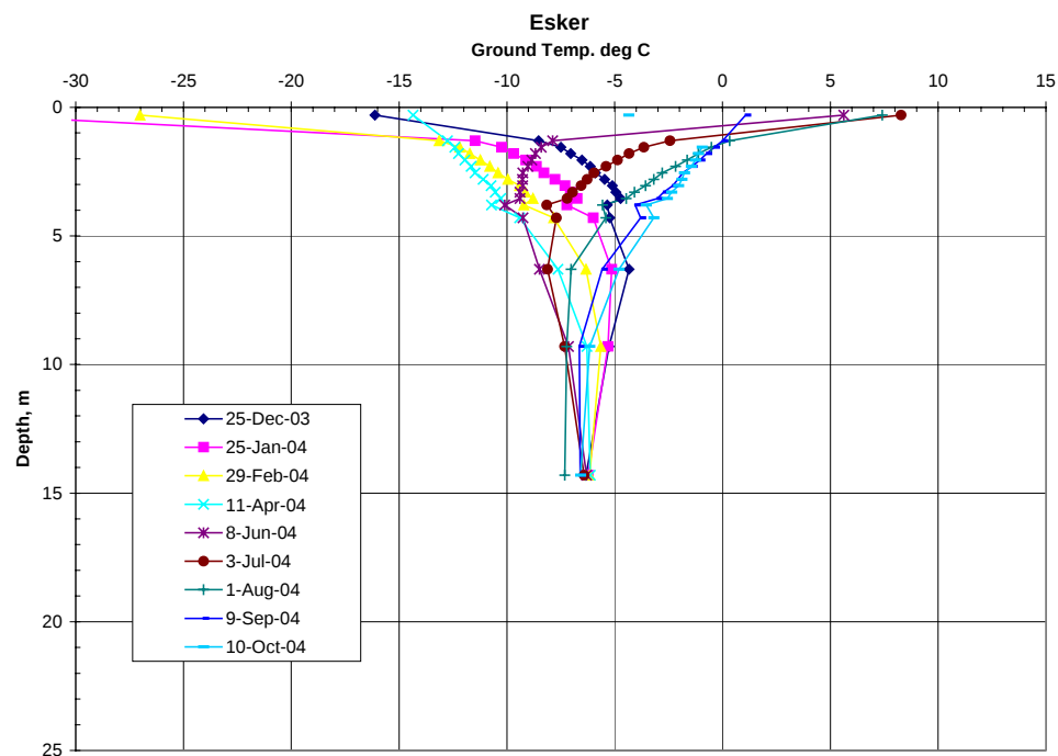
Figure C 15. Ground temperature regime at Cell 1 Test Pad (Thermistor TC1-3)
