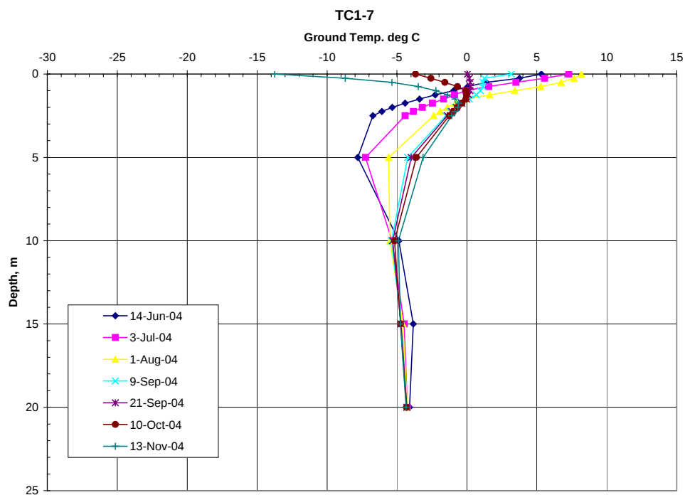
Figure C 18. Ground temperature regime in tailings Cell 1, near 3D Dam (Thermistor TC1-7)
