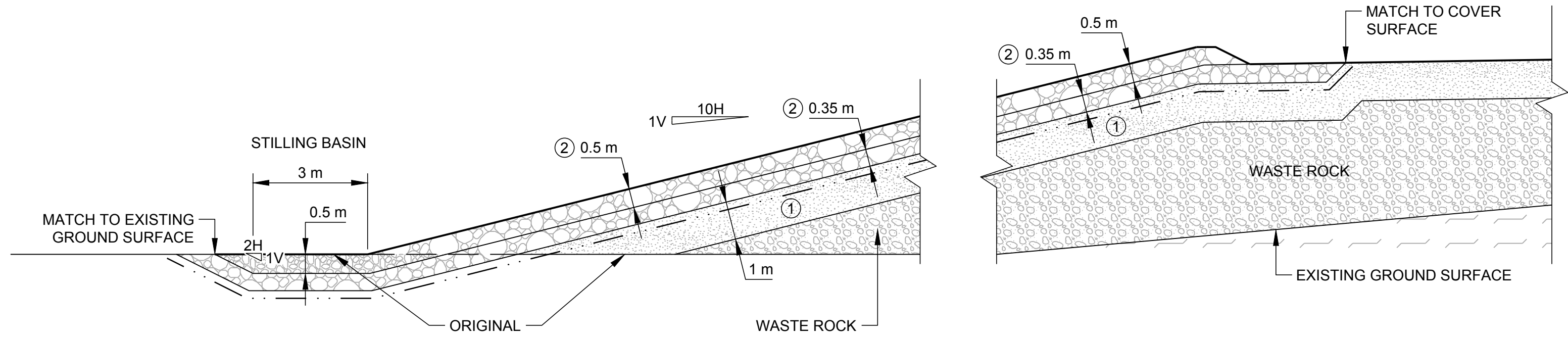
DRAINAGE CHUTE TYPICAL PROFILE N.T.S.
