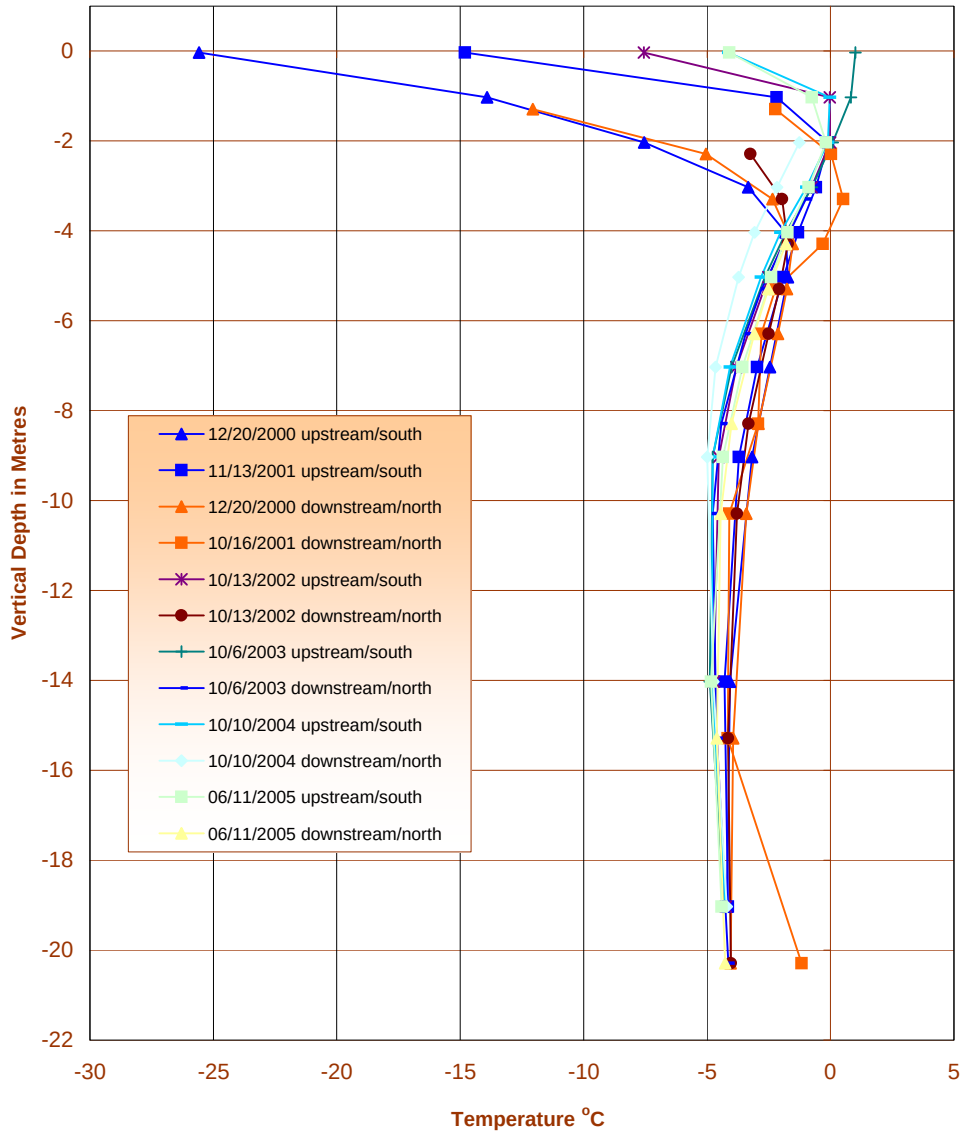
Graph 1 Dam1a Temperature Profile Thermistor D1A-00-1(south) and D1A-00-2(north)
