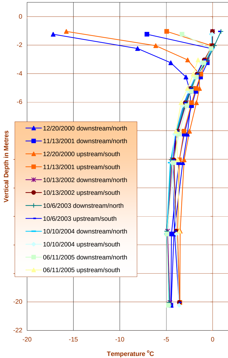
Graph 2 Dam2 Temperature Profile Thermistor D2-00-2(north) and D2-00-3(south)
