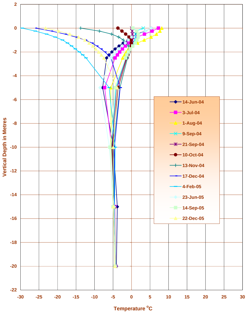
Graph 11 Cell 1 Temperature Profile Thermistor TC1-7
