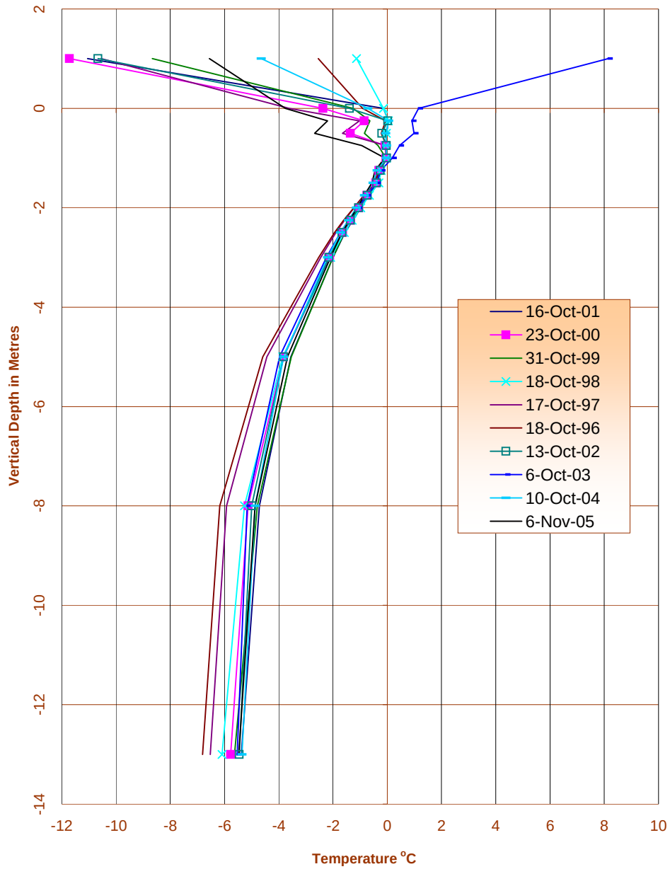
Graph 6 Cell No.1 Temperature Profile Thermistor TC1-3
