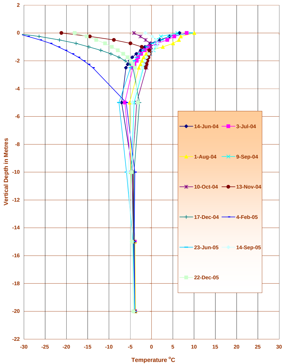
Graph 8 Cell 3 Temperature Profile Thermistor TC3-1
