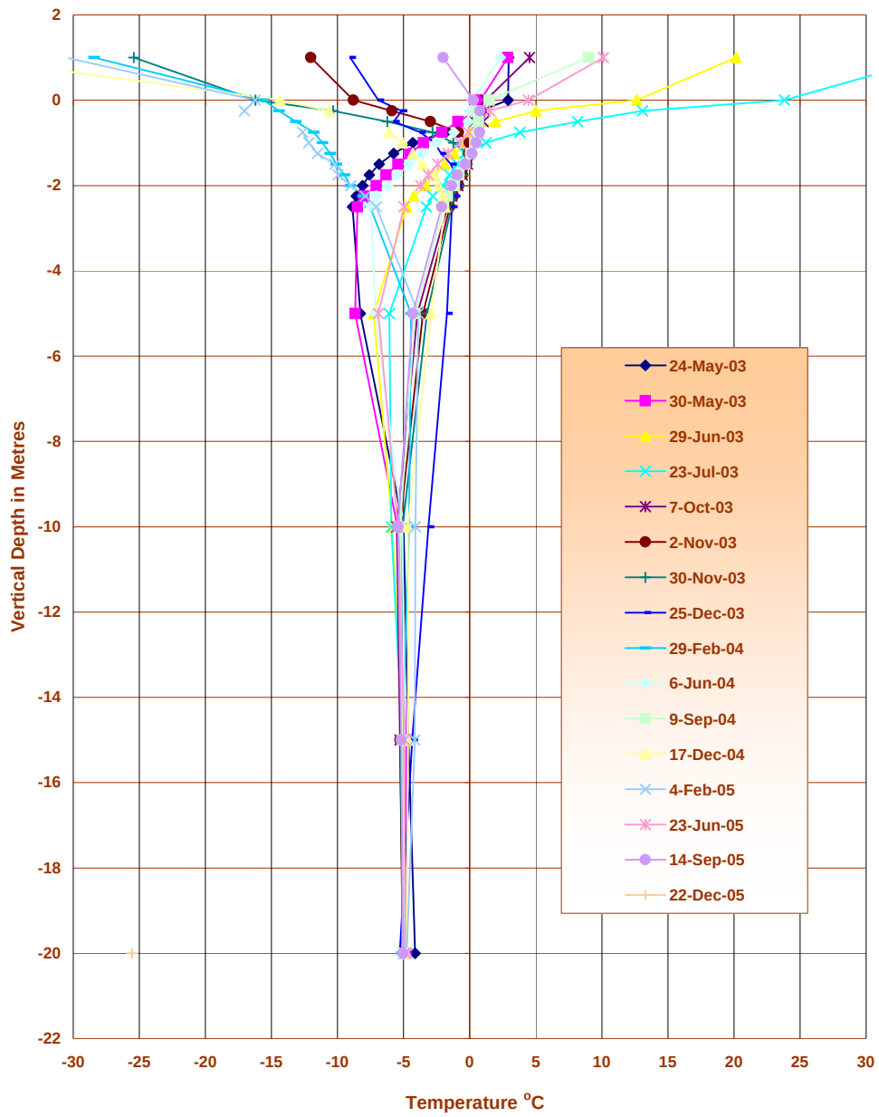
Graph 7 Cell 1 Test Pad Temperature Profile Thermistor 002-07
