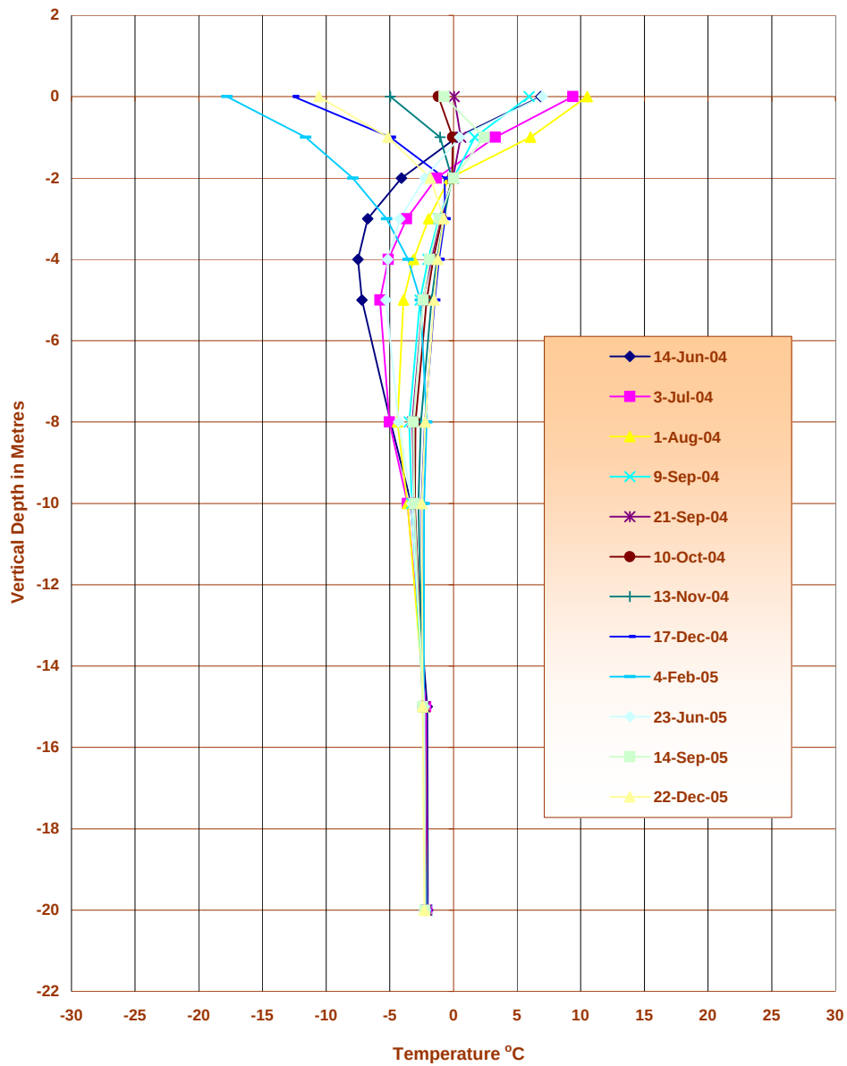
Graph 10 Dam 3D Temperature Profile Thermistor D3D-1
