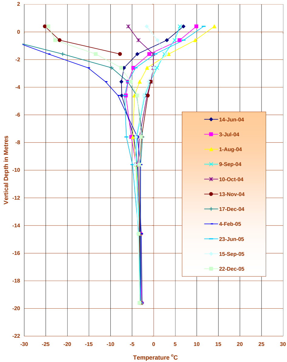
Graph 9 K Dam Temperature Profile Thermistor DK-1
