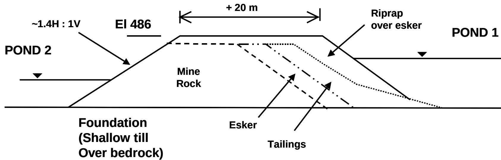
Figure B 9. J Dam section, facing north
